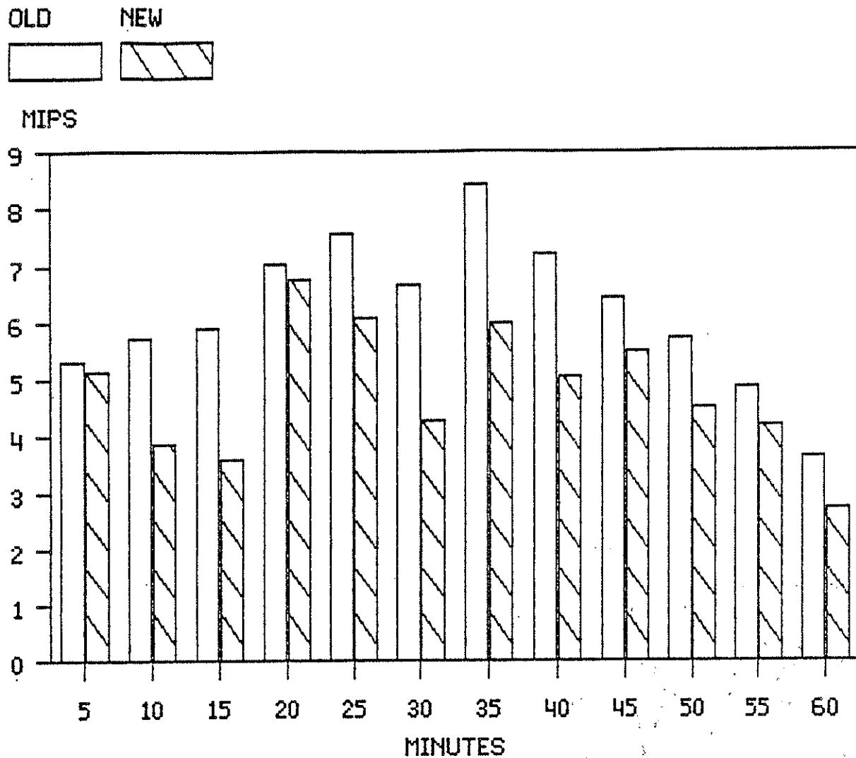
Figure 1. Estimated millions of instructions per second (MIPS) required to support meteorological and hydrological techniques in 5-min segments of a worst case hour. Both initial estimates contained in the AWIPS SRS (OLD) and estimates recently revised (NEW) are shown. The revised estimates are for only scheduled processing and explicitly exclude ad hoc requests made at workstations. The original estimates, although not addressing ad hoc requests explicitly, did purport to include all technique processing including that portion which is now considered to be non-scheduled.
