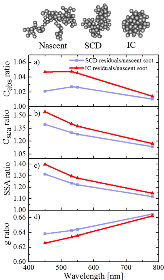
Figure 3. Images on top show the modeled soot particles used in the simulations, representing from left to right, open fractal-like nascent soot, soot residual from supercooled droplet (SCD) and ice crystal (IC). Normalized absorption (a) and scattering cross-sections (b), single scattering albedo (SSA) (c), and asymmetry parameter ( g ) (d), as functions of wavelength calculated using the discrete dipole approximation (DDA). The modeled soot particles were constructed by 100 monomers with 23 nm diameter each and different degrees of compaction to represent the measured morphological values. Optical cross-sections, SSA and g for SCD and IC soot residuals were normalized by the values obtained for nascent soot.
