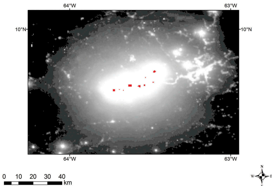
Figure 14. Glow surrounding the brightest cluster of gas flares in 2015, located near Madrid, Venezuela. The red spots indicate average radiances over 10,000 \text{ nW cm}^{-2} \text{ sr}^{-1} . These are the gas flare locations.
