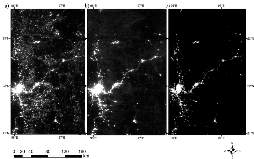
Figure 11. Three styles of VIIRS DNB average radiance grids were produced for 2015: (a) the raw cloud-free composite (RCFC), which has lights, biomass burning, and aurora present; (b) the outlier-removed cloud-free composite (ORCFC) that has been filtered to remove fires and some aurora; (c) night-time lights (VNL) with the background and all extraneous features removed except gas flaring.
