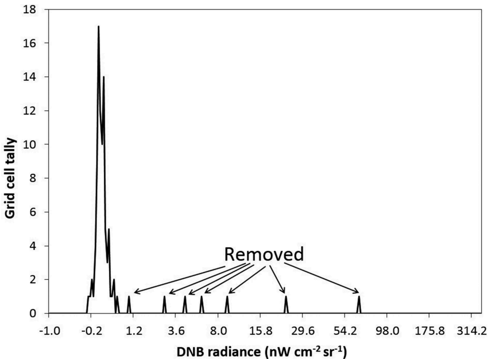
Figure 2. Outlier removal is applied to each 15 as grid cell. This histogram of 2015 data is for the grid cell at (10.43125 N, 1.31875 W) in Ghana, Africa.
