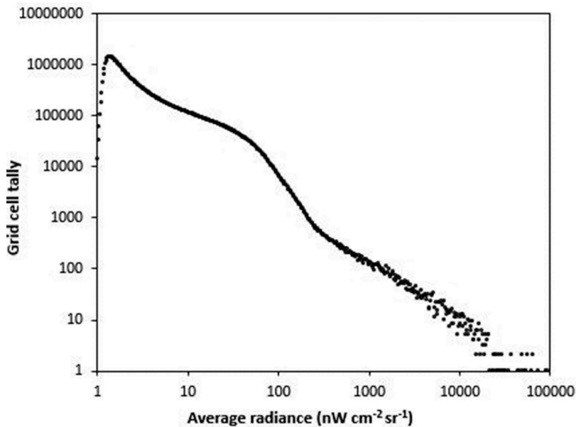
Figure 12. Histogram of the 2015 VIIRS night-time lights. There are vastly larger numbers of low radiance grid cells versus high radiance cells.
