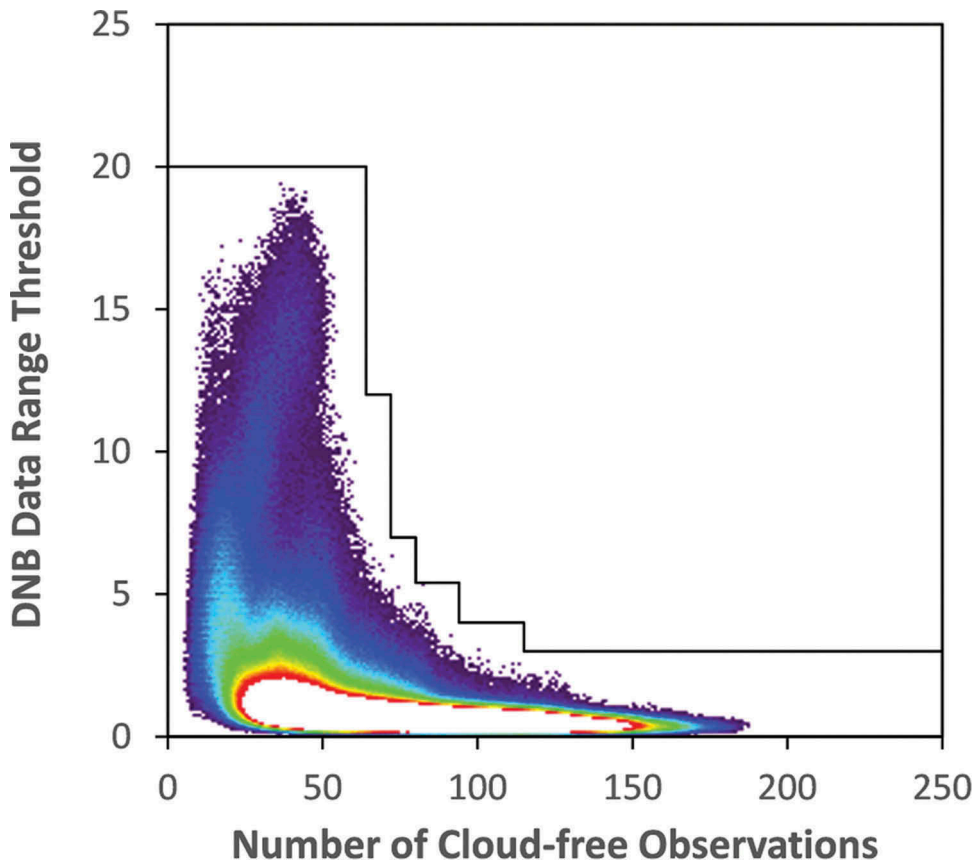
Figure 4. The threshold used to select the initial background pixel set rises as the number of cloud-free observations decreases. Thresholds are log-scaled radiance values.
