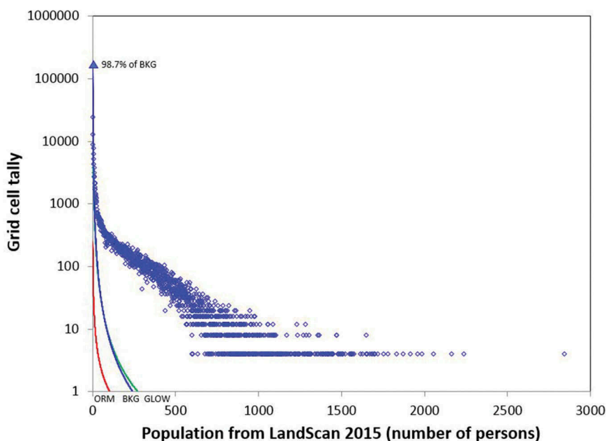
Figure 13. Comparison of Landscan population counts from four sets of grid cells in Australia. The data points are from the VIIRS night-time lights. The three trend lines show results from three varieties of background. ORM refers to grid cells where the average of high end outliers was 5 nW or more. GLOW are background grid cells where the average radiance was 0.1 nW and higher, BKG is the remainder of the background grid cells after removal of ORM and GLOW.
