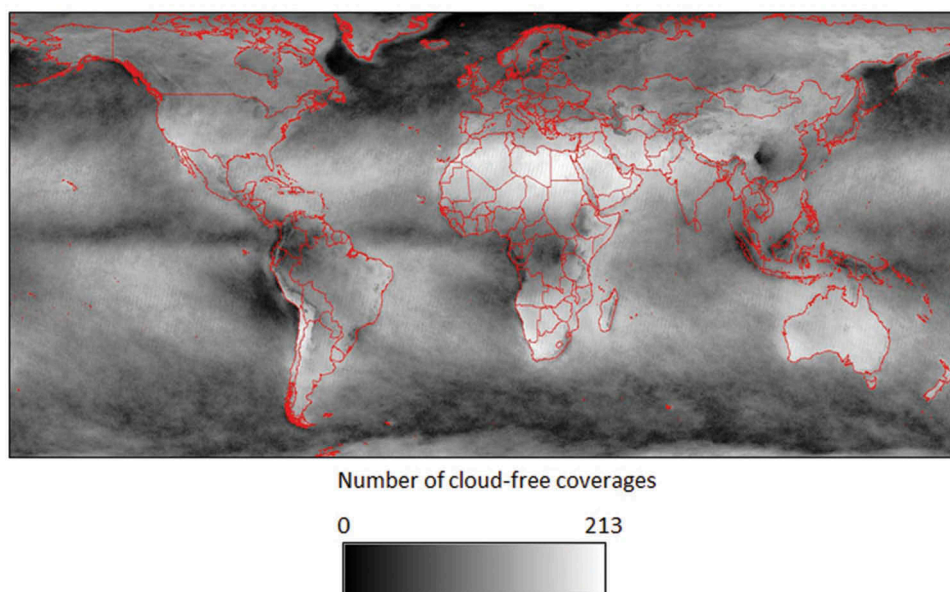
Figure 8. Grid tallying the number of cloud-free coverages (CF_CVG) for 2015. The tally includes the CVG pixels minus those pixels deemed to be cloudy by the VIIRS cloud mask.
