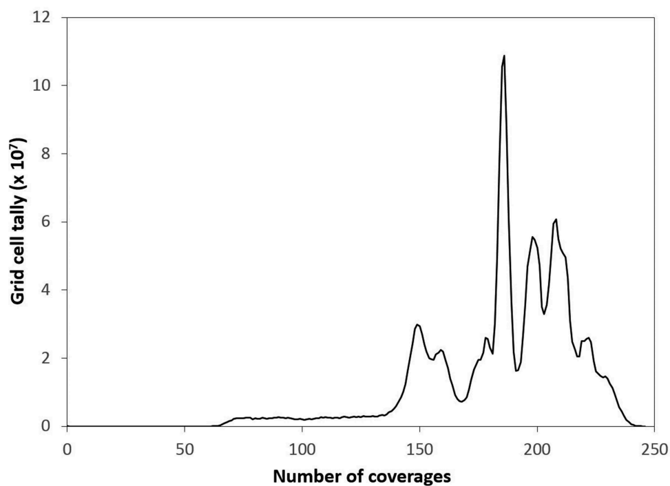
Figure 7. Histogram of coverage tallies for 2015.
