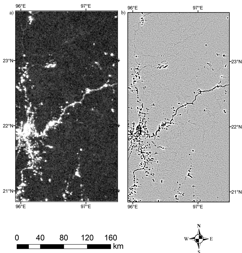
Figure 3. Two key grids used to define background pixel sets: (a) Data range calculated using a 3 \times 3 kernel. Background areas have low data ranges; (b) \lambda_1 is used to define small dim lighting features over land that are excluded from the background pixel set.
