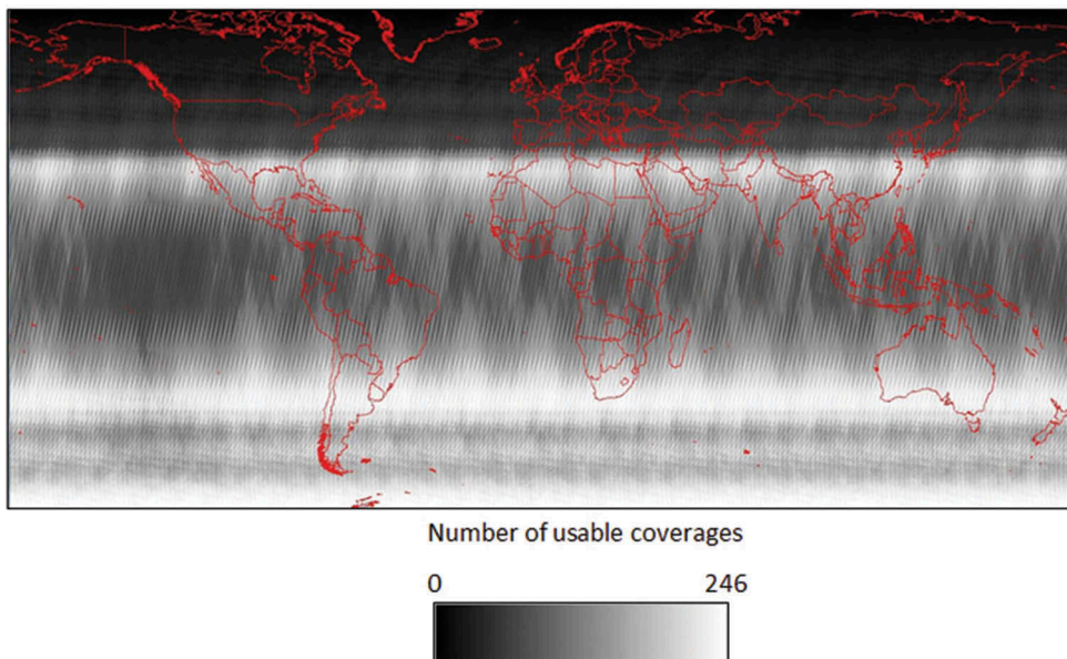
Figure 6. Grid tallying the number of usable coverages (CVG) for 2015. The tally includes pixels that passed filtering steps for sunlight, moonlight, stray light, and HEP detections.
