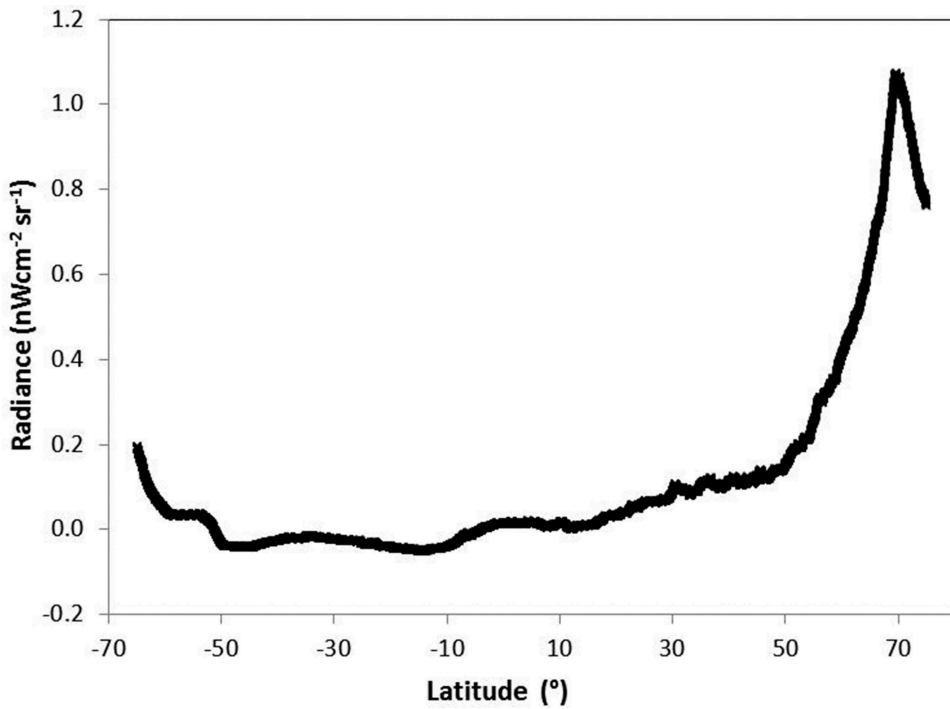
Figure 10. Average background radiance as a function of latitude for 2015.
