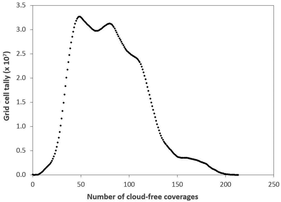
Figure 9. Histogram of the cloud-free coverages for 2015.
