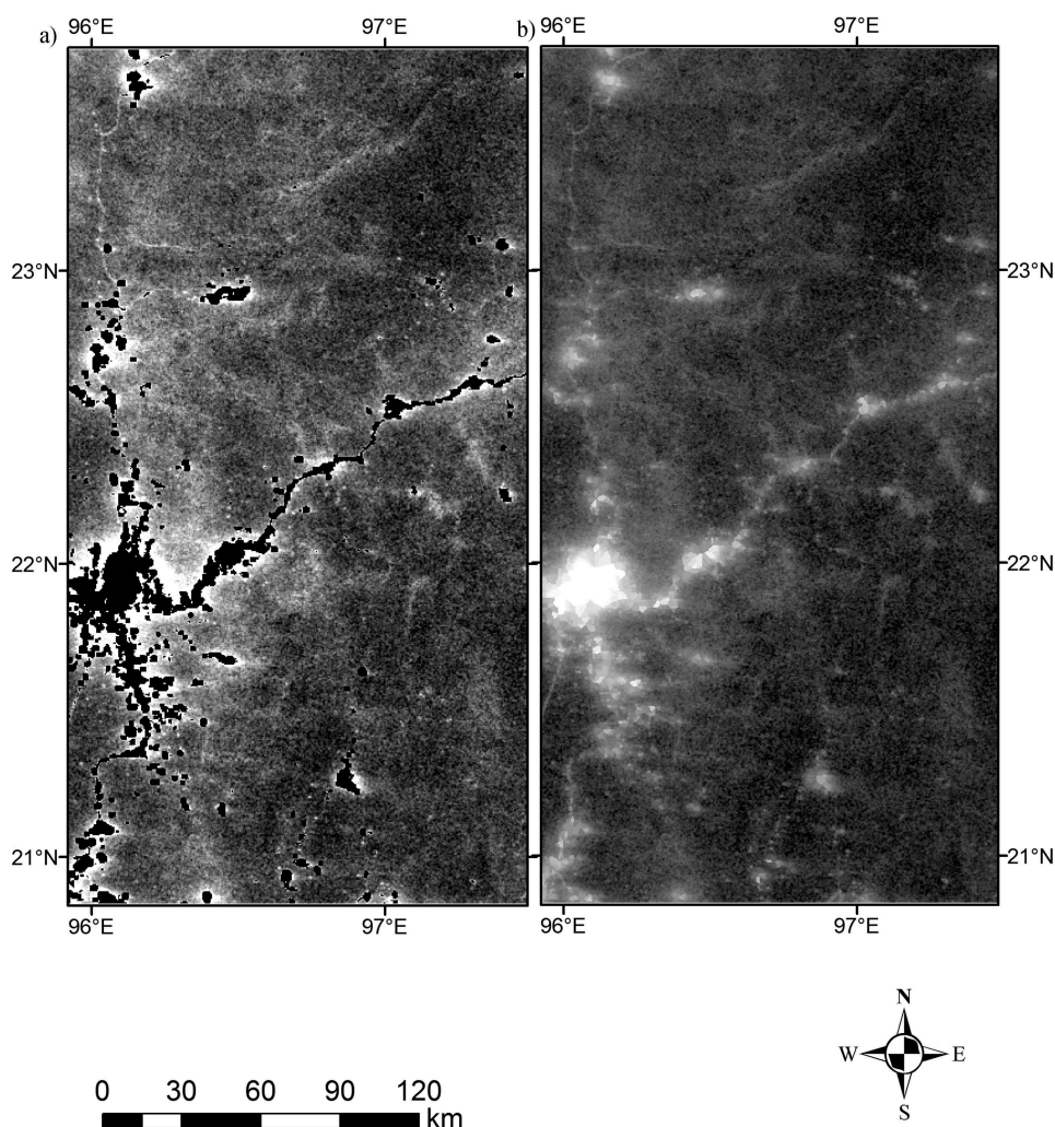
Figure 5. The final steps in defining the background: (a) After defining the seeds background pixel set, the average radiances are restored from the outlier-removed cloud-free composite, leaving zeros in the areas with data ranges that are above the selection threshold or \lambda_{a1} values over land less than -0.55 ; (b) the holes are filled using the radiance from the nearest background pixel. Note that the effects of glow surrounding bright lights can be seen in both the seeds grid and the background grid. The seeds grid contains part of the glow adjacent to bright lighting. The glow pixels are subsequently propagated to fill the holes in the background grid.
