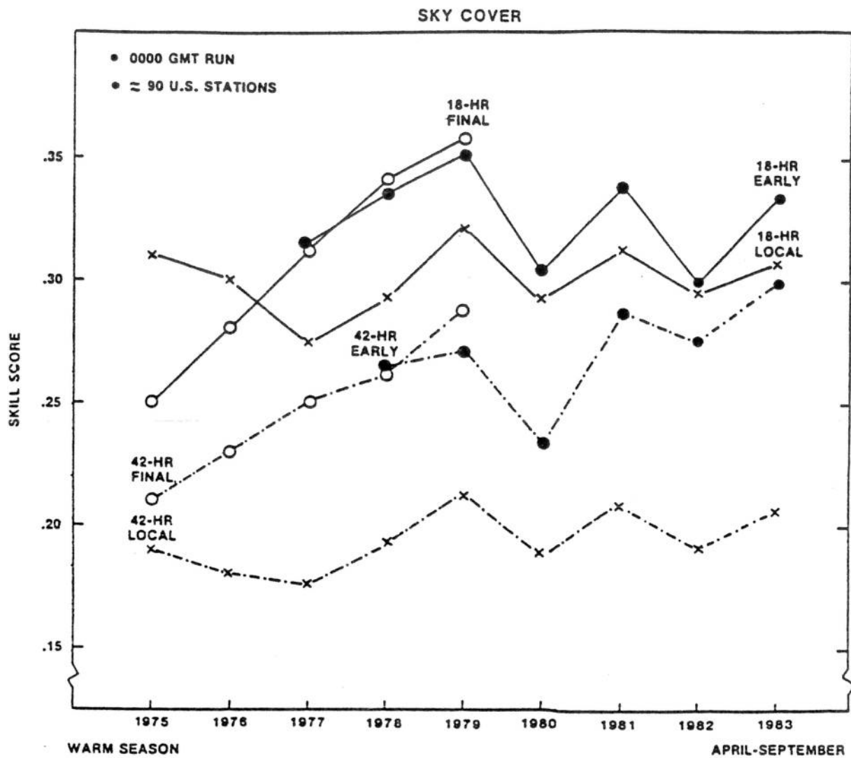
Figure 4.2. Same as Fig. 4.1 except for skill score.
