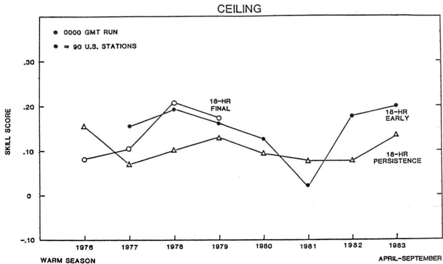
Figure 5.2. Same as Fig. 5.1 except for forecast projection.
