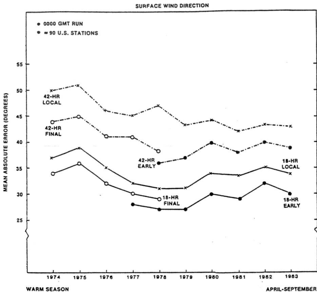
Figure 3.1. Mean absolute error for the local and the early and final guidance surface wind direction forecasts. Only 71 stations were available for 1983.
