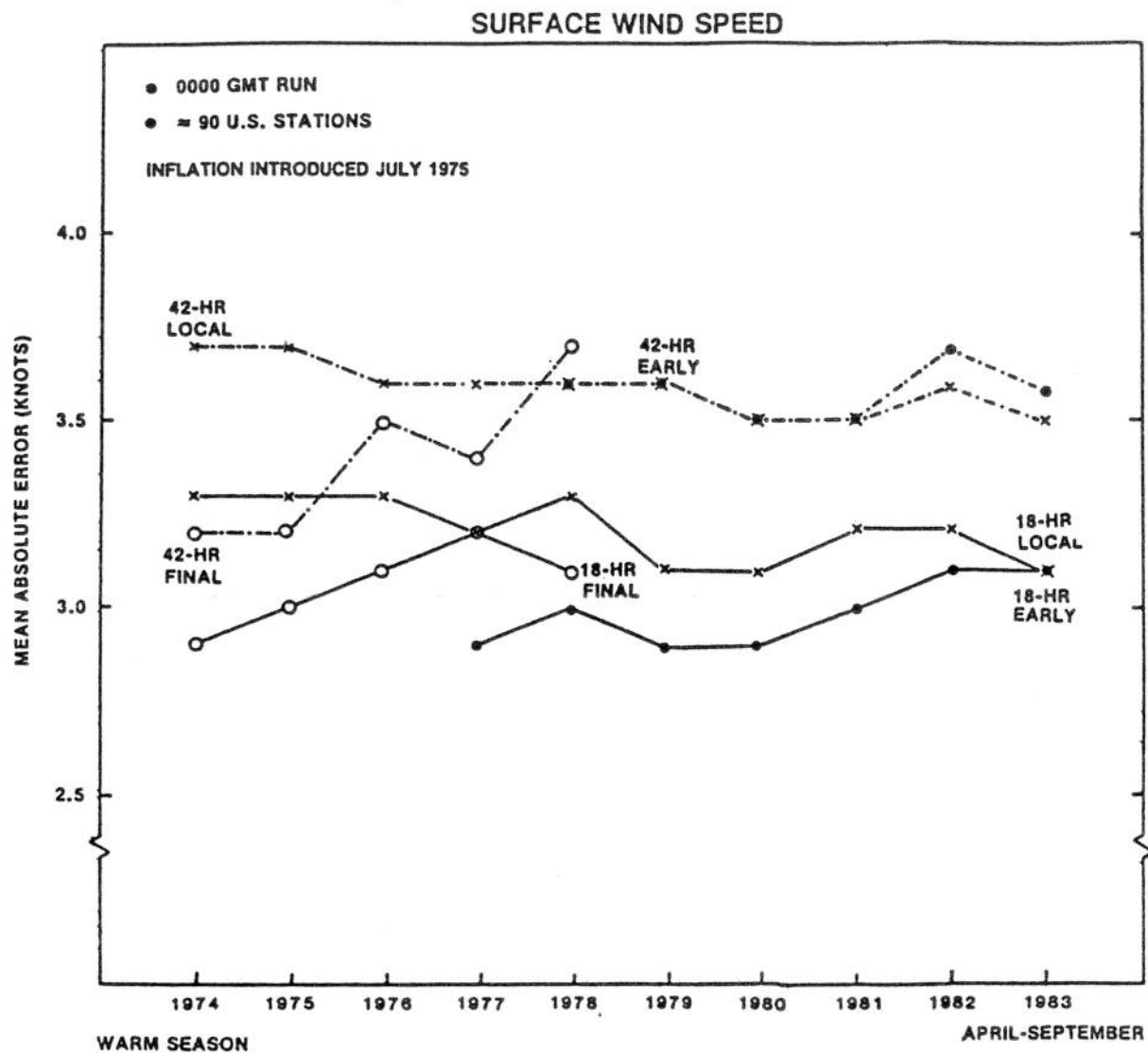
Figure 3.2. Same as Fig. 3.1 except for surface wind speed.
