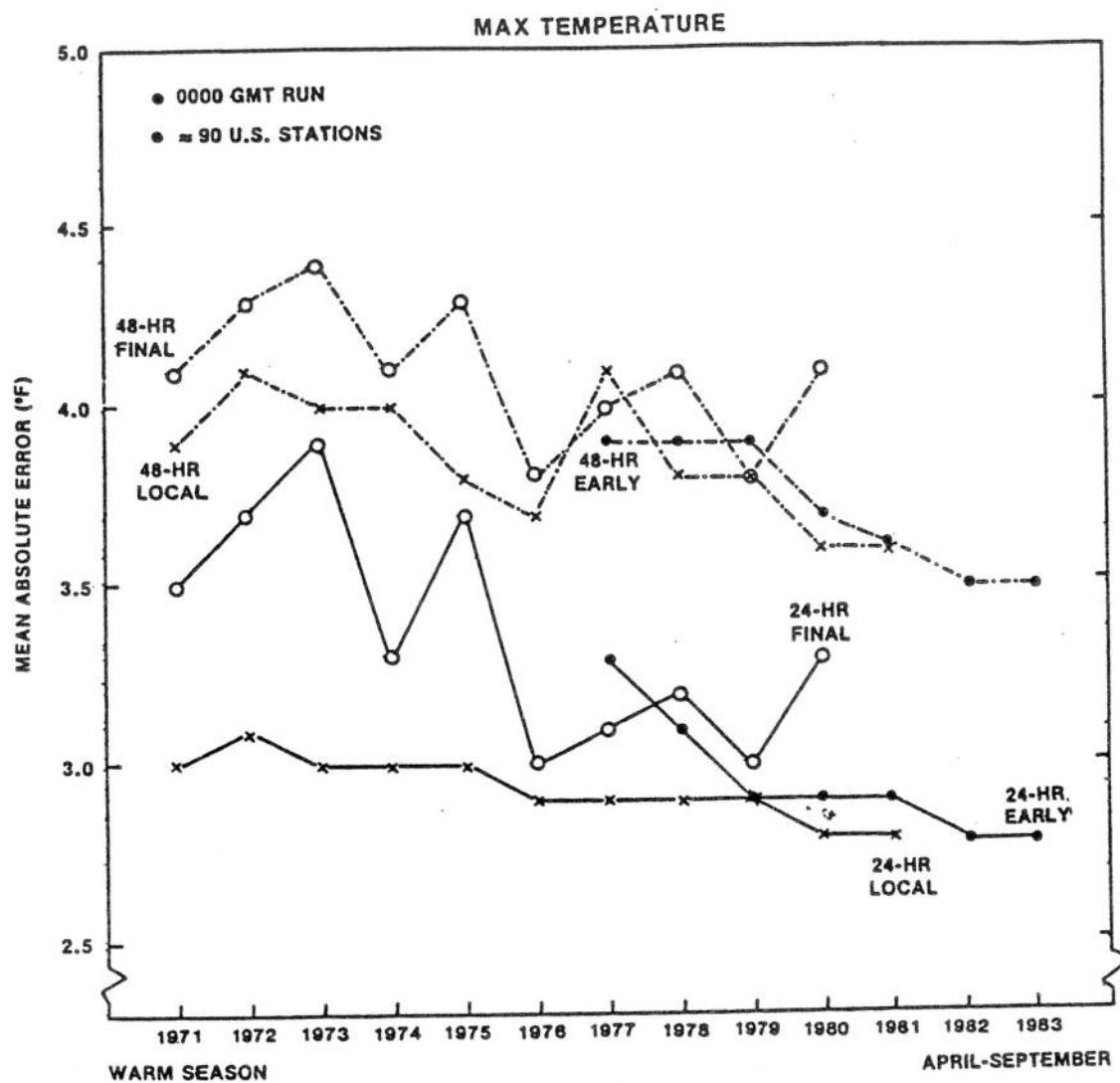
Figure 6.1. Mean absolute error for the local and the early and final guidance max temperature forecasts.
