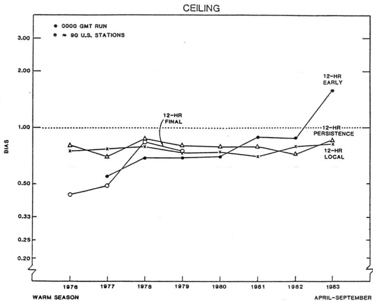
Figure 5.5. Bias for categories 1 and 2 combined for persistence, local, and guidance (early and final) ceiling height forecasts. Only 71 stations were available for 1983.
