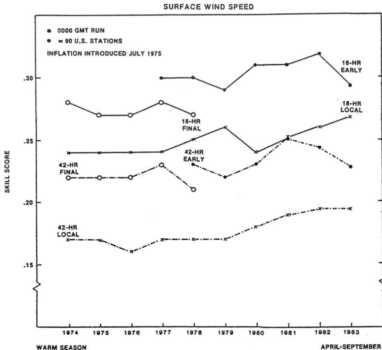
Figure 3.3. Skill score computed from five-category contingency tables for the local and the early and final guidance surface wind speed forecasts.
