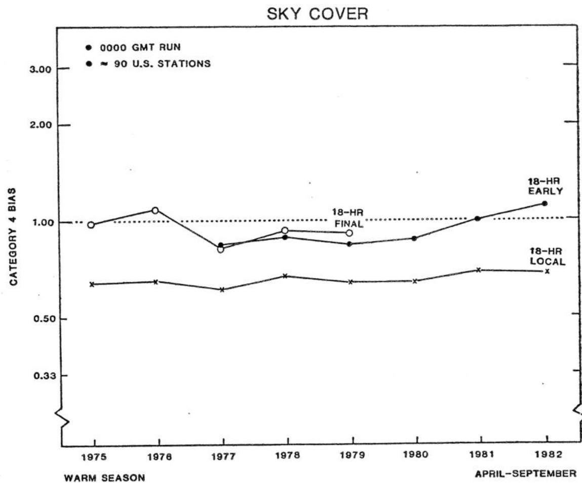
Figure 4.6. Same as Fig. 4.3 except for category 4 bias.
