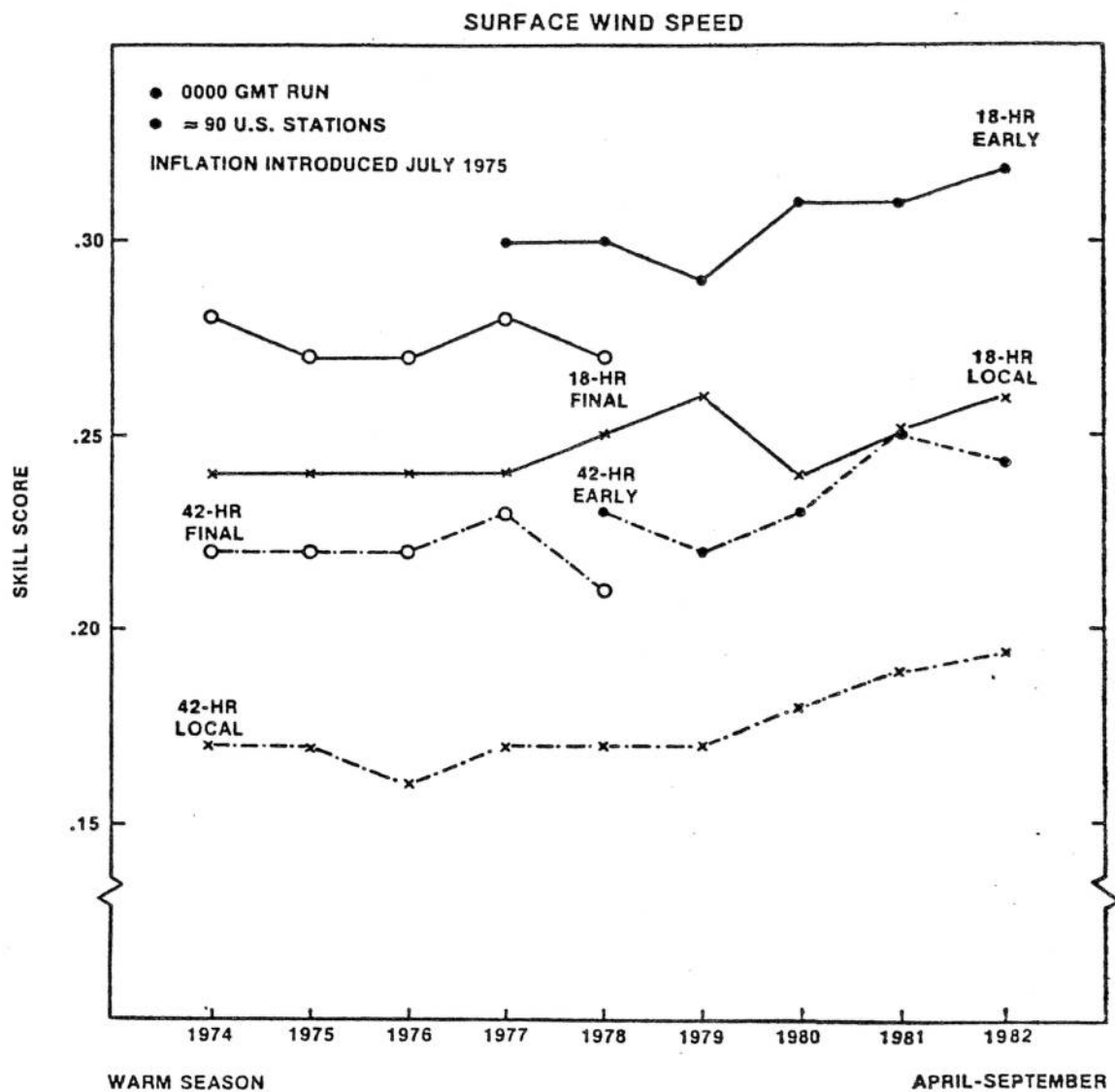
Figure 3.3. Skill score computed from five-category contingency tables for the local and the early and final guidance surface wind speed forecasts.
