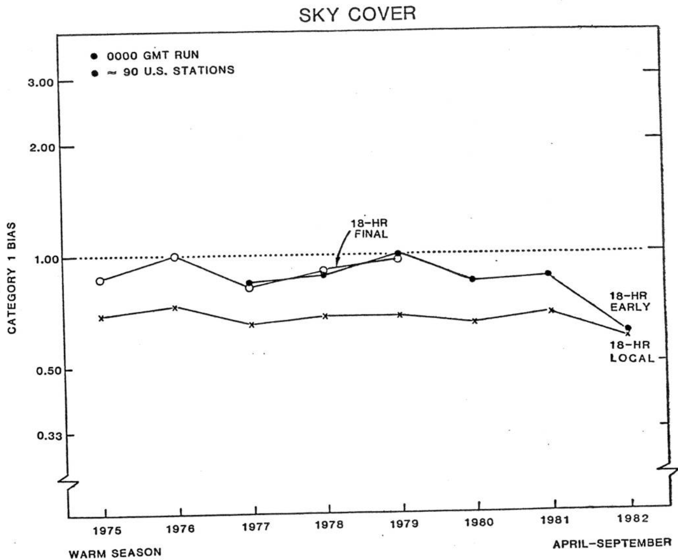
Figure 4.3. Category 1 bias for the local and the early and final guidance opaque sky cover forecasts.
