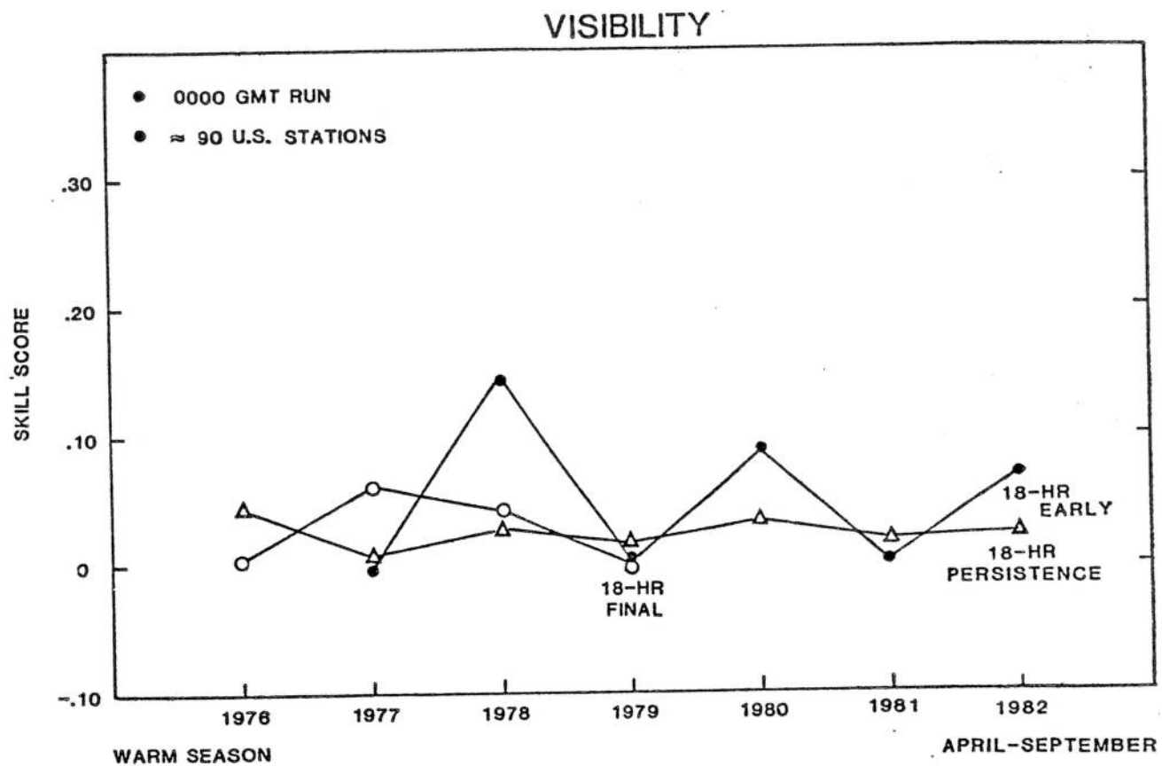
Figure 5.4. Same as Fig. 5.1 except for visibility and forecast projection.
