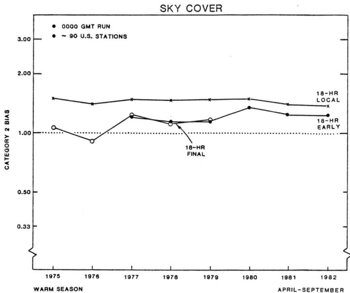
Figure 4.4. Same as Fig. 4.3 except for category 2 bias.
