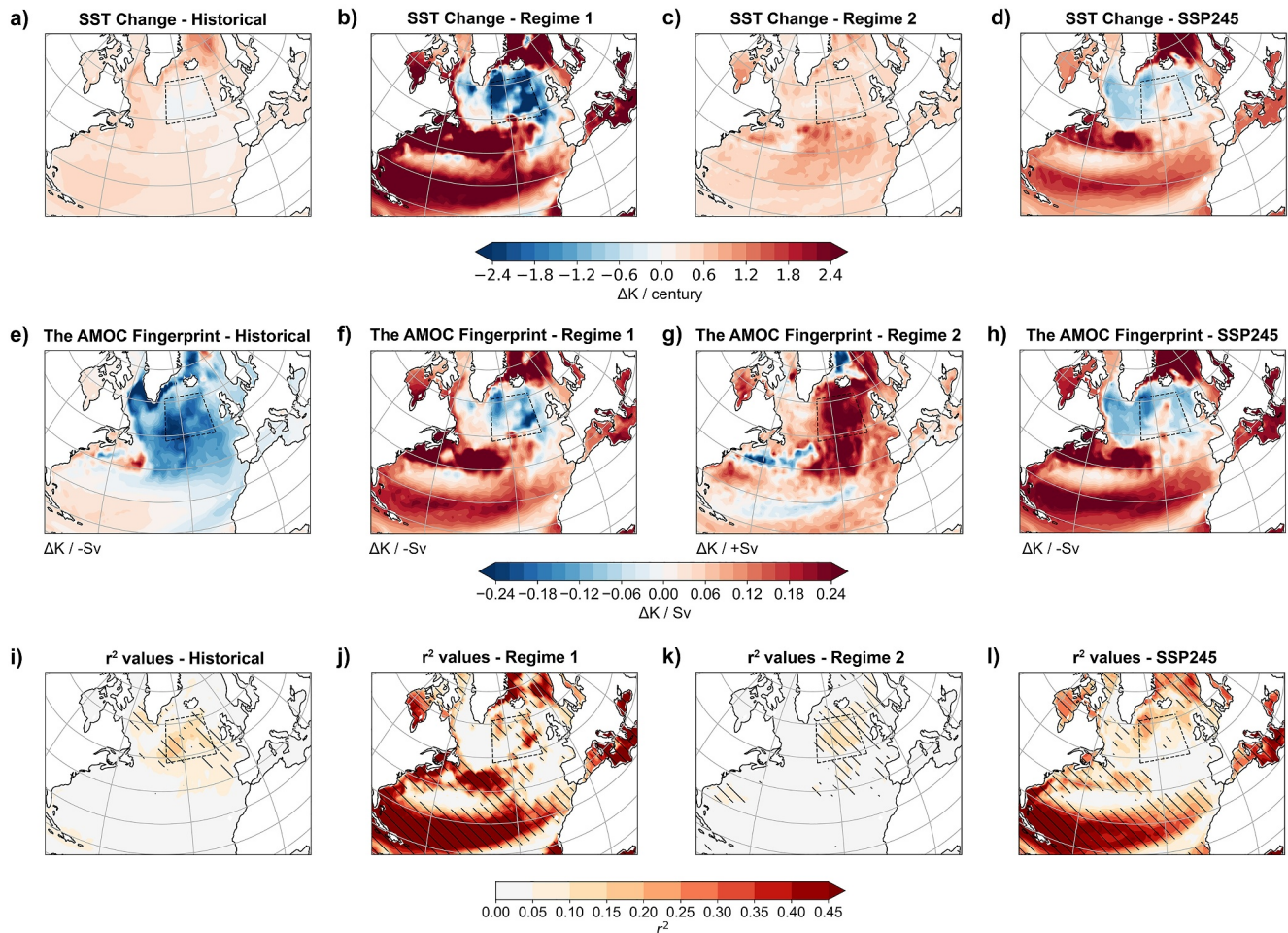
Figure 3. The SST trend (unit: K/century) over the subpolar North Atlantic as derived from the (a) Historical Simulation; (b) the decline period (Regime 1) of Abrupt 4\times\text{CO}_2 ; (c) the stabilized period (Regime 2) of Abrupt 4\times\text{CO}_2 ; and (d) the moderate pathway SSP245. (e–h) are the SST-based AMOC fingerprints calculated as a regression between AMOC-index and SST, with a lag of 0 years, showing the potential SST change per 1 Sv change in AMOC. Sub-figure (g) is shown in \Delta K / +\text{Sv} , as the overall SST pattern is warming in the NAWH during the scenario. (i–l) are the r^2 values, with hatches to signify a p < 0.05 . The dashed boxes outline the spatial extent of the subpolar North Atlantic warming hole in the MPI-ESM1.2-HR model.
