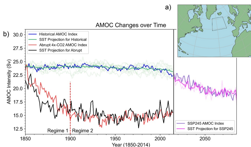
Figure 1. (a) A map demarking the location of the North Atlantic Warming Hole (NAWH). (b) Time series of AMOC intensity in Historical, Abrupt 4\times\text{CO}_2 and SSP245 scenarios. The Abrupt scenario is split into two distinct regimes, one characterized by a quick and constant decline, and the other by a stabilized “shutdown”. The historical simulation is averaged along 10 realizations, while SSP245 is averaged over 2. The WH-index and AMOC-index were regressed to project AMOC based on the WH-index.
