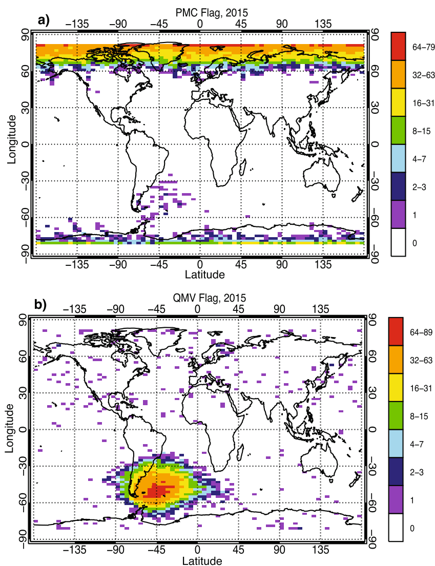
Figure 4. Spatial distribution of the PMC (a) and QMV (b) flags in 2015. The data are shown for 5^\circ by 2^\circ spatial bins (longitude \times latitudes) and expressed as the total number of profiles illuminated by the PMC (a) or QMV (b) flag in 2015. Increased flagging occurs south of the geographic location of the SAA because the tangent points are 3,000 km distant from the satellite itself.
