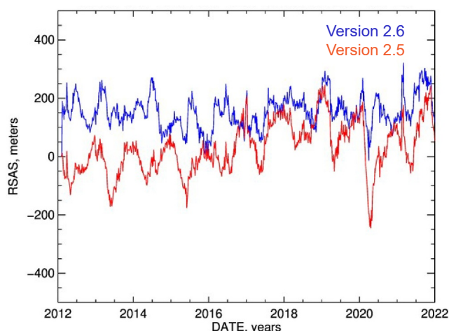
Figure 1. RSAS (Rayleigh Scattering Attitude Sensing) time series for versions 2.5 (red) and 2.6 (blue) from April 2012 through December 2021 in the Southern Hemisphere ( 50^{\circ}\text{S} – 20^{\circ}\text{S} ). The results are illustrated as errors in the instrument pointing expressed in meters. The RSAS method is sensitive to aerosol interference, therefore we limited the region to the southern mid-latitudes where the LP measurement sensitivity to aerosol as well as aerosol contamination are minimum. The Hunga eruption in January 2022 injected large amounts of aerosol into the stratosphere and as a result substantially affected the RSAS record (see Section 2.2.5 and Figure S9 in Supporting Information S1).
