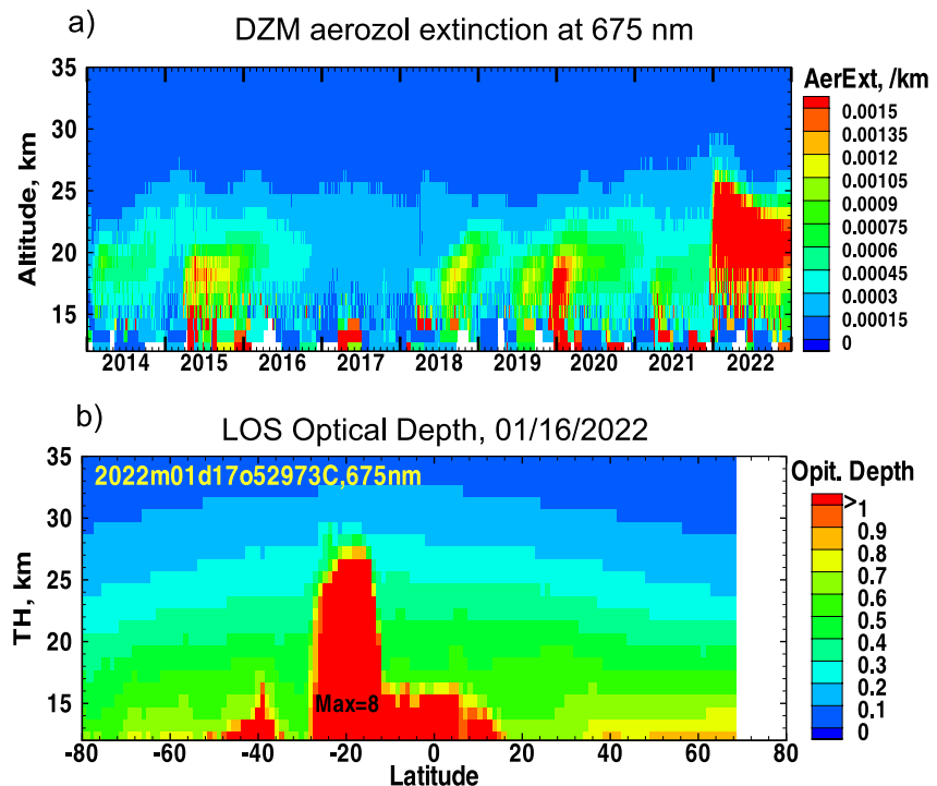
Figure 7. Upper panel shows daily zonal mean values of aerosol extinction in SH subtropics ( 15^{\circ} – 20^{\circ} S) over the SNPP mission. Typical background aerosol extinction is <10^{-3} \text{ km}^{-1} , particularly above 15 km, but extinction increases after volcanic eruptions (e.g., Calbuco eruption in 2015) or mega wildfires (2019–2020 New Year Australian fires). The Hunga eruption injected aerosol to an unprecedented height and increased zonally averaged aerosol extinction in the stratosphere to levels >1.5 \times 10^{-3} \text{ km}^{-1} . Lower panel shows LOS optical depth at 675 nm for one orbit (52,958) on 16 January 2022. The LOS optical depth was well above 1 in the region near the eruption (with the maximum estimated LOS depth \sim 8 ). Ozone retrievals are not possible in conditions when the LOS optical depth exceeds 1.
