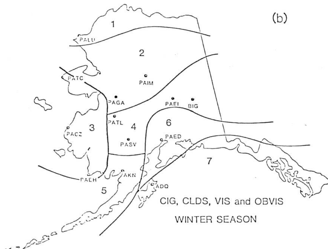
Figure 3. Alaskan military stations with regions used to develop probability of ceiling height (CIG), cloud amount (CLD), visibility (VIS, and obstructions to vision (OBSVIS) equations for the fall (a), winter (b), spring (c), and summer (d).
