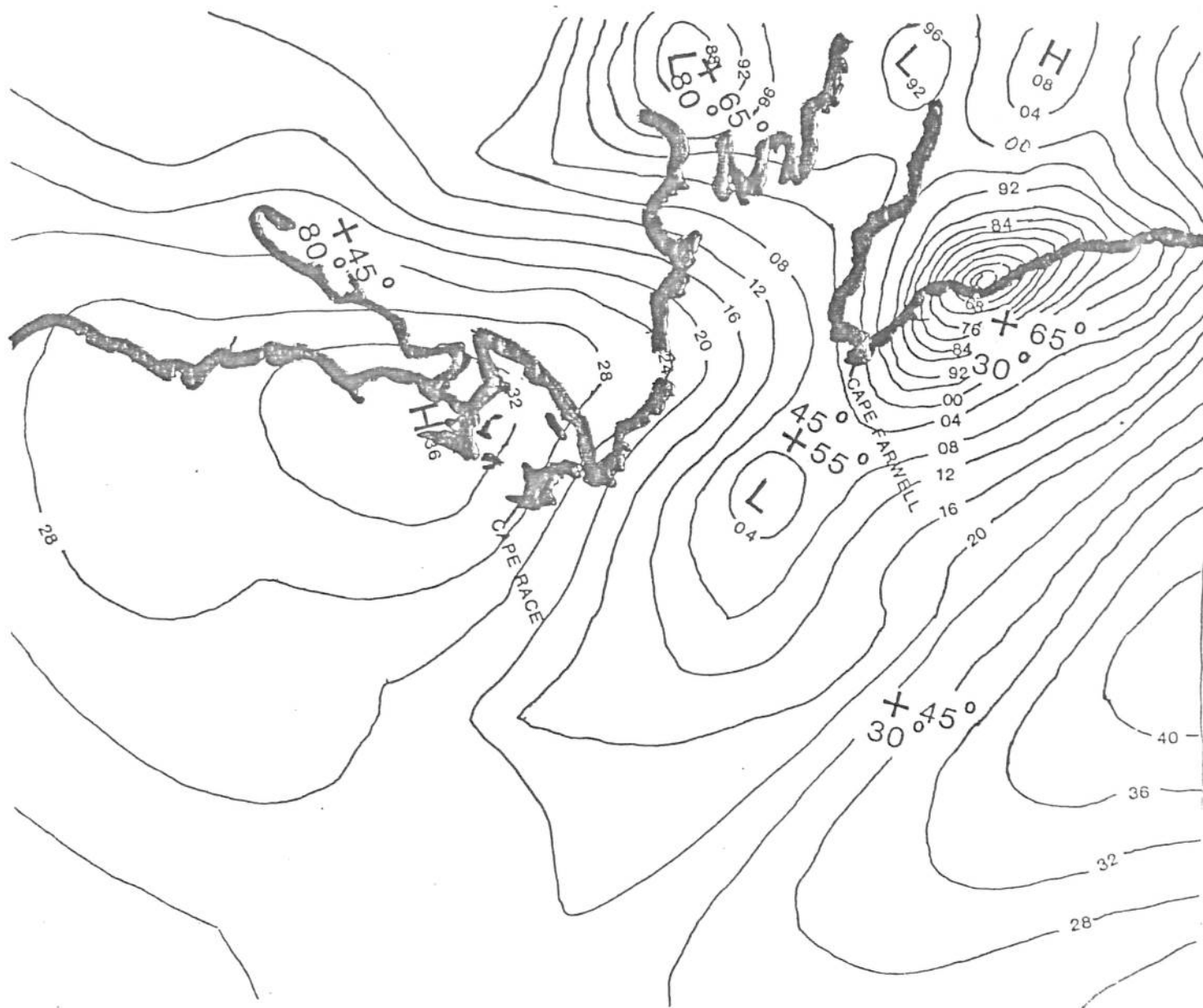
Figure 5. Sea level pressure analysis valid 1200 GMT February 10, 1984.
