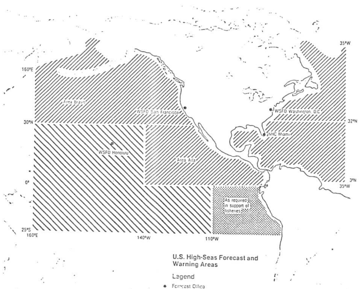
Figure 1. High seas forecast and warning areas for the United States (from National Weather Service, 1981).
