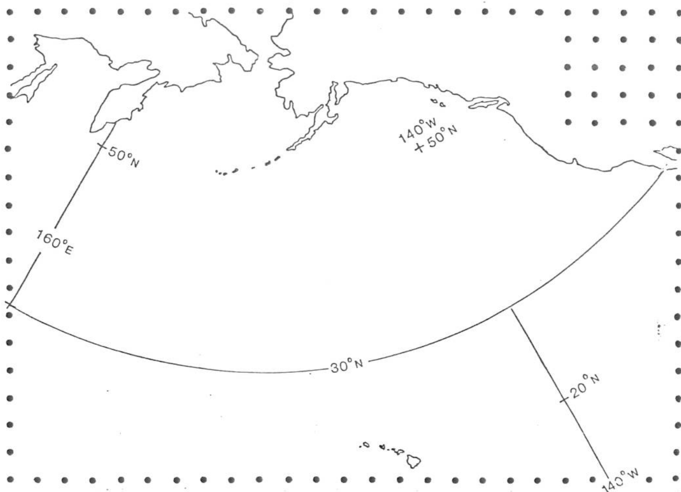
Figure 3. Same as Fig. 2 except for the Pacific Ocean.
