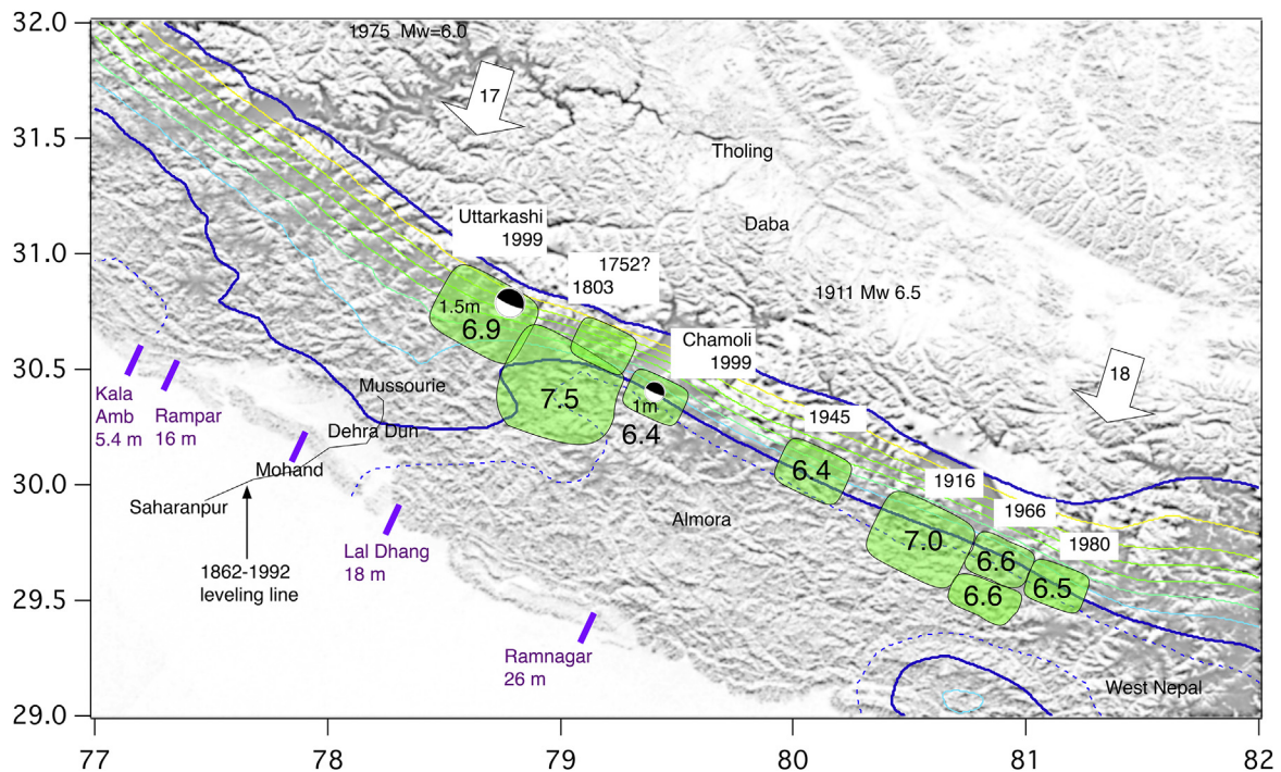
Fig. 11. Moderate Himalayan earthquakes since 1752 between longitudes 77^\circ\text{E} and 82^\circ\text{E} . Bold blue contours envelope the interseismic decoupling zone between 0.9 and zero coupling, dashed line = 1.0 i.e. locked (Stevens and Avouac, 2015). The 1752 and 1803 rupture zones shown are conjectural (the 1752 earthquake may have occurred close to Daba). Rupture zones for other earthquakes are scaled in proportion to magnitude. Paleoseismic trenches (violet bars) with maximum slip indicated from Kumar et al. (2006; 2010). An 8.6 < M_w < 8.8 earthquake is inferred to have ruptured the entire décollement 6 June 1505 (Ambraseys and Jackson, 2003).
