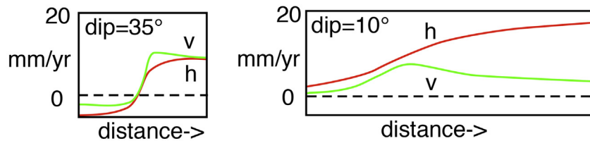
b. dip vs. width, w
