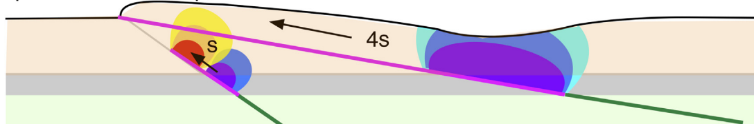
Fig. 2. Cartoon illustrating the influence of dip on (a) surface velocity fields, (b) the width of the interseismic decoupling zone, (c) the consequent increased volume ( V ) and capacity for this zone to store strain energy, u_\epsilon at shallow dip ( E = Young's Modulus; \epsilon = strain), and (d) coseismic slip. The increased slip in (d) arises because a fourfold increase in time must elapse for Himalayan convergence in (c) to attain the critical strain to nucleate rupture. Thus although the strain at failure ( \epsilon_c ) is the same, the slip deficit is four times greater. The grey zone in each case is the temperature-depth range within which partial interseismic decoupling occurs from 1 = fully locked, to 0 = fully creeping. Red/yellow = interseismic contraction; Blue/violet = coseismic extension; complimentary strains in the Indian plate are omitted. In the example shown (d), the shallow dipping fault has sufficient slip-potential to rupture to the surface whereas the steeply dipping fault incompletely ruptures the décollement.
