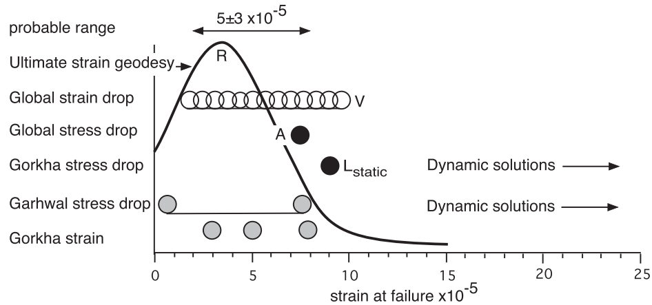
Fig. 3. Strain at failure from different methods. R = Gaussian fit to geodetic strain at failure for \approx 50 earthquakes (Rikitate, 1976, 1982). V = Vallée, (2013), A = Allmann and Shearer (2009), L_{static} = Lay et al., 2016. See text for additional sources used in the figure.
