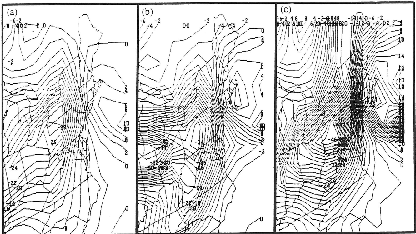
Figure 6. Temperature advection ( ^{\circ}\text{C}/12 \text{ hr} ) at (a) 850 mb, (b) 700 mb, and (c) 500 mb.
