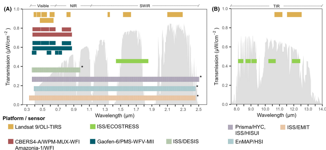
Figure 4. Spectral bands captured by spaceborne sensors in the (A) visible, near-infrared (NIR), shortwave-infrared (SWIR) and (B) thermal-infrared (TIR) regions of the spectra. *Figure scale constrained the complete visualization of the narrow spectral bands of hyperspectral systems. Number of bands ( n ) for the hyperspectral platform/instrument are: ISS/DESIS ( n = 235 ), Prisma/HYC ( n = 240 ), ISS/HISUI ( n = 185 ), EnMAP/HSI ( n = 242 ). 1 \mu\text{m} = 1000 \text{ nm} .
