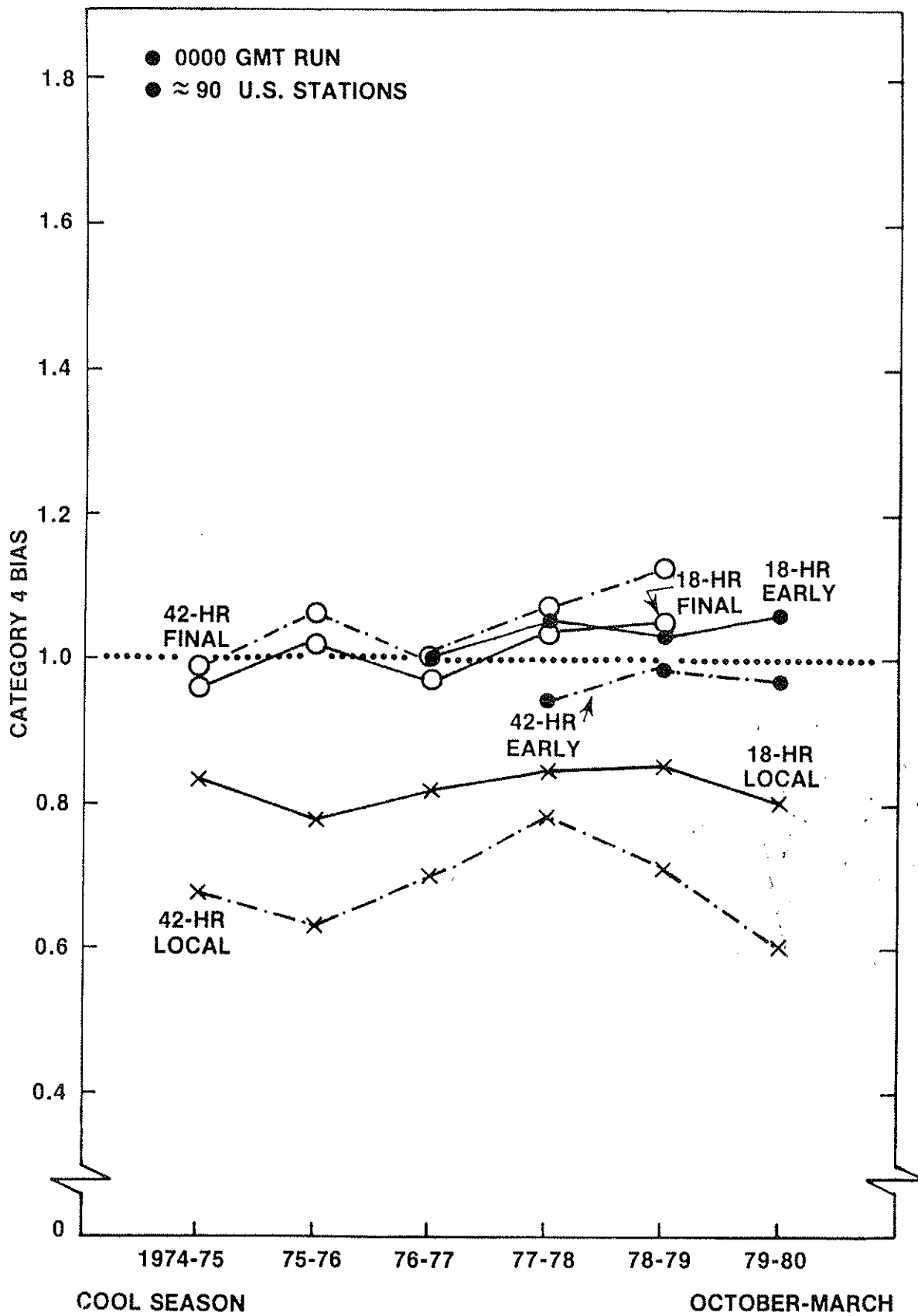
Fig. 5.6. Same as Fig. 5.3 except for category 4 bias.
