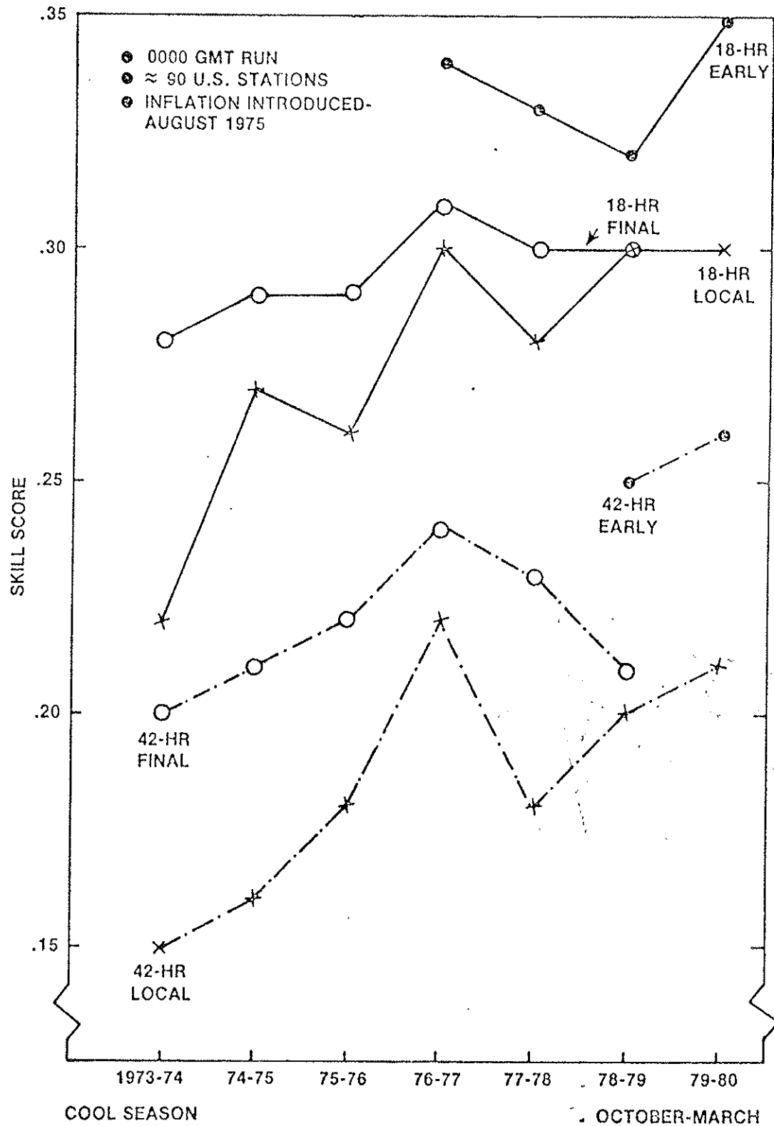
Fig. 4.3. Skill scores computed from five category contingency tables for local and guidance surface wind speed forecasts for the cool season.
