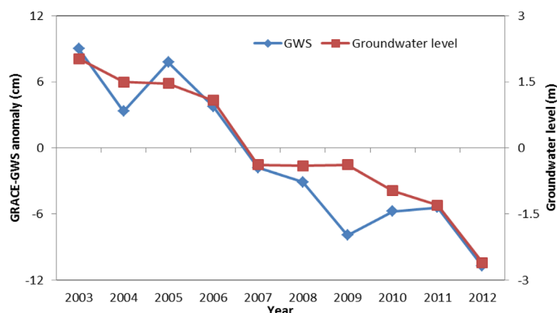
Figure 6. Comparison of the GRACE-derived GWS anomalies and in situ groundwater level anomalies averaged from about 250 observation wells in Punjab (i.e., the highest overdraft state) during the water years 2003–2012.
