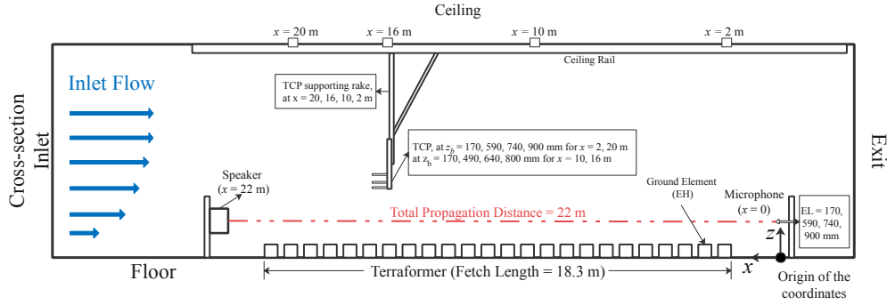
Figure 4: Experimental schematic from the UFBLWT acoustic propagation tests [28].
