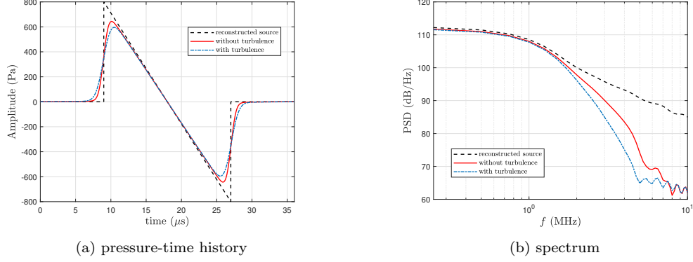
Figure 13: Comparison with the experimental results of Lipkens and Blackstock [34]
