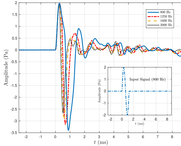
Figure 3: Output single cycle signals at 2 m from speaker. [27]
