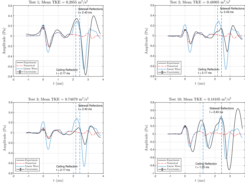
Figure 5: Comparison between predictions and wind tunnel measurements.
