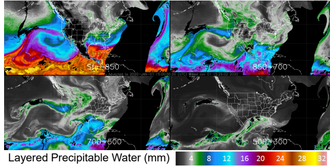
Figure 5: The Advection Layered Precipitable Water Product (ALPW) visualizes water moisture in the atmosphere at four different levels. Water moisture is measured in millimeters (mm) of precipitable water and ranges from 0 mm to 32 mm. Traditionally, each layer is shown separately in different windows.
