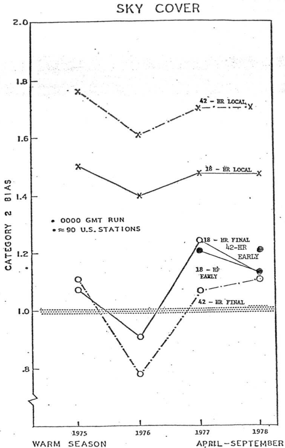
Figure 4.4. Same as Fig. 4.3 except for category 2 bias.
