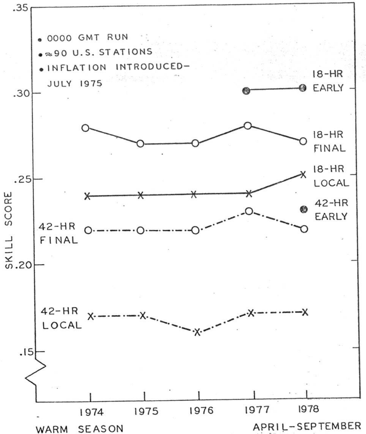
Figure 3.3. Skill scores computed from five-category contingency tables for subjective local and objective (early and final) surface wind speed forecasts for approximately 90 U.S. stations.
