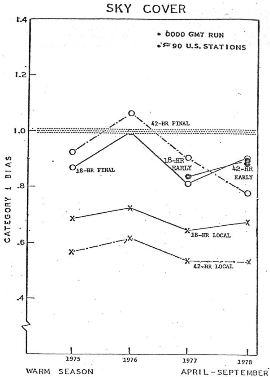
Figure 4.3. Bias of the local and guidance cloud amount forecasts of category 1 for the warm season.
