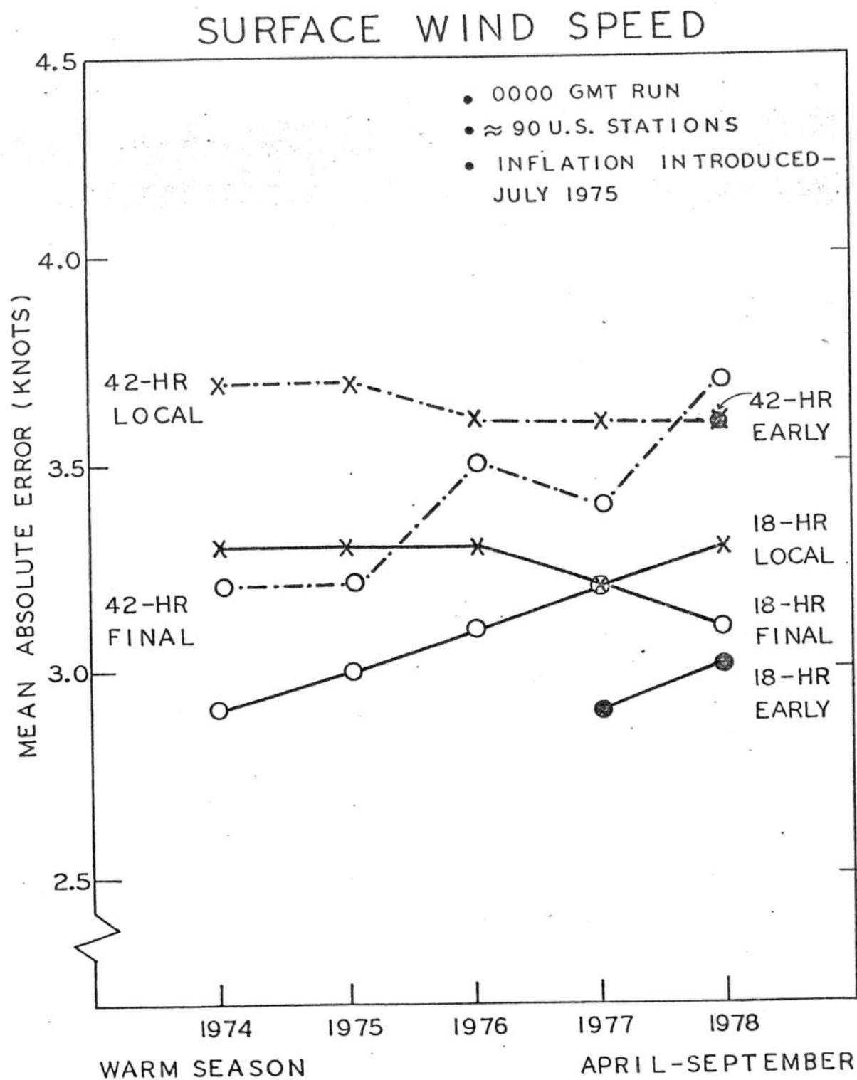
Figure 3.2. Same as Fig. 3.1 except for wind speed forecasts.
