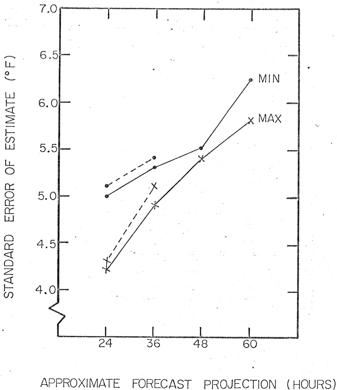
Figure 2. Standard errors of estimate ( ^{\circ}\text{F} ) for the cool season early guidance max (X) and min ( \bullet ) forecast equations. Values for the first projection are an average of those for the fall and winter seasons. The dashed lines indicate standard errors for the backup equations which do not use surface observations as predictors.
