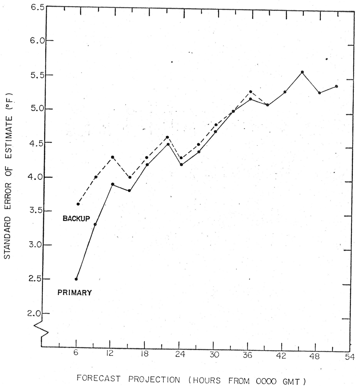
Figure 3-a. Standard errors of estimate ( ^{\circ}\text{F} ) for the cool season 0000 GMT 3-hourly temperature forecast equations. The values for the 6-through 27-h projections are averages of the fall and winter season errors. The dashed lines indicate standard errors for the backup equations which do not use surface observations as predictors.
