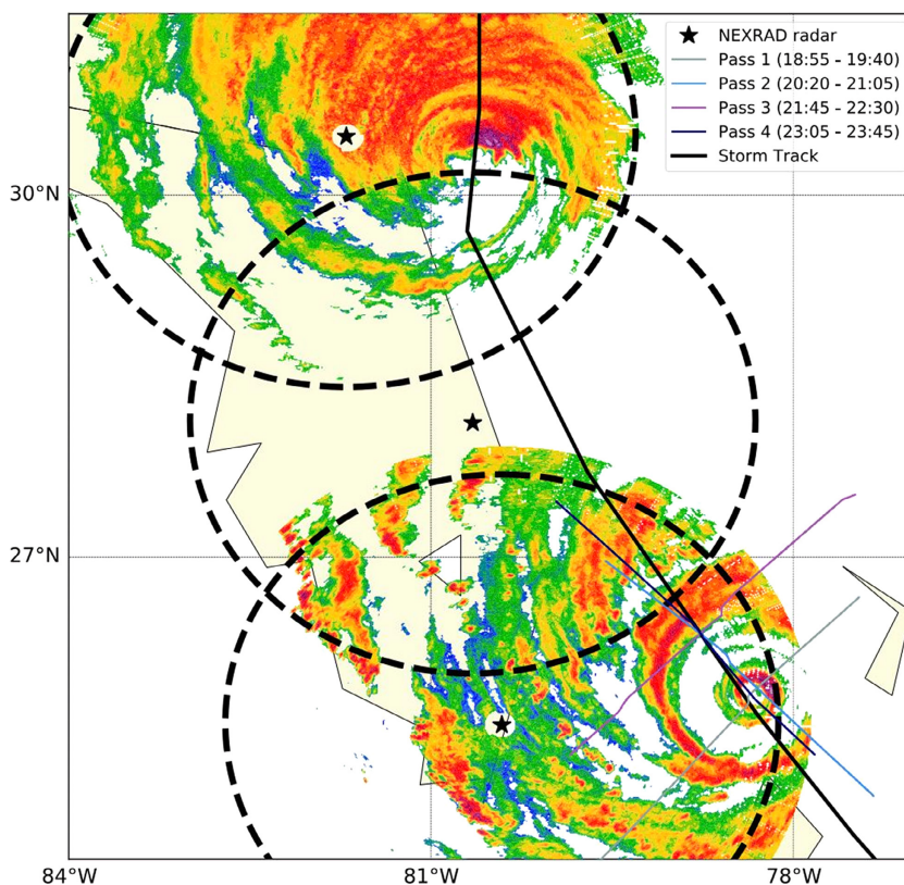
Fig. 8. Hurricane Matthew's track (solid line) and reflectivity at z = 4 km at 1930 UTC 6 October and 2126 7 October, respectively. Figure 1 of Cha et al. (2021). © American Meteorological Society. Used with permission.
