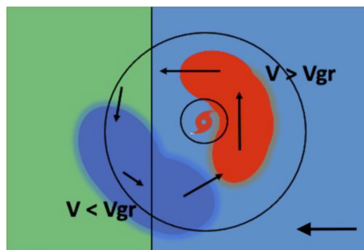
Fig. 5. A schematic illustration of the flow around a landfalling TC. The subgradient winds with large inflow angles are indicated in blue, while the supergradient winds at the top of the boundary layer are indicated in red. Figure 23 of Hlywiak and Nolan (2022). © American Meteorological Society. Used with permission.
