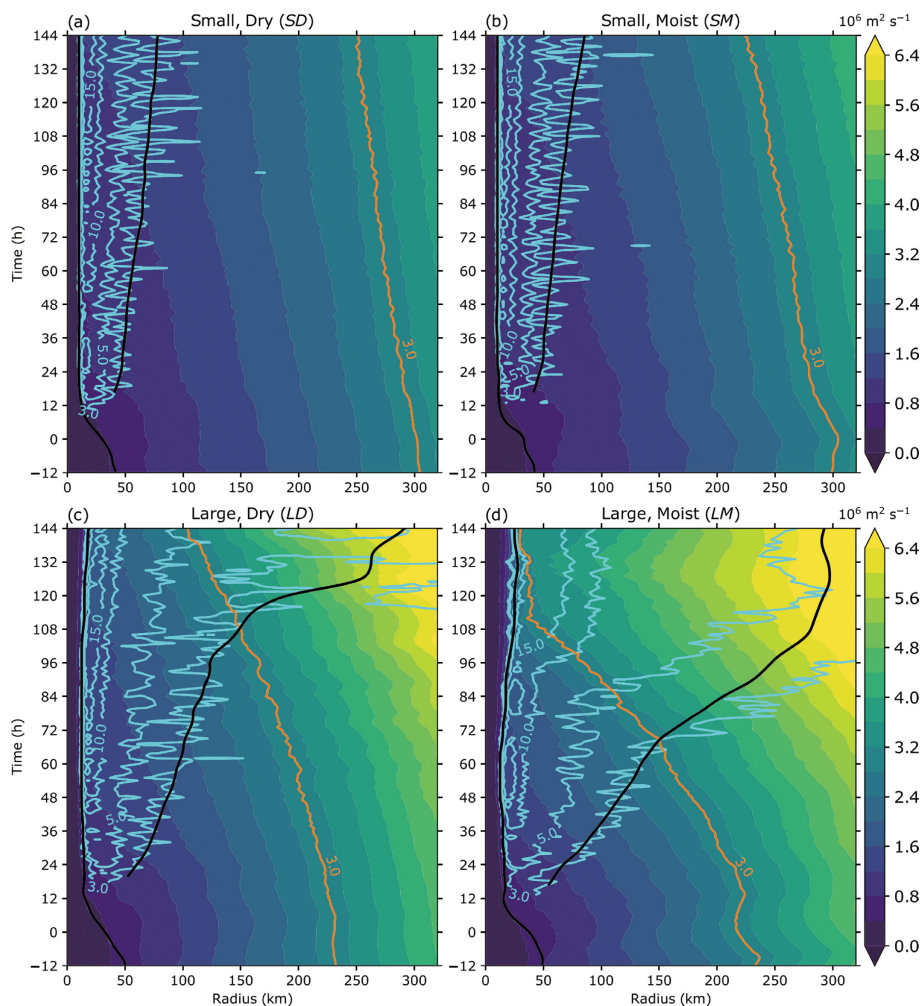
Fig. 7. AAM at z = 1 km (shaded), radial velocity averaged from surface to z = 1 km (cyan contours at 3, 5, 10, and 15 \text{m s}^{-1} ) for the simulations: (a) small incipient vortex in the dry environment, (b) small incipient vortex in the moist environment, (c) large incipient vortex in the dry environment, and (d) large incipient vortex in the moist environment. The AAM contour of 3.0 \times 10^6 \text{ m}^2 \text{ s}^{-1} is shown in orange. The inner black line represents RMW, while the outer black line represents the radius of gale-force winds. Figure 6 of Martinez et al. (2020).
