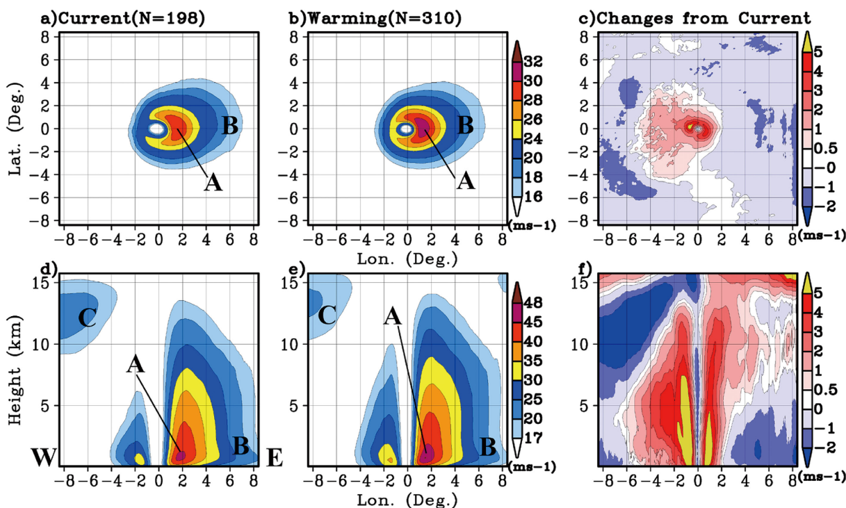
Fig. 15. Composite of TC-centered 10-m wind fields when the TC center was located in [142–147°E, 35–40°N] in the (a) current and (b) warming climates. The differences with respect to the current climate is shown in (c). (d)–(f) Same as (a)–(c), but for vertical cross sections of horizontal wind speeds. ‘A,’ ‘B,’ and ‘C’ in the panels indicate the areas of high winds, moderate wind speeds, and the jet, respectively. Figure 3 of Kanada et al. (2020).
