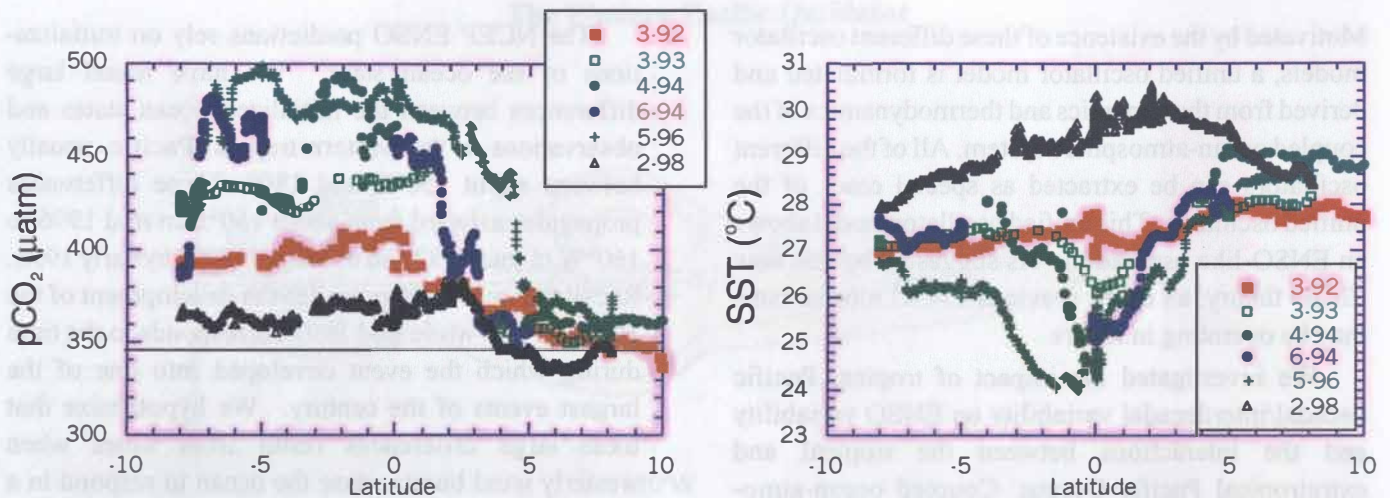
Figure 10. Changes of p\text{CO}_2 (left) and SST (right) over time along 110^\circ\text{W} in response to the ENSO cycle. During El Niños, the efflux of \text{CO}_2 is depressed. The dates in the panel, denoted by the month followed by the year (e.g., 6-94), give the dates when the data were collected.
