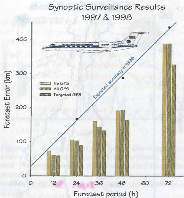
Figure 27. Results of data denial experiments with synoptic surveillance observations, illustrating ~15% improvement of already very good forecasts.
