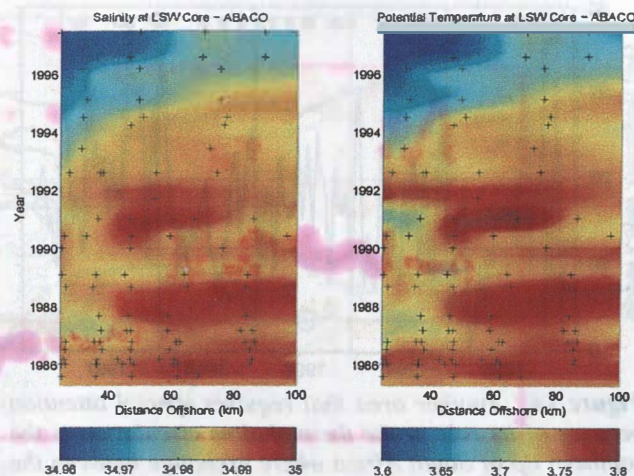
Figure 12. Time series of temperature and salinity at the depth of Labrador Sea Water obtained from data collected east of Abaco Island, the Bahamas (26.5°N). Crosses represent station positions. The section is taken across the axis of the Deep Western Boundary Current. The Deep Western Boundary Current transports Labrador Sea Water from its source region in the Labrador Sea to south of the equator and is an important component of the global meridional overturning circulation. Prior to 1993, temperature and salinity characteristics are relatively uniform. After 1993, temperature and salinity begin decreasing dramatically, beginning at the boundary and then extending offshore. This change in water mass characteristics indicates the arrival of Labrador Sea Water formed some 10 years earlier, indicating that the Deep Western Boundary Current advects waters from the Labrador Sea at faster rates than previously thought. These findings have important implications in studies of the ocean's ability to uptake atmospheric gases such as carbon dioxide.
