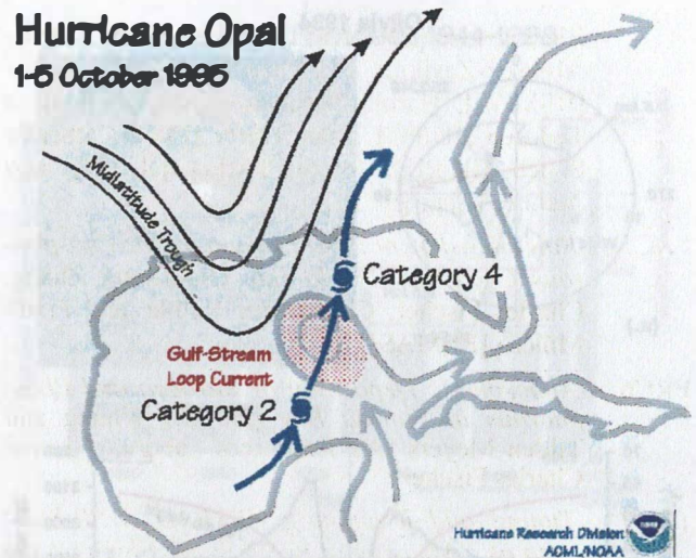
Figure 28. Hurricane Opal intensified rapidly under the influence of a “digging” mid-latitude trough as it careened northward across a warm eddy spun off from the Gulf Stream toward the U.S. coast.
