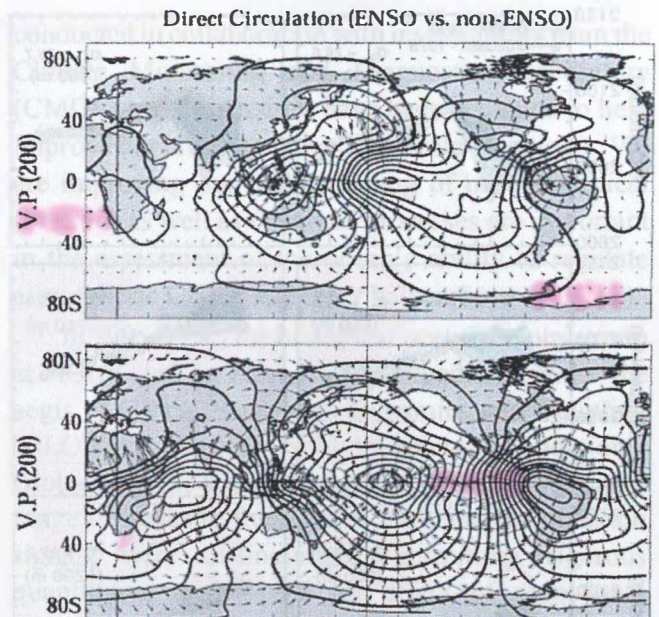
Figure 4. Anomalous distributions of the tropospheric direct circulation associated with the global ENSO (top) and non-ENSO (residual) variabilities in the equatorial Pacific. Top Panel: Composite average of 200 hPa velocity potential and irrotational velocity associated with positive-minus-negative phases of the global ENSO variability in the NINO3 region (see Figure 3, middle panel). Features to note are (1) the lateral convergence and implied suppressed convection west of the dateline and over northern South America, plus (2) the enhanced (suppressed) Hadley circulation in the central North Pacific (North Atlantic). Bottom Panel: Composite average of 200 hPa velocity potential and irrotational velocity associated with the change in the residual NINO3 SST between two multidecadal periods: 1978-1999 minus 1950-1977 (see Figure 3, bottom panel). Features to note include: (1) convergence (divergence) just east of the dateline (over South America), where the global ENSO shows divergence (convergence); and (2) anomalous Hadley circulations in the central North Pacific and North Atlantic that are opposite to those of the global ENSO mode.
