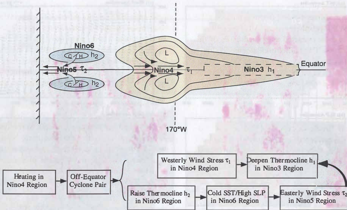
Figure 9. Schematic diagram of the western Pacific oscillator for ENSO. Condensation heating in the western central Pacific induces a pair of off-equatorial cyclones with westerly wind anomalies on the equator. These equatorial westerly wind anomalies act to deepen the thermocline and increase SST in the equatorial eastern Pacific, thereby providing a positive feedback for anomaly growth. On the other hand, the off-equatorial cyclones raise the thermocline there via Ekman pumping. Thus, a shallow off-equatorial thermocline anomaly expands over the western Pacific leading to a decrease in SST and an increase in SLP in the off-equatorial western Pacific. During the mature phase of El Niño, this off-equatorial high SLP initiates equatorial easterly wind anomalies in the western Pacific. These equatorial easterly wind anomalies cause upwelling and cooling that proceed eastward as a forced ocean response providing a negative feedback for the coupled ocean-atmosphere system to oscillate. Scientists at AOML are continuing to work on ENSO mechanisms by developing a unified ENSO oscillator model that includes the delayed oscillator, the western Pacific oscillator, the recharge-discharge oscillator, and the advective-reflective oscillator.
