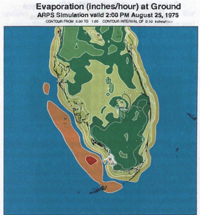
Figure 20. Evaporation valid at 2:00 p.m., August 25, 1975 from an ARPS mesoscale atmosphere model simulation over the Florida Area Cumulus Experiment (FACE) mesonet region. The evaporation pattern correlates well with the strongest divergent and initially driest surface wind fields, in the vicinity of the greatest surface-to-air temperature/humidity differences. Moisture was picked up by the atmospheric flow over Lake Okeechobee and by the organized offshore downdrafts associated with the west coast sea breeze circulation, while the Florida Everglades "muck" soil in the interior of the state tended to resist evaporation due to its high water retention and strong capillary forces. Thus, a significant north-south mesoscale gradient in evaporation was simulated across Florida Bay.
