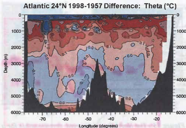
Figure 11. Decadal variability in surface heat fluxes can most clearly be seen from high quality hydrographic sections sufficiently accurate enough to measure the small changes in temperature seen between sections taken during different epochs. The ocean effectively integrates small changes in surface heat flux that result in small biases in sea surface temperature which become subducted and overturned into the deep water. Repeat hydrographic measurements taken at the same location through time can then be differenced to get indicators of climate change. Shown here is the temperature difference along pressure surfaces between the Ronald H. Brown (1998) and Discoverer (1957) hydrographic sections. Large warming of the water column from 300-2500 m is seen, suggesting increased surface heating in the northern North Atlantic over these decades. The strong negative temperature difference above 300 m is due to the fact that the 1957 data was taken during summer and the 1998 data was taken during winter.
