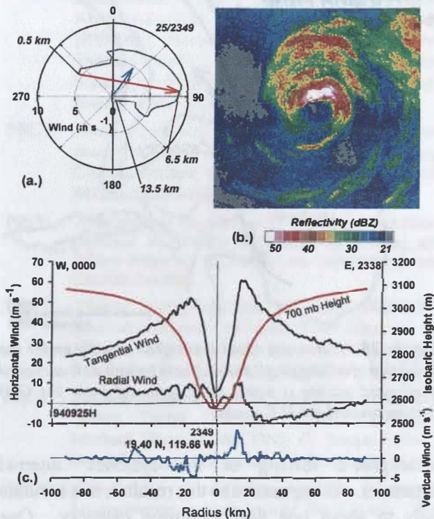
Figure 29. Eastern-Pacific Hurricane Olivia in westerly shear: (a) “environmental” hodograph; (b) radar reflectivity; and (c) flight-level wind and 700 mb height.
