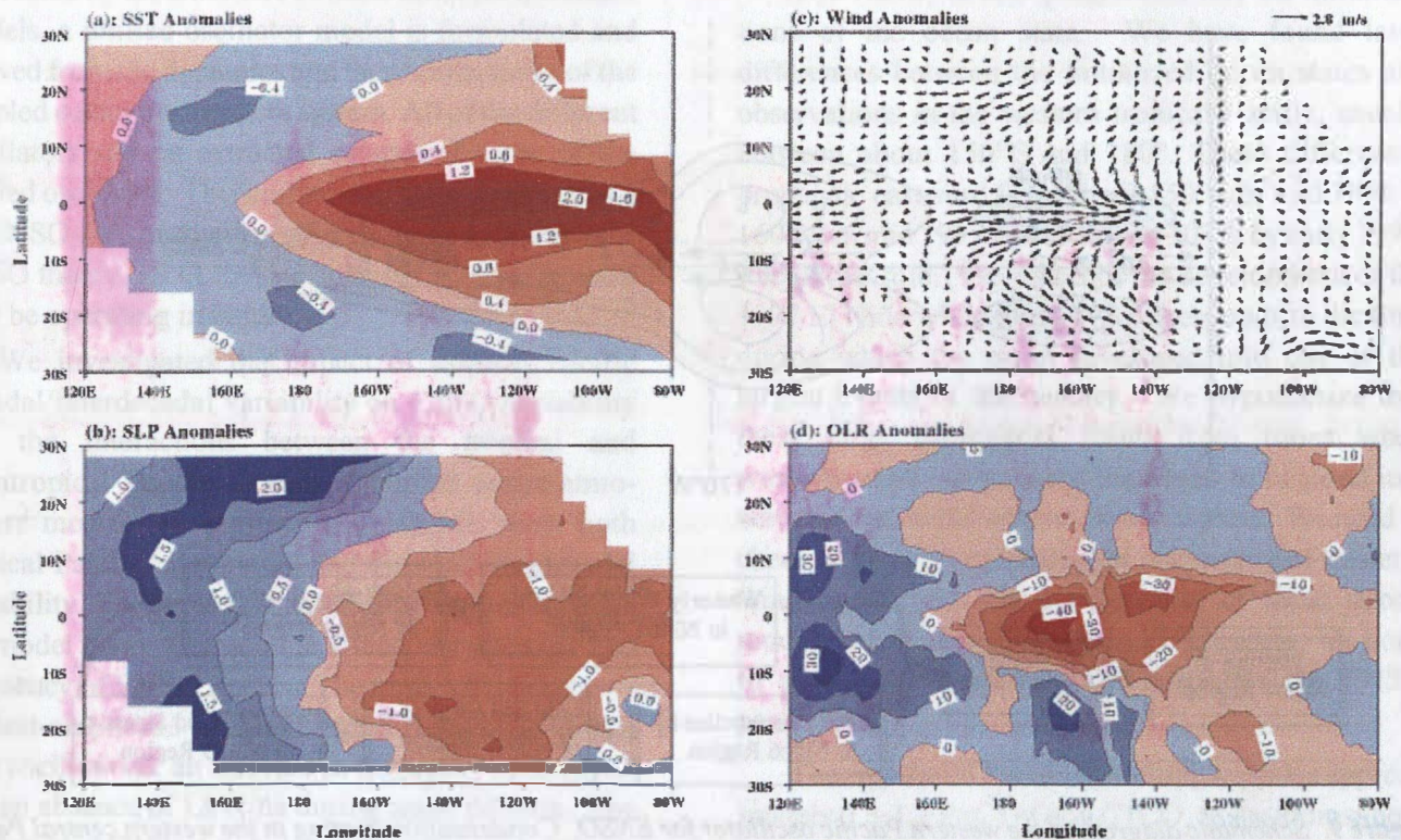
Figure 8. The El Niño composite of (a) SST anomalies, (b) SLP anomalies, (c) surface wind anomalies, and (d) OLR anomalies (Wang et al., 1999). El Niño displays western Pacific anomaly patterns in addition to eastern Pacific anomaly patterns. During the peak phase of El Niño, warm SST and low SLP anomalies in the equatorial eastern Pacific and low OLR anomalies in the equatorial central Pacific are accompanied by cold SST and high SLP anomalies in the off-equatorial western Pacific and high OLR anomalies in the off-equatorial far western Pacific. Also, while the zonal wind anomalies over the equatorial central Pacific are westerly, those over the equatorial far western Pacific are easterly. AOML is studying these neglected western Pacific relationships and is consolidating them into a unified theoretical model that combines them with the postulated mechanisms of other ENSO scientists.
