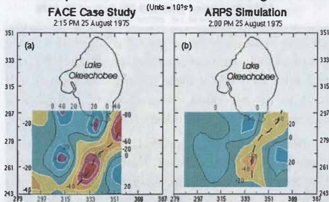
Figure 21. The divergence of the surface winds diagnosed from (a) real observations from the Florida Area Cumulus Experiment (FACE) mesonet region, and (b) and ARPS mesoscale atmospheric model simulation for the same case. When realistic land surface characteristics are incorporated into the model, the porous, cultivated land south of Lake Okeechobee causes enhanced diurnal surface heating, which results in more abrupt divergent deflections of the surface winds over the lake. This increases the convergence of the wind field over the agricultural land (heavy dashed line) and causes a thunderstorm complex to develop immediately south of the lake, similar to the convective cells diagnosed in the real data. Thus, the crescent-shaped band of maximum rainfall associated with the lake breeze shifts from east of Lake Okeechobee to its southern shore.
