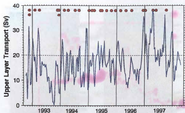
Figure 14. Another area that requires special attention because of its role in the thermohaline circulation is the southern tip of South Africa where exchange between the Indian and Atlantic Oceans takes place. One of the key questions still to be answered is how much heat and salt is transferred from the Indian to the Atlantic Ocean and what are the processes involved in this exchange. This figure shows the time series of the upper layer, westward baroclinic mass transport from the Indian to the Atlantic Ocean (solid line), and times when Agulhas rings were shed (circles). The transport was calculated using a combination of hydrographic and altimeter data and a simple model that relates the sea height anomaly with the depth of the upper layer. A strong interannual variability is observed. During 1997, the average transport of the Agulhas Current is significantly higher (23 Sv) than the long term mean (15.7 Sv). In spite of the high transport in 1997, the number of rings shed at the retroflection (4) was smaller than the other years (4 to 7), but each one of the rings transported twice the average volume of mass and heat. Variability of the strength of the retroflection and number and size of the eddies shed have a direct implication on the thermohaline circulation. Further observational and theoretical studies are needed to fully understand the process and its role in the global climate.
