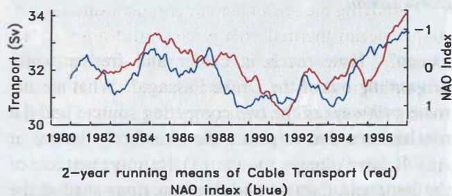
Figure 13. Florida Current transports are measured from West Palm Beach, Florida to the Bahamas via a submerged submarine cable. Voltage differences are measured at either end of the cable coupled with simple electromagnetic theory that says charged particles (water) moving through earth's magnetic field will create a current (voltage) which gives a measure of how fast the water is moving through the Straits of Florida. Measurements taken since 1982 show a high correlation (0.9) with the NAO Index. The NAO is a measure of variability in atmospheric surface pressure difference between Portugal and Iceland which has been shown to be correlated with the climate of the continental U.S. and hurricane formation. Continued measurements of Florida Current transport may help unravel the mystery of coupling between the ocean and atmosphere at decadal time scales.
