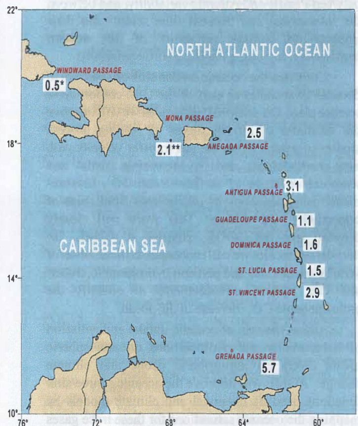
Figure 17. Direct measurements of transport in the Atlantic-Caribbean Passages from 1991–1998 have produced mean transports shown. Around 20 Sv of the approximately 32 Sv that flows through the Florida Straits enters the Caribbean south of the Virgin Islands, where southern hemisphere water masses dominate. A pilot program is underway (Caribbean Inflow Variability, with RSMAS and PMEL) to continuously measure the transport through the Grenada Passage via telephone cable and sea level to better understand the mesoscale transport variability and discern long-period changes in transport.
