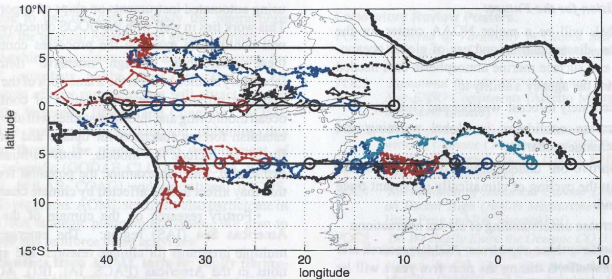
Figure 16. Trajectories of PALACE floats in the tropical Atlantic during the period July 1997 through November 1999 ballasted to drift at 1000 dbar and programmed to surface every 10 days to transmit in real time, via satellite, the profile obtained while rising to the surface. The instruments were deployed during the 1997 R/V Seward Johnson cruise (solid black lines). Each submerged trajectory segment is shown as a line starting at a dot. The trajectories reveal three regions of different flow characteristics. The equatorial band is characterized by high velocities (long trajectory segments), with a mean speed between 1°S and 3°N of about 10 cm/s. Further north, 3–8°N, and further south, 2–8°S, the speed is about half as large (shorter trajectory segments). Another difference between the high and the low energy regimes is that, in the latter, some of the PALACE floats tend to stay a long time in a small area, e.g., the three red trajectories are more than two years long. The one near 5°S, 10°W does not reveal much displacement whereas the trajectories at and north of the equator cover large distances. Several zonal currents can be identified in the trajectories. These are the westward Equatorial Intermediate Current between about 1°S and 1°N, the Northern Intermediate Countercurrent in 2–3°N west of 25°W and at about 1°N further east, as well as the central branch of the intermediate South Equatorial Current between 2°S and 4°S (black and light blue trajectories starting at 6°S, 0–10°E). The flow pattern between 4°S and 8°S does not show persistent zonal currents over longer periods of time; instead, typical periods are shorter than four months.
