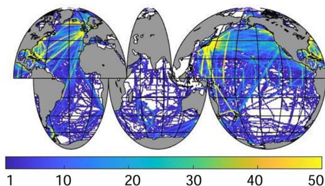
Figure 1: The number of individual months with 1°x1° gridded surface ocean f\text{CO}_2 values between 1970 and 2002. Reproduced from Bakker et al. 2024.
