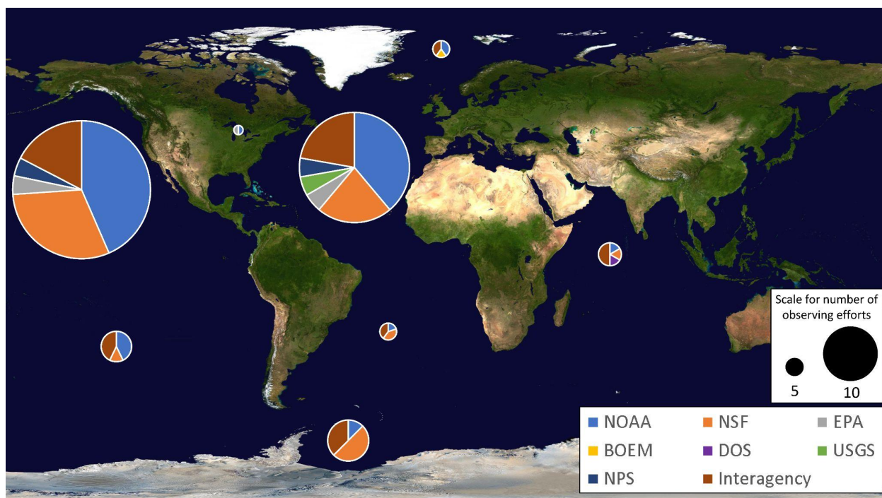
Figure 2: Sustained observing efforts and programs per ocean basin by an agency or interagency partnership (i.e., efforts conducted in partnership by two or more agencies) conducting the observing effort. If one effort collected measurements in multiple ocean basins, the effort was counted multiple times (once for each relevant basin). The size of the pie chart indicates the number of observing efforts, while color represents the agency conducting the observing effort(s).
