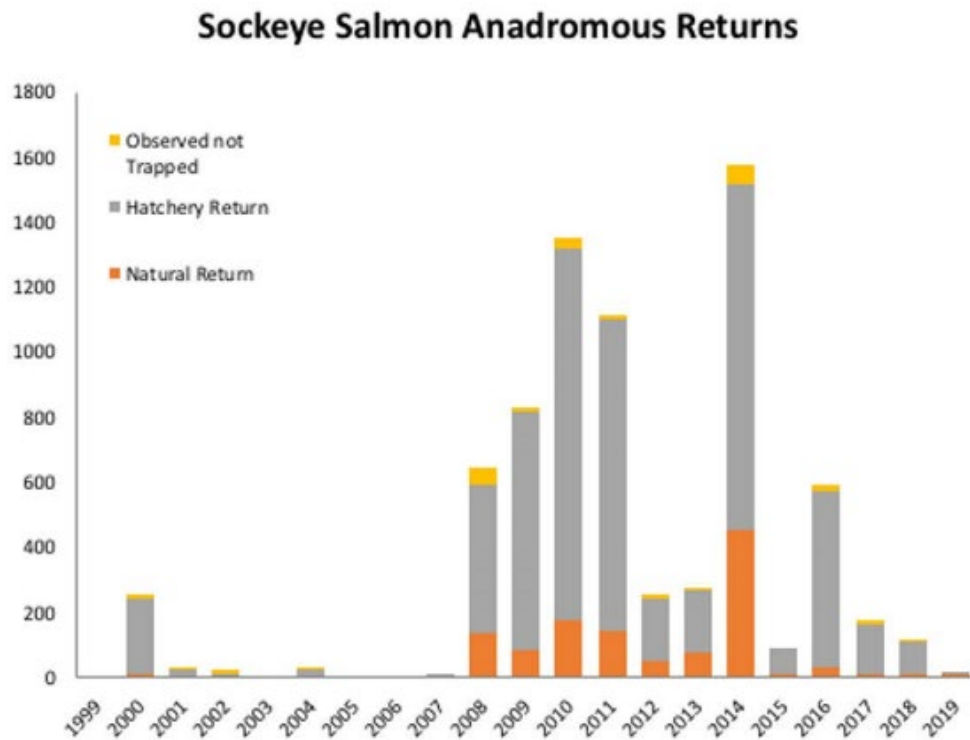
Figure 38. Snake River sockeye salmon anadromous returns, 1999–2019 (figure from Johnson et al. (2020)).
