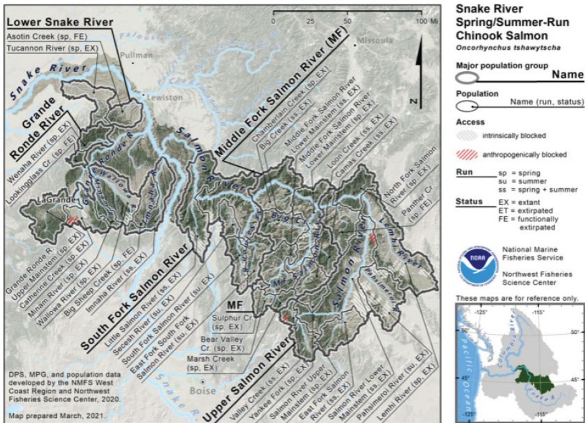
Figure 17. The Snake River spring/summer-run Chinook salmon ESU's spawning and rearing areas, illustrating populations and MPGs (Ford 2022).
