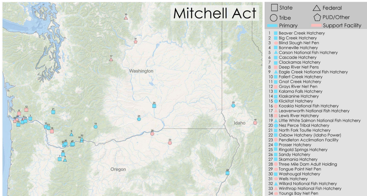
Figure 65. Hatchery facilities funded by Mitchell Act (NWPCC).
