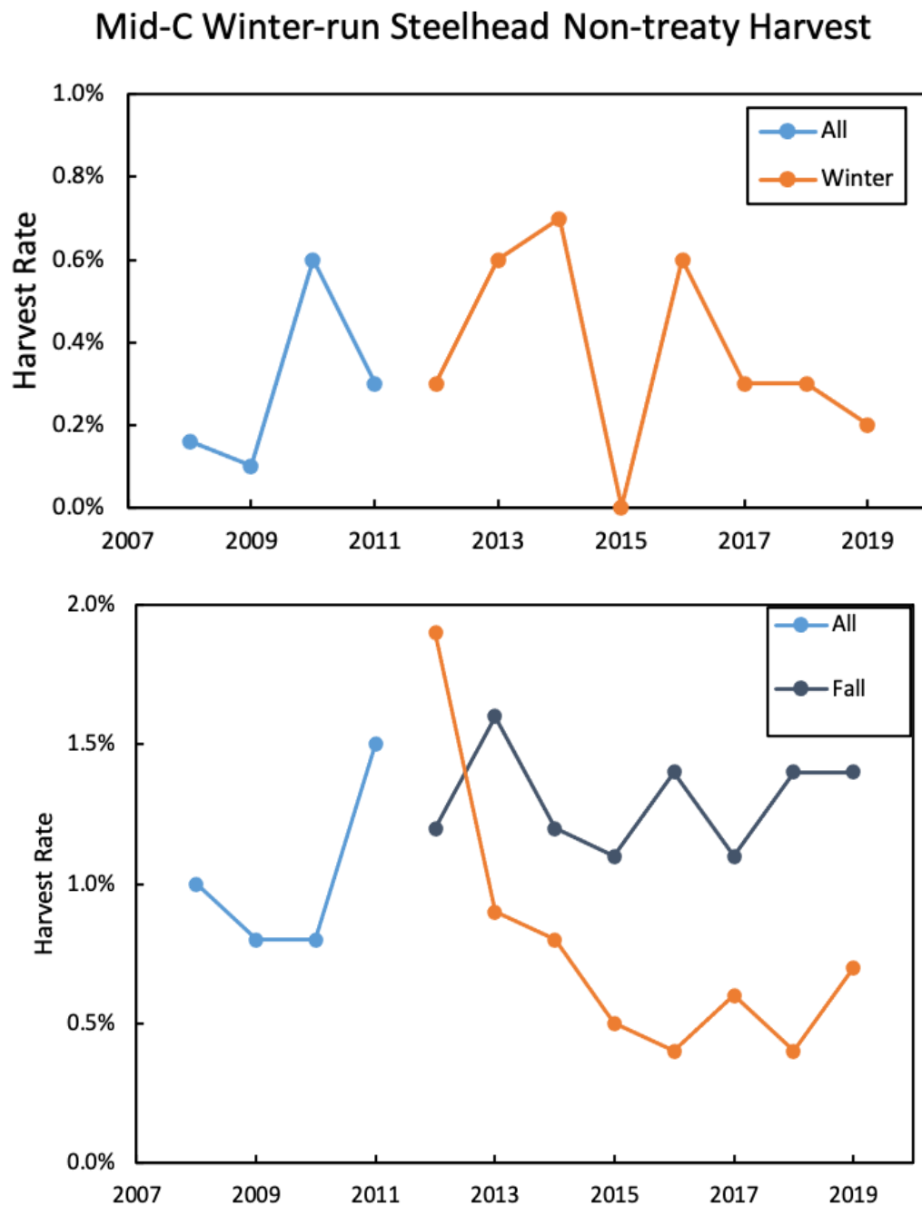
Figure 47. Non-treaty harvest impacts on natural winter- (upper panel) and summer-run (lower panel) steelhead from the Middle Columbia River steelhead DPS. As of 2012, harvest management reporting is broken into two periods, FA and W/SP/SU, where previously reporting was done by full calendar year (Figure reproduced from Ford (2022)).
