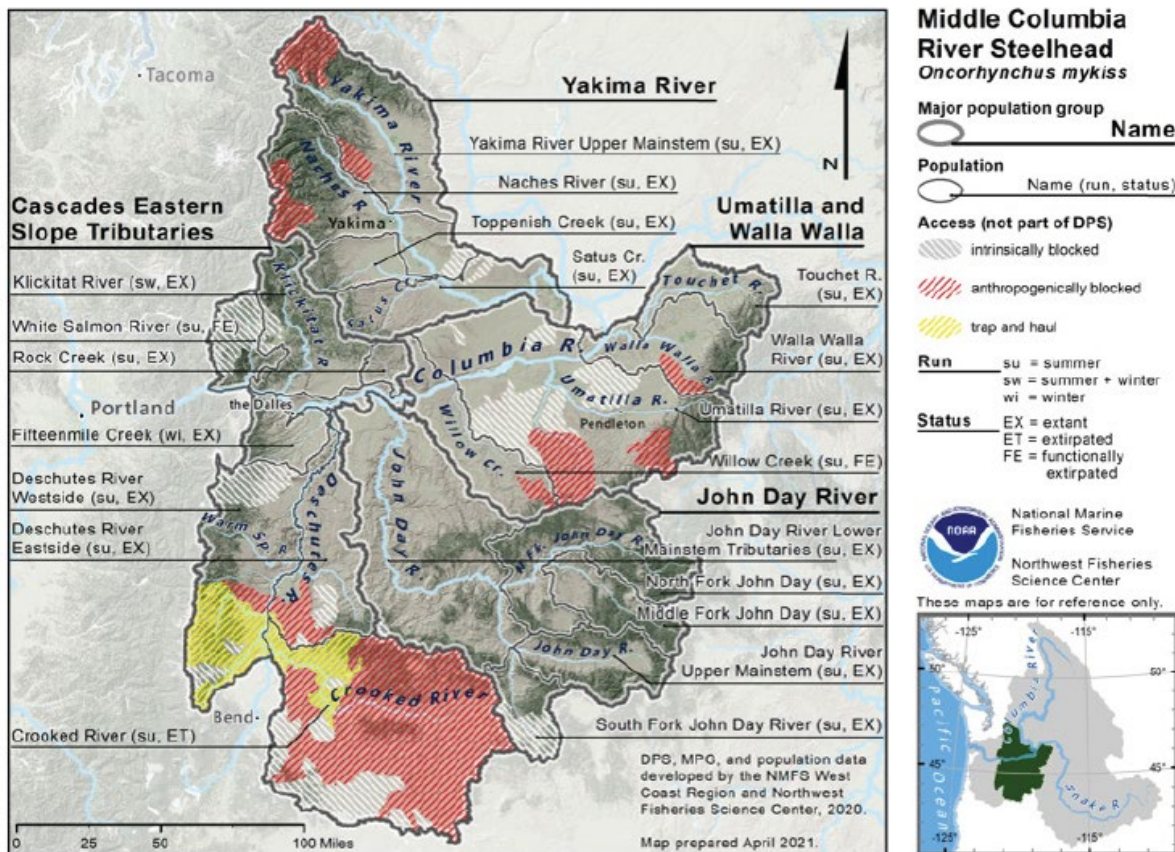
Figure 45. Map of the Middle Columbia River steelhead DPS's spawning and rearing areas, illustrating populations and MPGs (Ford 2022).
