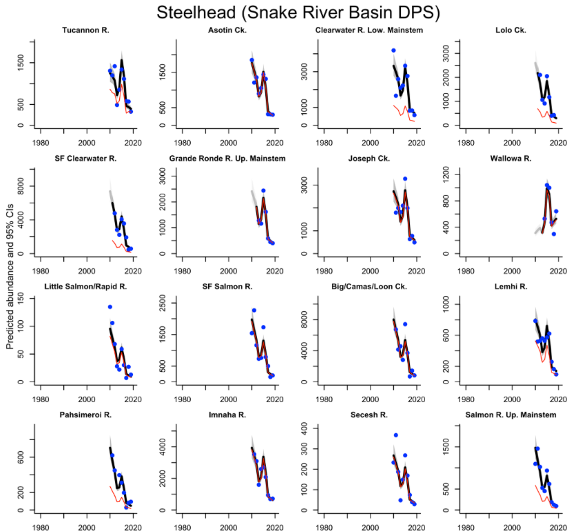
Figure 52. Smoothed trend in estimated total (thick black line, with 95% confidence interval in gray) and natural (thin red line) population spawning abundance. In portions of a time series where a population has no annual estimates but smoothed spawning abundance is estimated from correlations with other populations, the smoothed estimate is shown in light gray. Points show the annual raw spawning abundance estimates. For some trends, the smoothed estimate may be influenced by earlier data points not included in the plot (Ford 2022). a) Long-term dataset from weir and redd surveys. b) Super-population groups from Genetic Stock Identification (GSI)-based run partitioning of the run-at-large over Lower Granite Dam. c) PIT-tag-based population estimation method based on mixture model and tag detection network across the DPS.
