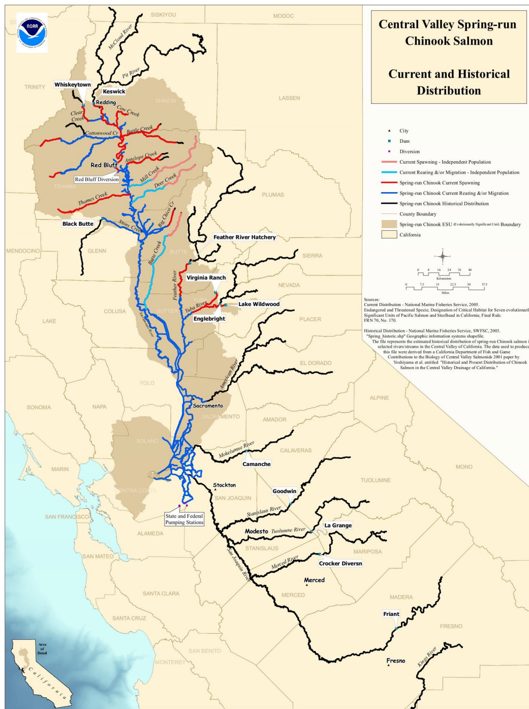
Figure 27. Map of the Central Valley Spring-run Chinook Salmon ESU's spawning and rearing areas, illustrating historical populations and diversity groups (NMFS 2014h).
