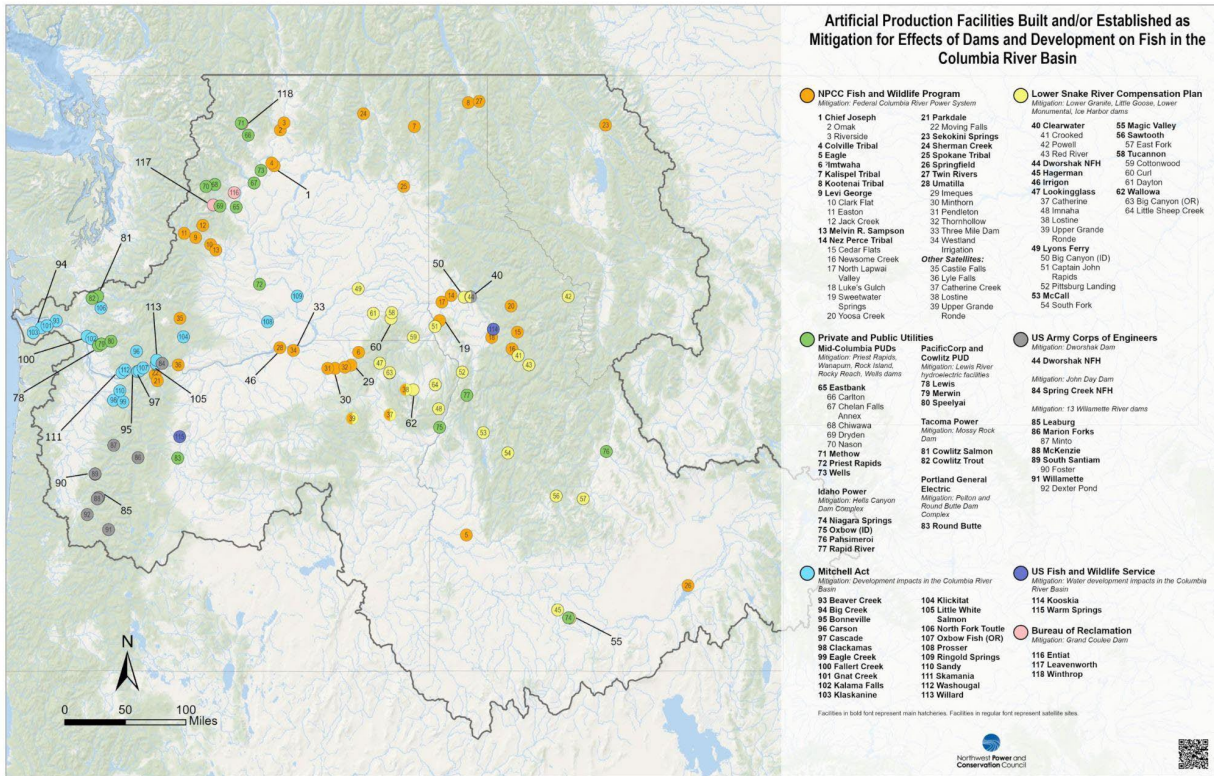
Figure 64. Mitigation hatchery facilities in the Columbia River Basin (NWPCC).
