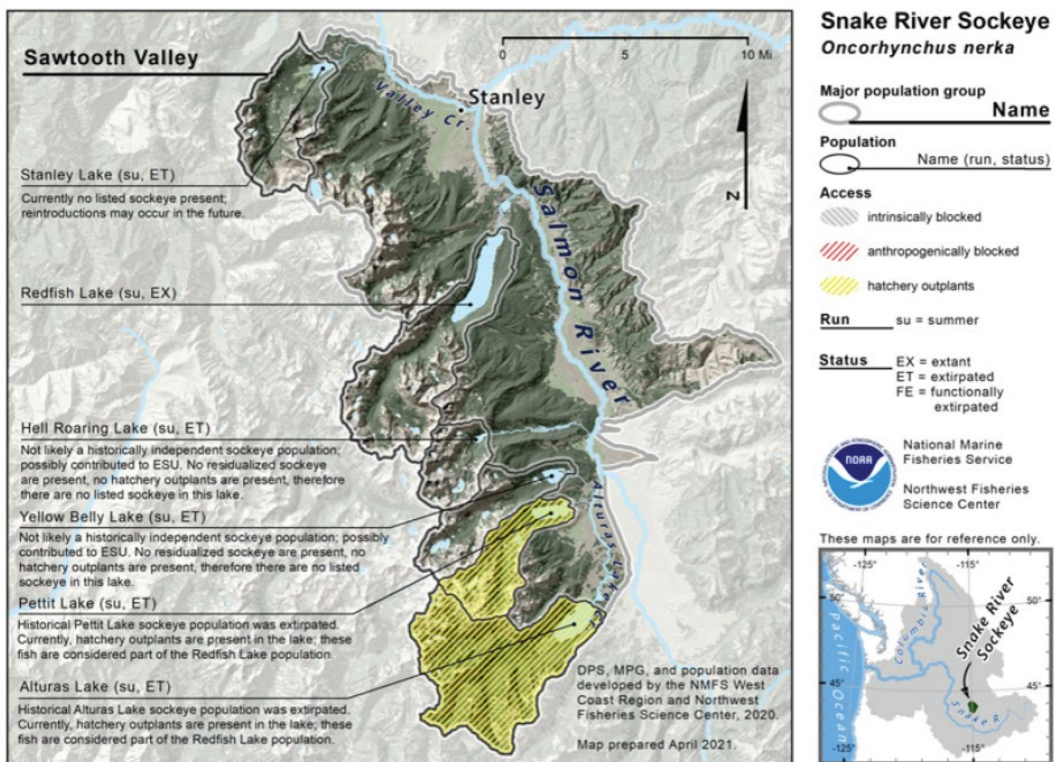
Figure 37. Map of the Snake River Sockeye Salmon ESU's spawning and rearing areas, illustrating populations and MPGs (Ford 2022).
