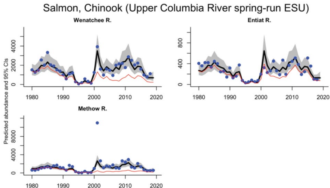
Figure 21. Smoothed trend in estimated total (thick black line, with 95% confidence interval in gray) and natural (thin red line) population spawning abundance. In portions of a time series where a population has no annual estimates but smoothed spawning abundance is estimated from correlations with other populations, the smoothed estimate is shown in light gray. Points show the annual raw spawning abundance estimates. For some trends, the smoothed estimate may be influenced by earlier data points not included in the plot (Ford 2022).
