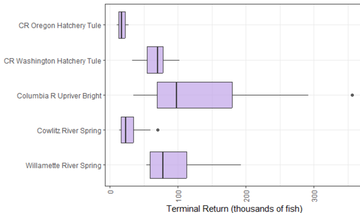
Figure 2: Summary of projected 2009-2018 returns to the river for FRAM stocks with Mitchell Act funded production. These projections are from the base '2019 PST' model runs without modified hatchery production and, with the exception of White River spring, represent only the marked component of each stock.
