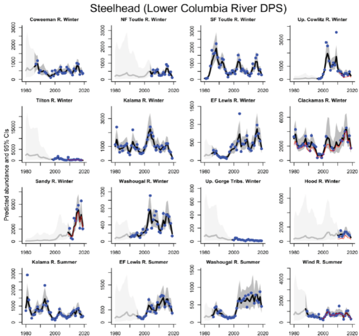
Figure 41. Smoothed trend in estimated total (thick black line, with 95% confidence interval in gray) and natural (thin red line) population spawning abundance. In portions of a time series where a population has no annual estimates but smoothed spawning abundance is estimated from correlations with other populations the smoothed estimate is shown in light gray. Points show the annual raw spawning abundance estimates. For some trends the smoothed estimate may be influenced by earlier data points not included in the plot (Ford 2022).
