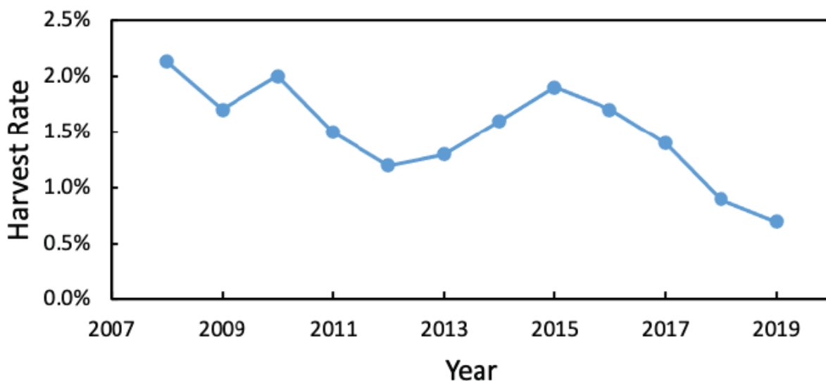
Figure 22. Non-treaty harvest rate for Upper Columbia River spring-run Chinook salmon. Data from the Columbia River Technical Advisory Committee (Figure reproduced from Ford (Ford 2022)).
