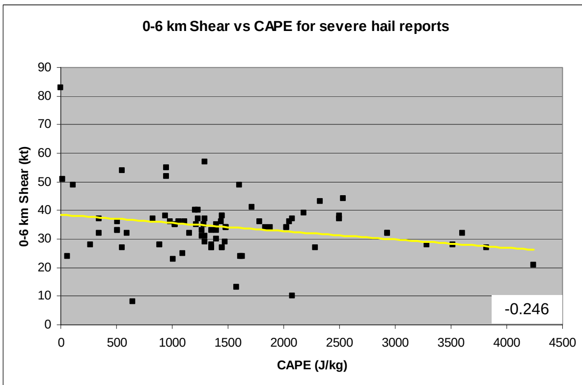
Figure 14. Scatter diagram of 0-6 km shear (kt) vs. CAPE ( \text{J kg}^{-1} ) for severe hail reports.
