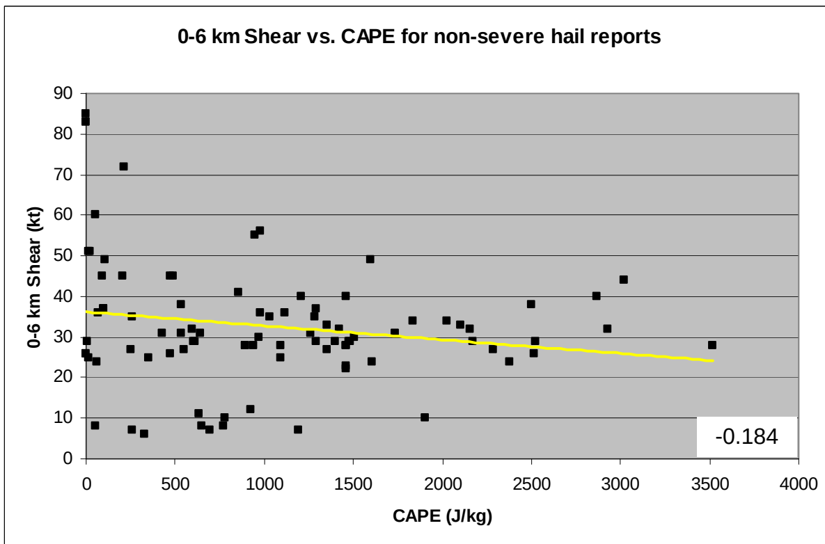
Figure 15. Scatter diagram of 0-6km shear (kt.) vs. CAPE ( \text{J kg}^{-1} ) for non-severe hail reports.
