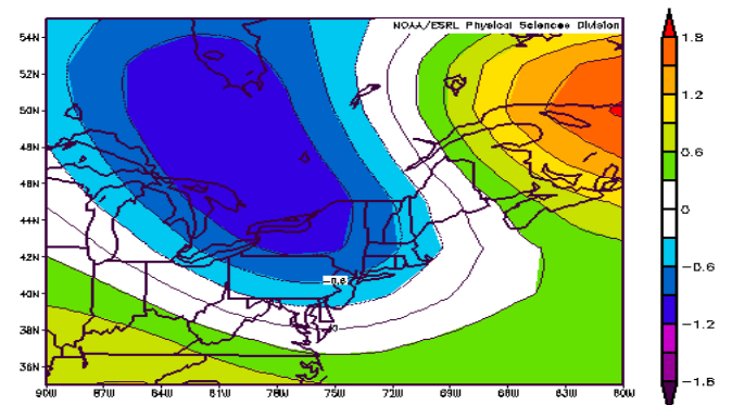
Figure 8. 500 mb mean temperature composite (upper left) and anomaly (lower right) ( ^{\circ}\text{C} ) for all hail days.
