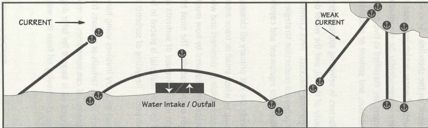
c/d Combination of exclusion and deflection
