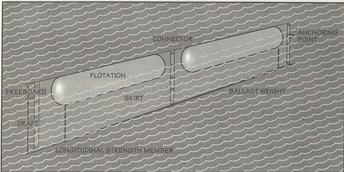
Figure 5. Major elements of standard boom.
