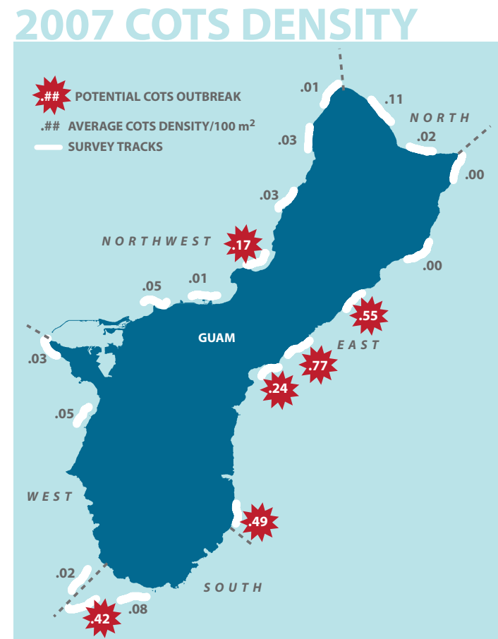
Figure 10. Densities (organisms/100 m 2 ) of crown-of-thorns seastars (COTS) from towed-diver surveys of forereef habitats conducted around Guam in 2007.
