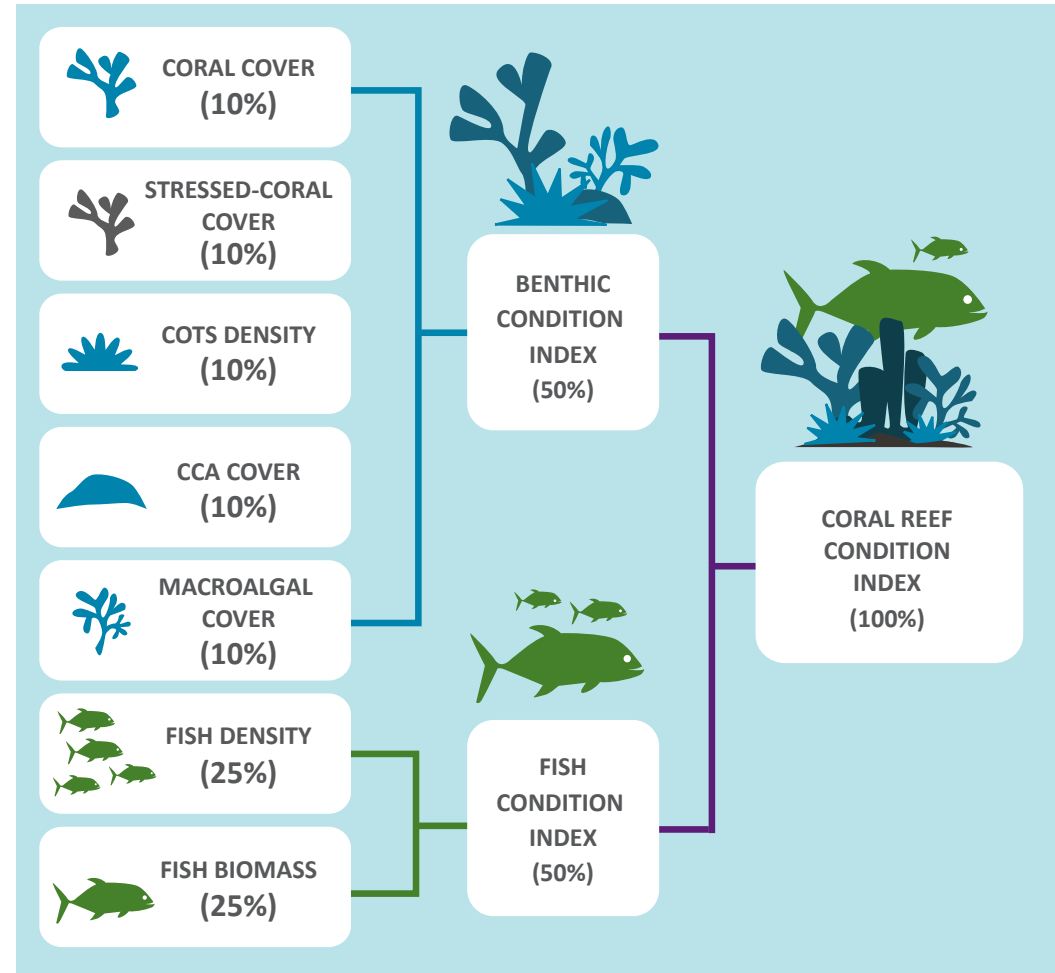
Figure 6. Conceptual diagram of the calculation of the 3 condition indices, which are based on data from towed-diver surveys conducted on forereef habitats during MARAMP cruises in 2005 and 2007. CCA stands for crustose coralline red algae and COTS for crown-of-thorns seastar.
