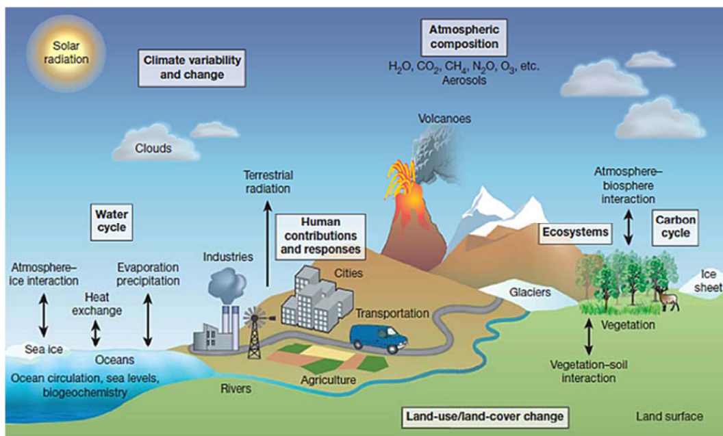
Figure 2 Schematic view of much of what needs to be considered in an Earth System Model (from www.gfdl.noaa.gov ). Atmospheric circulation, weather systems, the trace gases important for air quality and secondary aerosol formation, and ocean surface waves also have to be taken into account. Source: www.gfdl.noaa.gov ; adapted from Trenberth et al. (1995)
