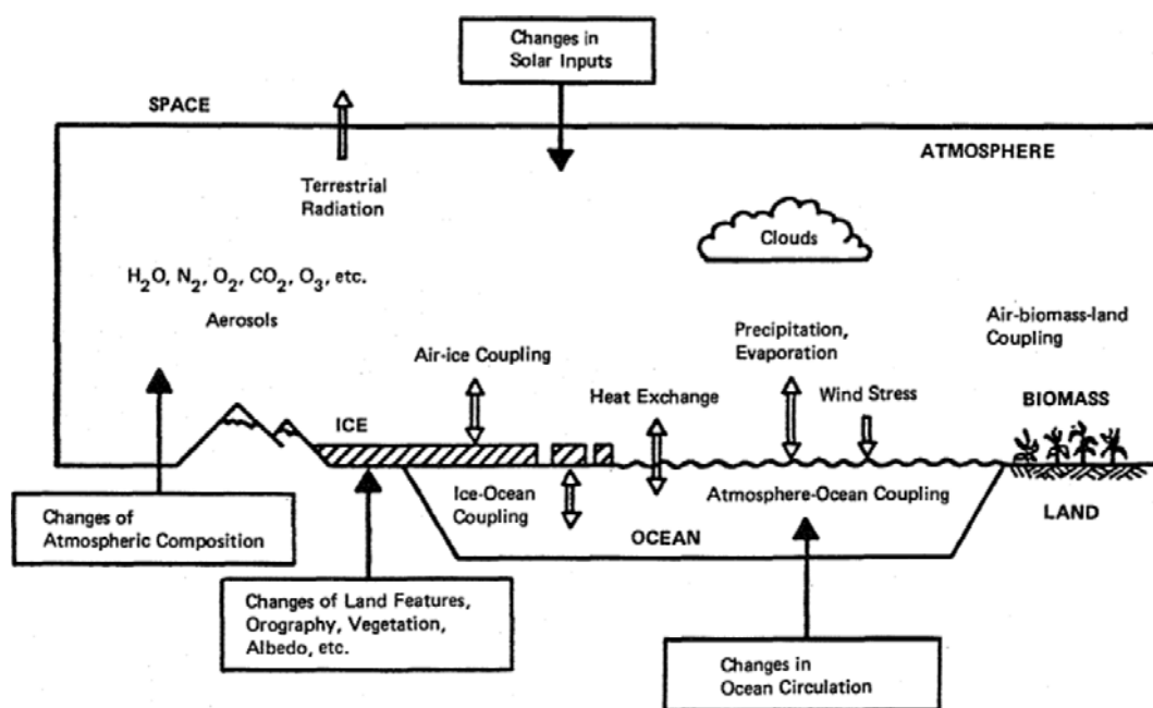
Figure 1 Schematic illustration of the Earth's climatic system, with some examples of the processes responsible for climate and its change, as presented by Source: Gates (1979) , adapted from NRC (1975).
