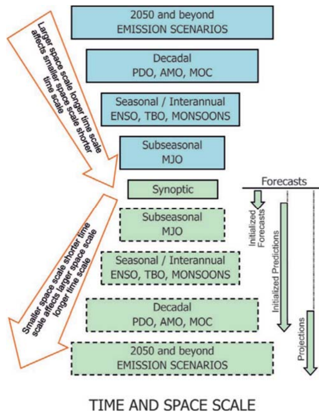
Figure 7 Schematic illustrating some of the interactions between various time and space scales in the climate system. Space scales and possible forecasts are indicated. From Source: Hurrell et al. (2009).
