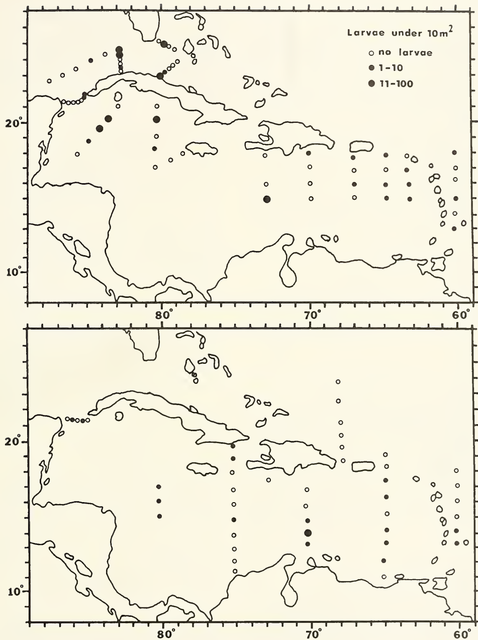
Figure 8.—Distribution and number per station of the bregmacerotid larvae Bregmaceros mucroflandii during Oregon II cruises 7239 (upper) and 7343 (lower).
