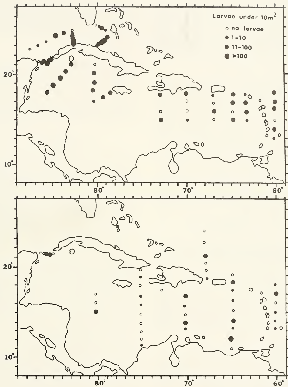
Figure 12.—Distribution and number per station of scard larvae during Oregon II cruises 7239 (upper) and 7343 (lower).
