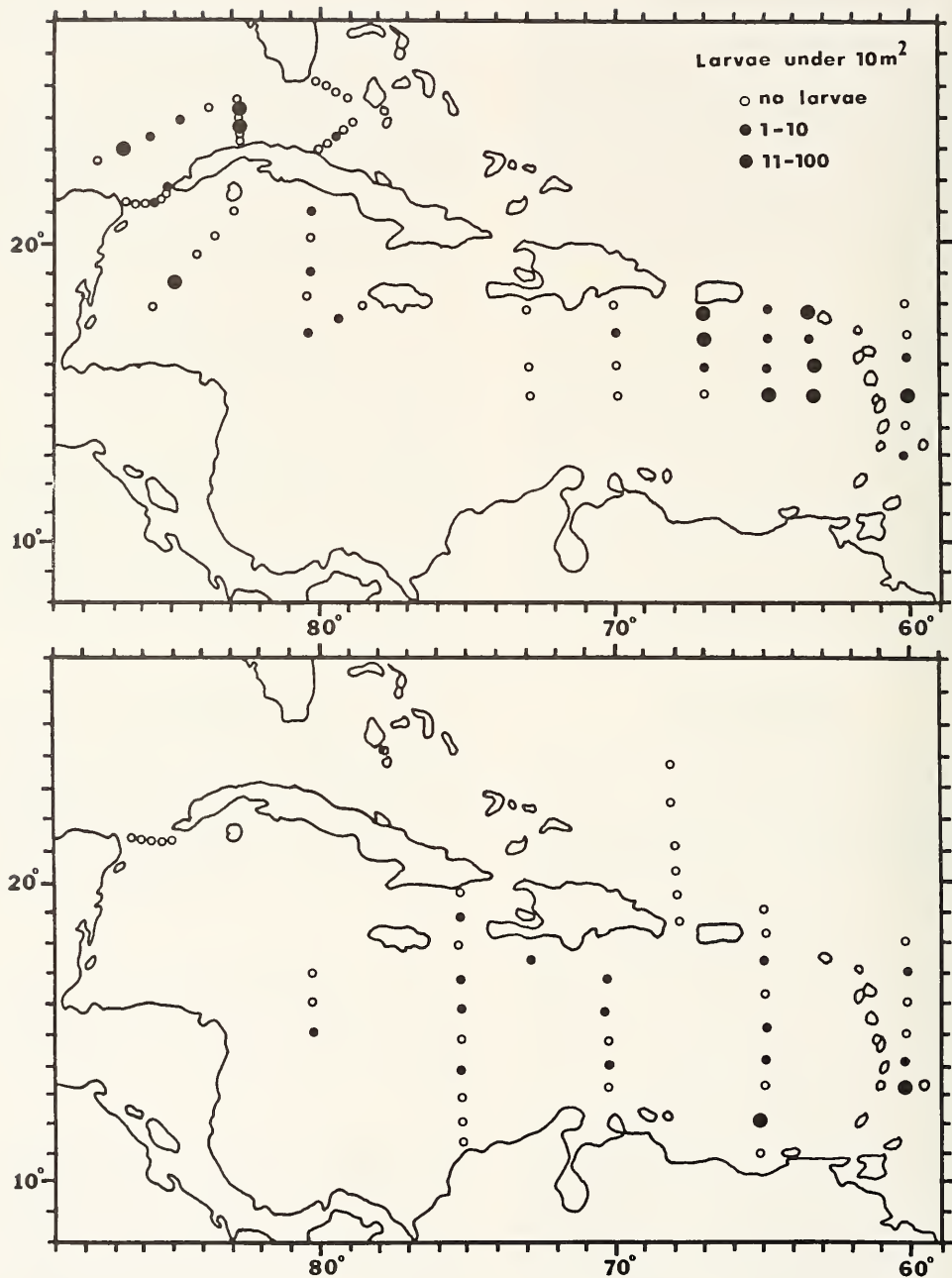
Figure 4.—Distribution and number per station of the paraplepid larvae Lestidium spp. during Oregon II cruises 7239 (upper) and 7343 (lower).
