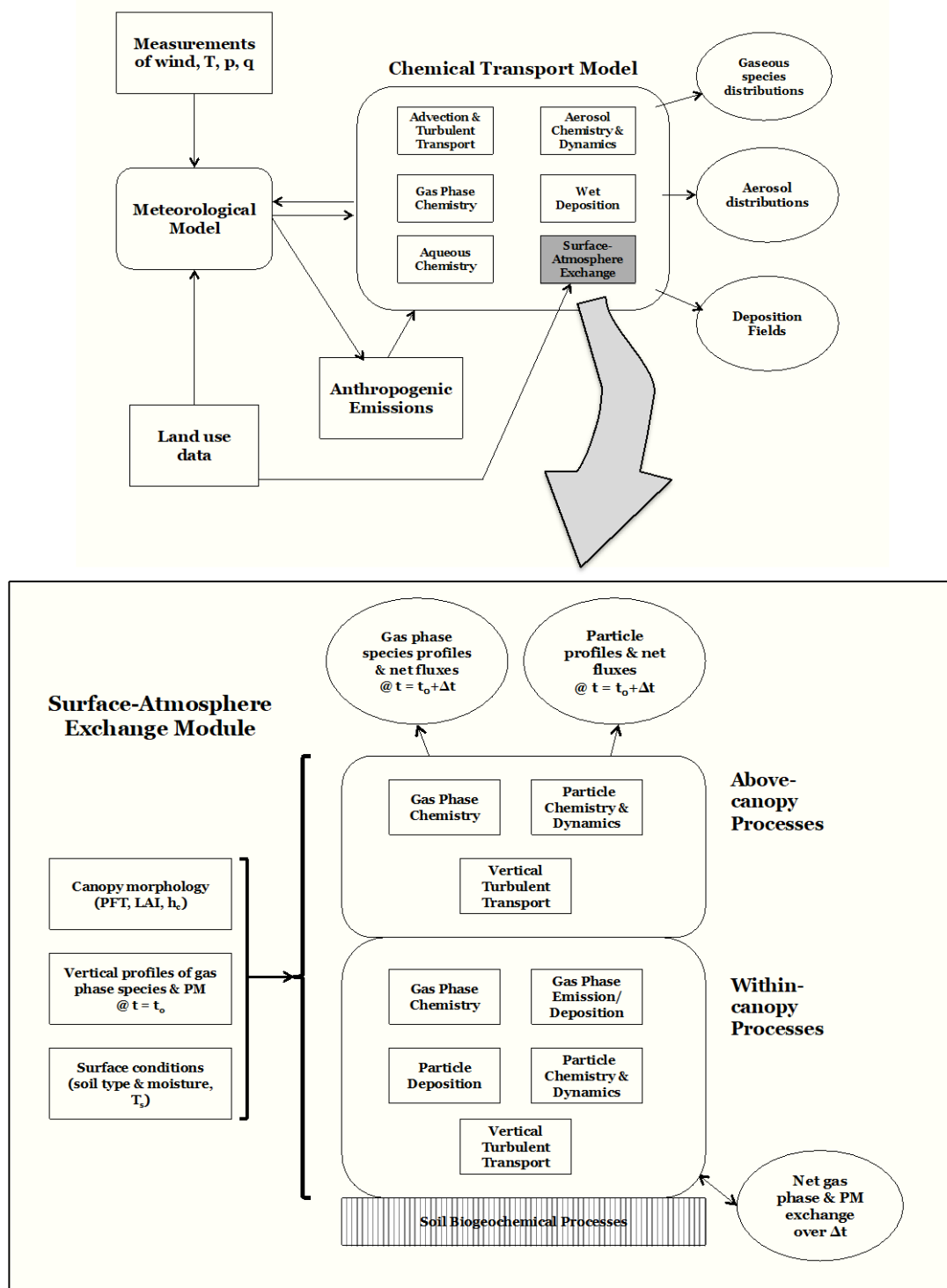
Figure 2. Potential Air Quality Model with Surface-Atmosphere Exchange Module
