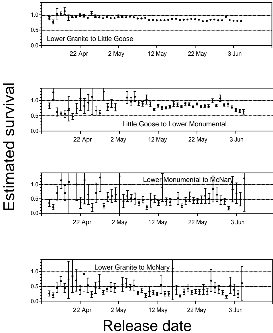
Figure 3. Estimated survival through various reaches versus release date at Lower Granite Dam for daily release groups of Snake River steelhead, 2004. Bars extend one standard error above and below point estimates.
