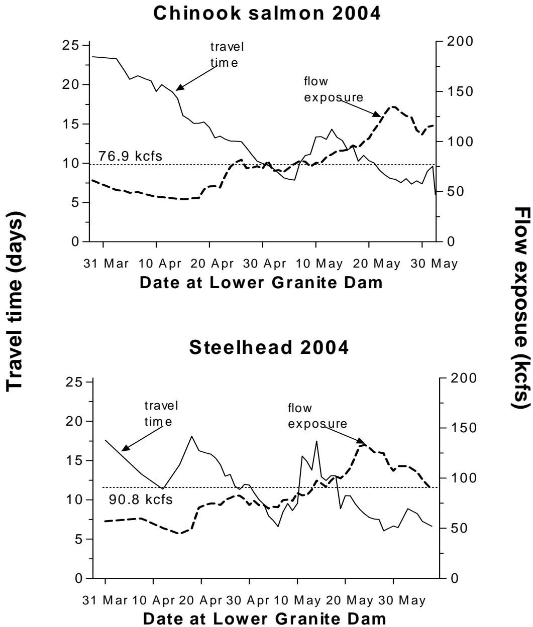
Figure 5. Travel time (days) for yearling Chinook salmon and steelhead from Lower Granite Dam to McNary Dam and index of flow exposure at Lower Granite Dam (kcfs) for daily groups of PIT-tagged fish during 2004. Dashed horizontal lines represent the annual average flow exposure index, weighted by the number of PIT-tagged fish in each group.
