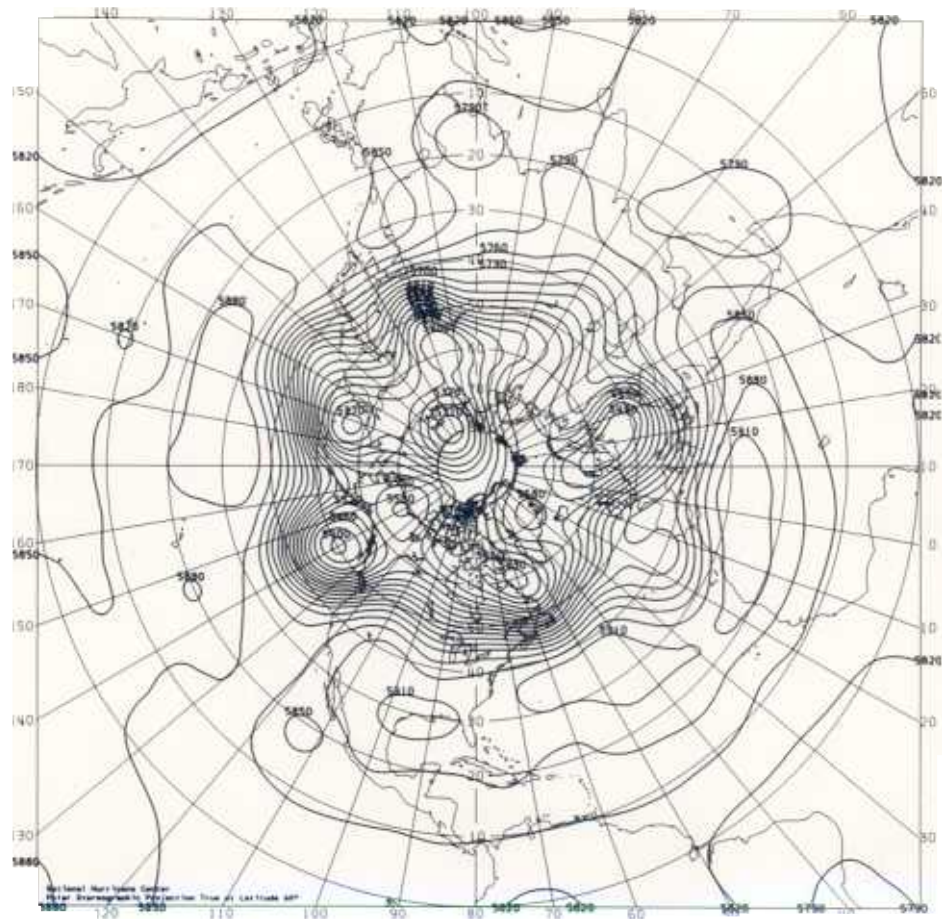
Figure 10. Northern Hemisphere 500-mb height field generated by the balance equation procedure for 1200 GMT 2 September 1978.
