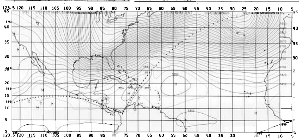
Figure 2. Same as Fig. 1, but with addition of heights interpolated from latest LFM initial analysis. Heavy dotted line is outer boundary of LFM analysis region.
