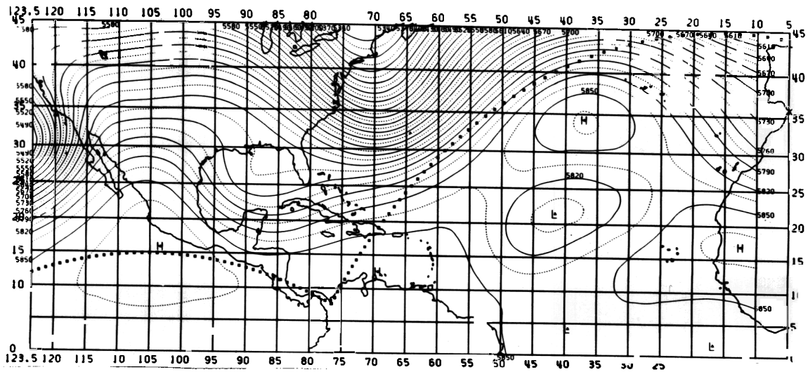
Figure 8. Generated 500-mb heights from balance equation procedure for 1200 GMT 31 March 1978.
