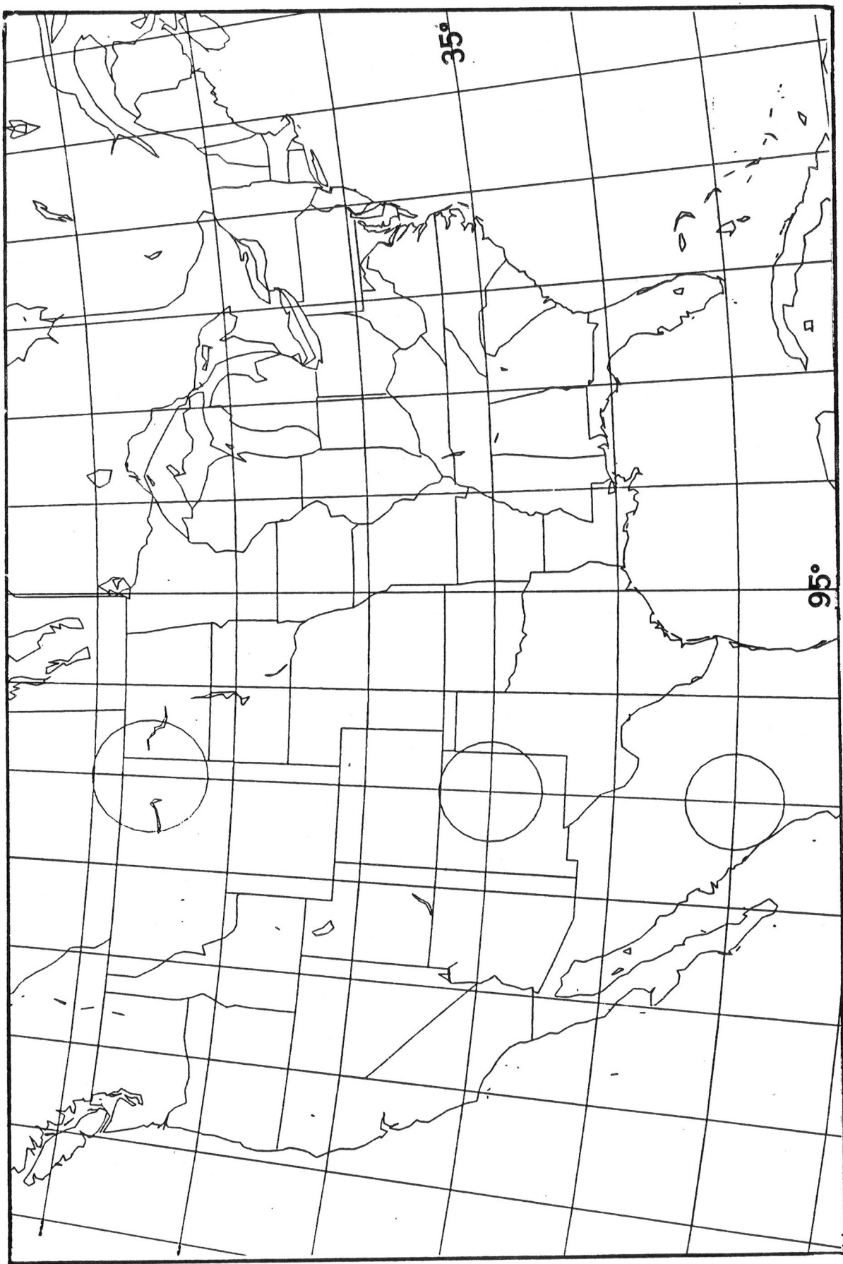
Figure 11. Same as Fig. 9, except a Lambert conformal tangent at 17.5° N.
