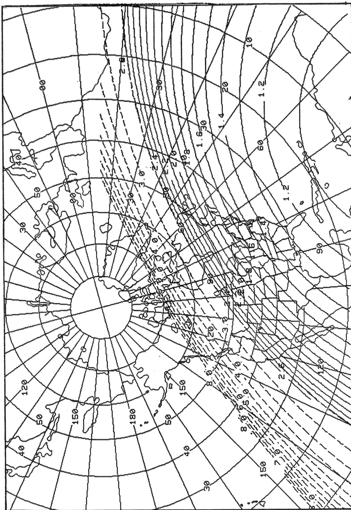
Figure 15. The maximum dimension D of the rectangle viewed by GOES EAST located at 75^{\circ} W. Contouring is at intervals of 0.1 km (solid lines), then at intervals of 0.5 km (dashed lines).
