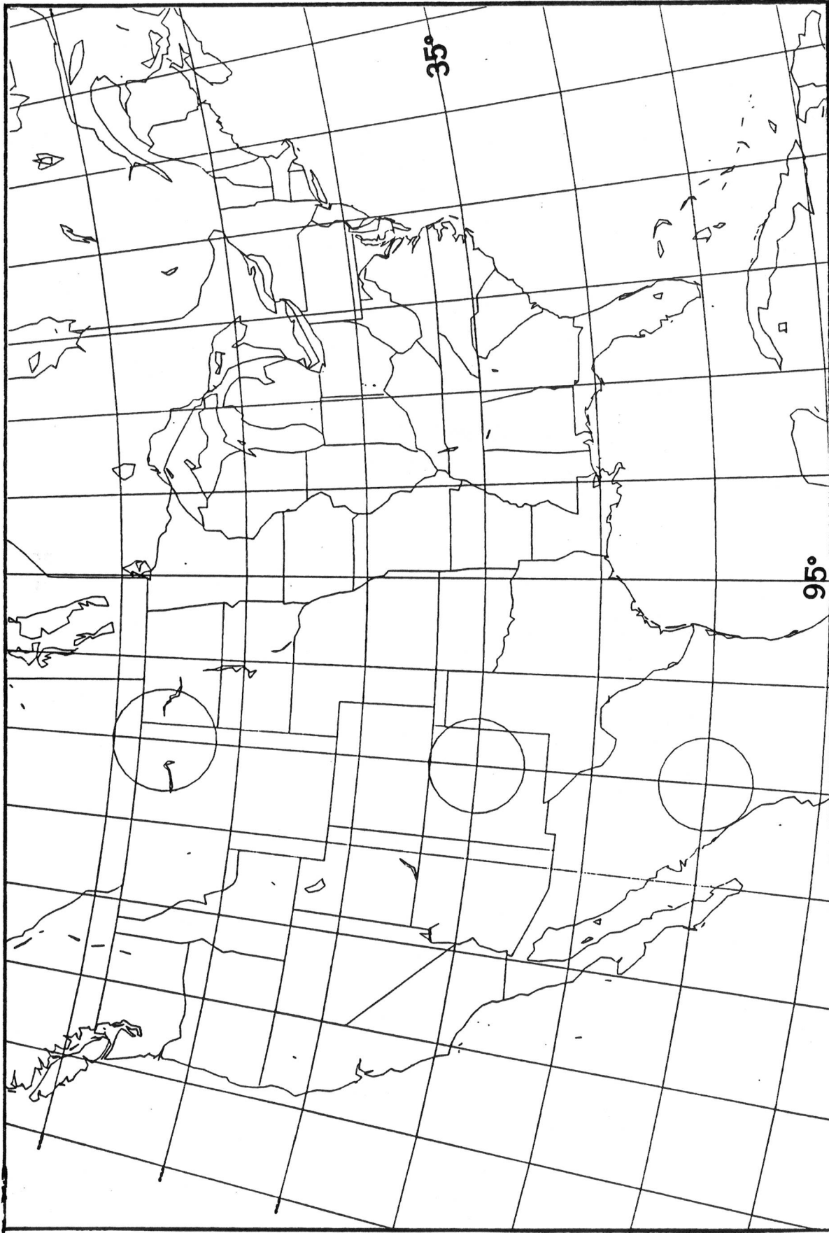
Figure 12. Same as Fig. 9, except a Lambert conformal tangent at 25^{\circ} N.
