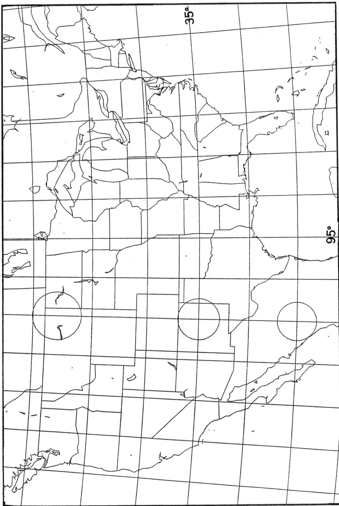
Figure 10. Same as Fig. 9, except a Lambert conformal tangent at 10^{\circ} N.
