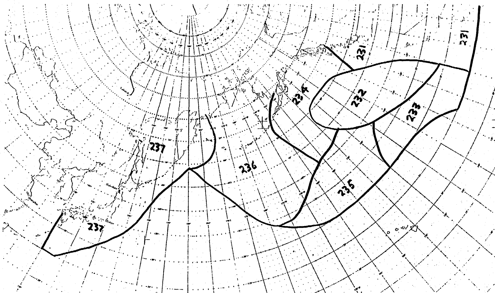
Figure 25. The fog forecasting regions for the North Pacific cool season. Regions are generally labeled from north to south and from the coast of North America seaward. The first number is 2 for cool season, and the middle number is 3 for Pacific.
