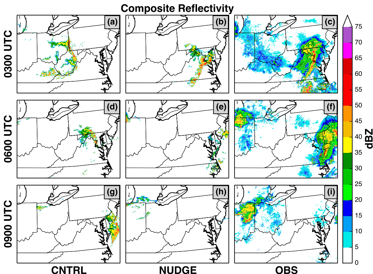
FIG. 7. As in Fig. 4, except results are displayed at 3-h intervals between 0300 and 0900 UTC 30 Jun 2012. The east central portion of the model domain is displayed.
