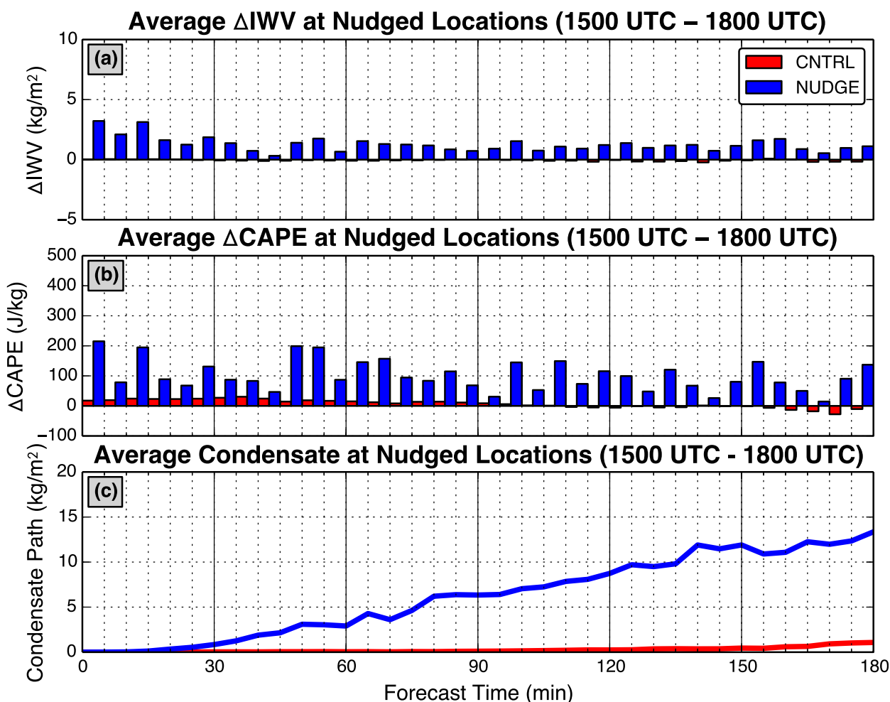
FIG. 17. Average temporal changes in (a) IWV and (b) CAPE at grid points where nudging is performed in NUDGE for the 17 Nov 2013 event. (c) Average column condensate (liquid and solid water path) at nudged locations. Red bars (barely visible) and lines represent results from CNTRL, while blue bars and lines represent results from NUDGE.
