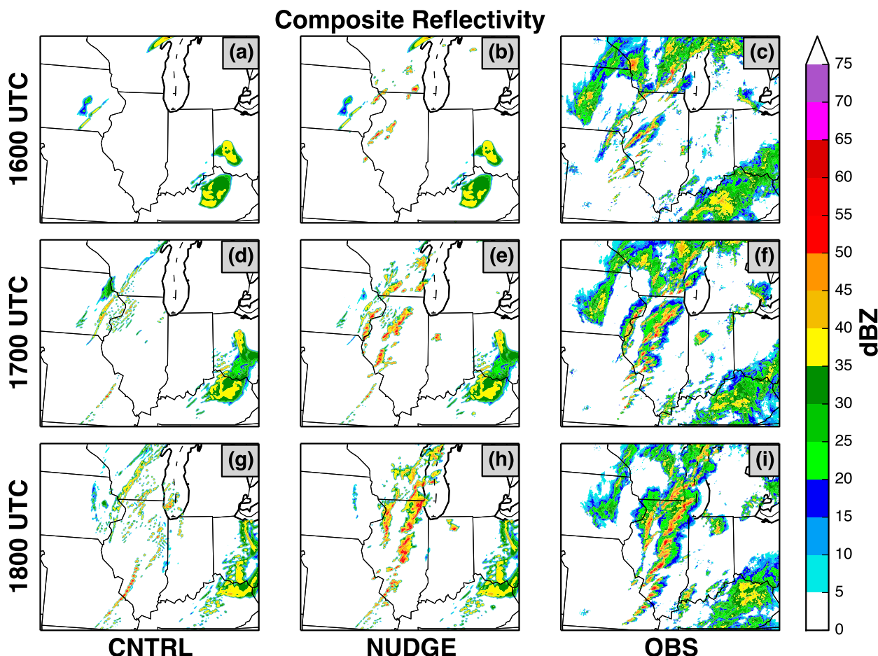
FIG. 18. Simulated and observed composite reflectivity for (top to bottom) the first three hours of the deterministic simulations of the 17 Nov 2013 event (1600–1800 UTC 17 Nov 2013) for (left to right) CNTRL, NUDGE, and observations. The north central portion of the model domain is displayed.
