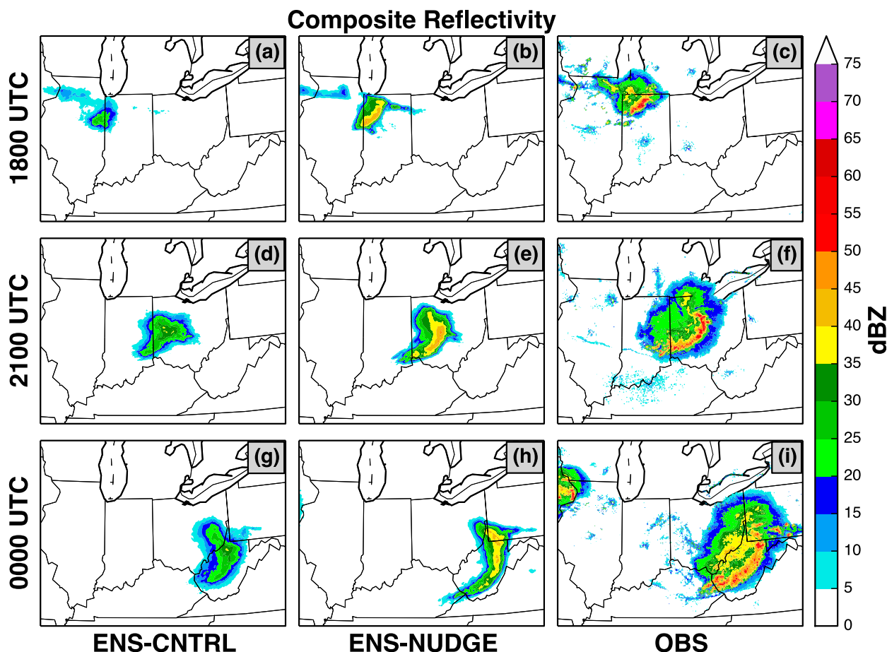
FIG. 11. As in Fig. 10, except results are displayed at 3-h intervals between 1800 UTC 29 Jun 2012 and 0000 UTC 30 Jun 2012. The central portion of the model domain is displayed.
