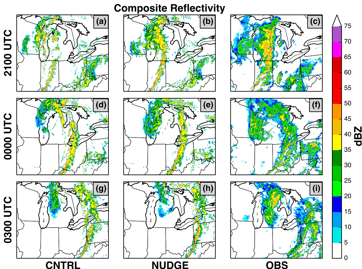
FIG. 19. As in Fig. 18, except results are displayed at 3-h intervals between 2100 UTC 17 Nov 2013 and 0300 UTC 18 Nov 2013. The north-central portion of the model domain is displayed.
