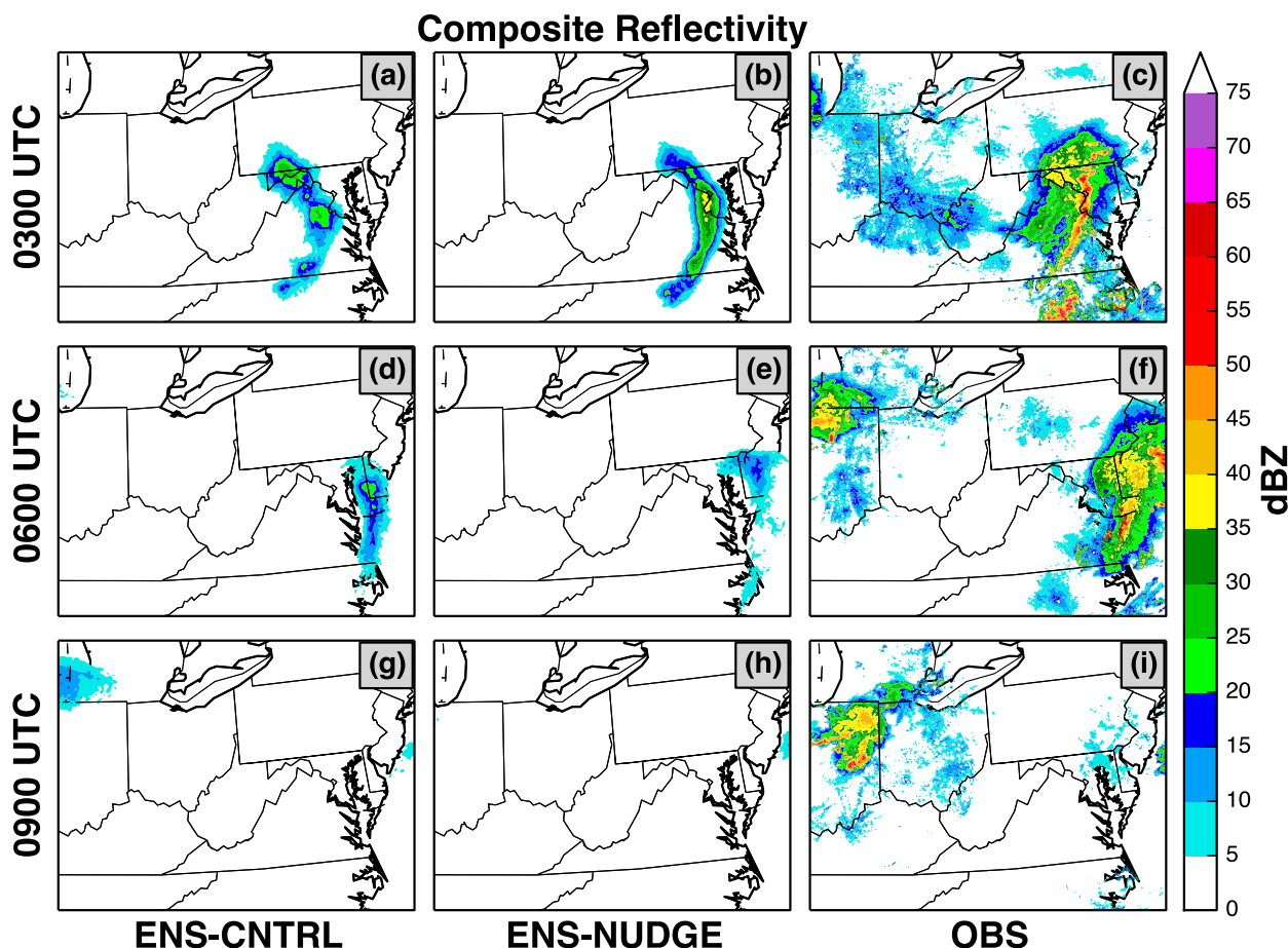
FIG. 12. As in Fig. 10, except results are displayed at 3-h intervals between 0300 UTC 30 Jun 2012 and 0900 UTC 30 Jun 2012. The central portion of the model domain is displayed.
