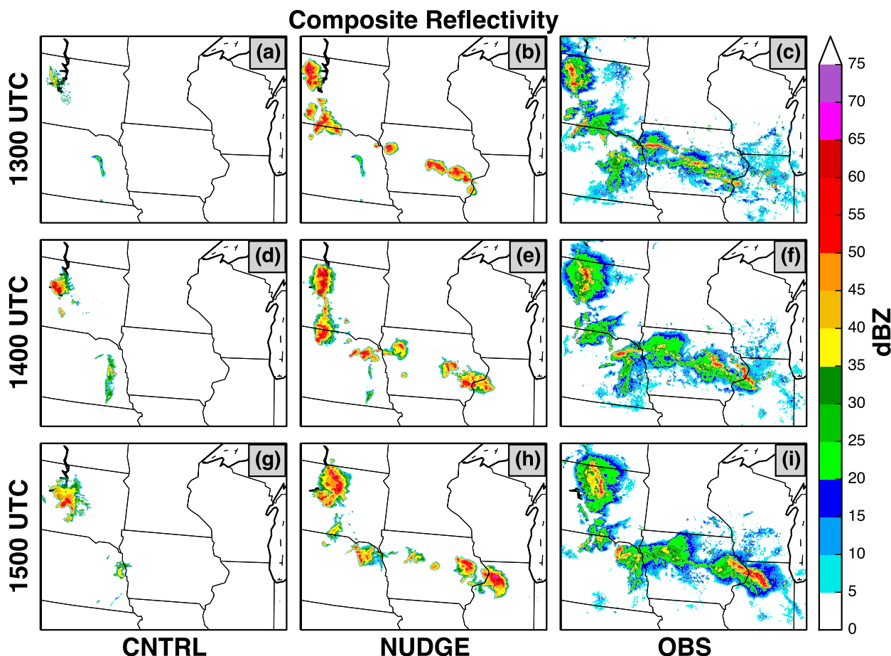
FIG. 4. Simulated and observed composite reflectivity for the first three hours of the deterministic simulations of the 29 Jun 2012 event (1300–1500 UTC 29 Jun 2012) for (a),(d),(g) CNTRL, (b),(e),(h) NUDGE, and (c),(f),(i) observations. The northwest portion of the model domain is displayed.
