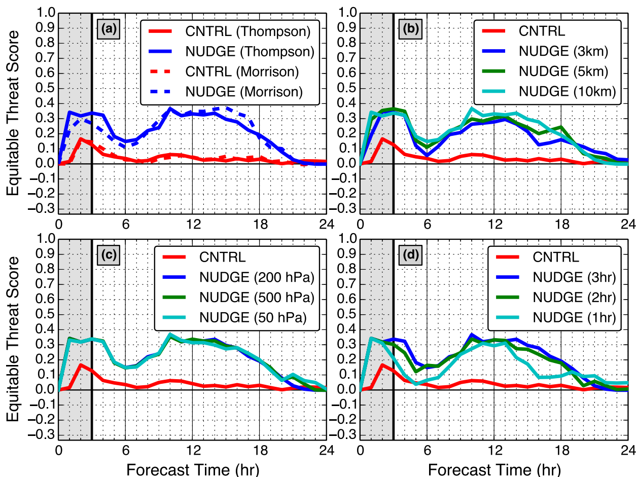
FIG. 8. ETS for precipitation \geq 1 mm for both the control and nudged simulations of the 29 Jun 2012 event, using (a) either Thompson or Morrison microphysics, for various (b) nudging radii, and differing (c) vertical nudging extents and (d) nudging periods. The vertical gray shaded area indicates times of moisture nudging in the NUDGE simulations.
