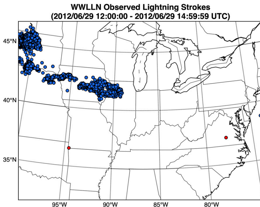
FIG. 2. Lightning strikes observed by WWLLN between 1200 and 1500 UTC 29 Jun 2012 over the WRF domain described in section 2c. Location data from 4315 lightning strikes were assimilated in the NUDGE and ENS-NUDGE experiments (blue dots). Two lightning strikes were removed by the filtering technique described in section 2a (red dots).
