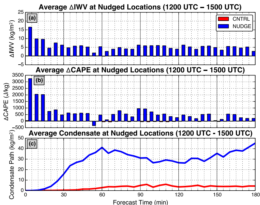
FIG. 3. Average temporal changes in (a) IWV and (b) CAPE at grid points where nudging is performed in NUDGE for the deterministic simulation of the 29 Jun 2012 event. (c) Average column condensate (liquid and solid water path) at nudged locations. Red bars (barely visible) and lines represent results from CNTRL, while blue bars and lines represent results from NUDGE.
