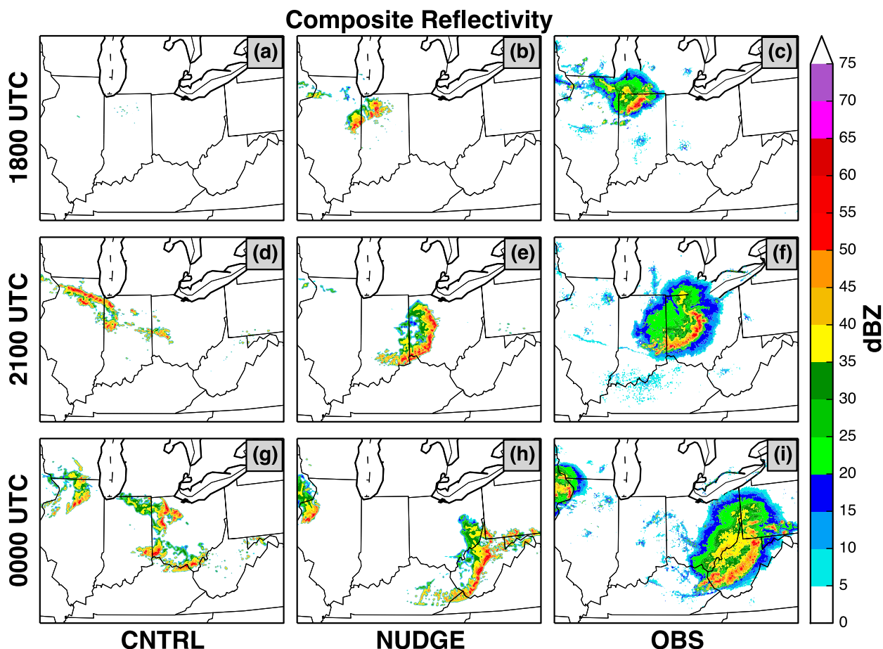
FIG. 6. As in Fig. 4, except results are displayed at 3-h intervals between 1800 UTC 29 Jun and 0000 UTC 30 Jun 2012. The central portion of the model domain is displayed.
