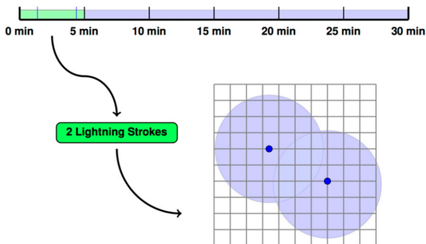
FIG. 1. A schematic of the lightning nudging process. (top) A timeline during a portion of the simulation, divided into 5-min bins. The green highlighting indicates the temporal bin containing the current time step, with blue lines representing observed lightning strikes. (bottom) An example of how the lightning strike locations (blue dots) are used to determine which grid points are nudged on the model domain (points within light blue circles) when the current simulation time step is within the green-highlighted bin.
