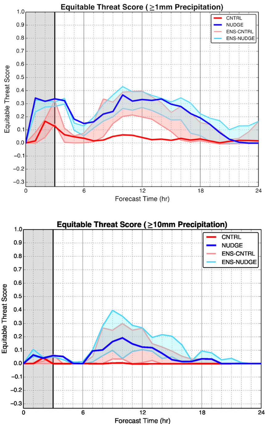
FIG. 14. Time series of ETS for CNTRL (thick red line), NUDGE (thick blue line), ENS-CNTRL (light red shaded region), and ENS-NUDGE (light blue shaded region) for the 29 Jun 2012 event for (top) \geq 1 and (bottom) \geq 10 mm over the previous hour. The vertical gray shaded area indicates times of moisture nudging in the NUDGE and ENS-NUDGE simulations.
