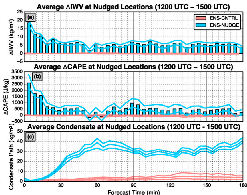
FIG. 15. Average temporal changes in (a) IWV and (b) CAPE at grid points where nudging is performed in ENS-NUDGE for the ensemble simulations of the 29 Jun 2012 event. (c) Average column condensate (liquid and solid water path) at nudged locations. Red bars (barely visible) and lines represent ensemble mean and range from ENS-CNTRL, while blue bars and lines represent ensemble mean and range from ENS-NUDGE.
