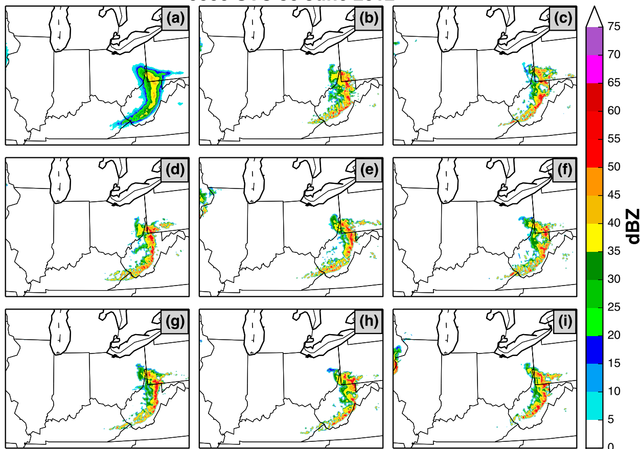
FIG. 13. Composite reflectivity from ENS-NUDGE at 0000 UTC 30 Jun 2012. (a) Ensemble-mean, and ensemble members (b) 1, (c) 6, (d) 11, (e) 16, (f) 21, (g) 26, (h) 31, and (i) 36. The central portion of the model domain is displayed.
