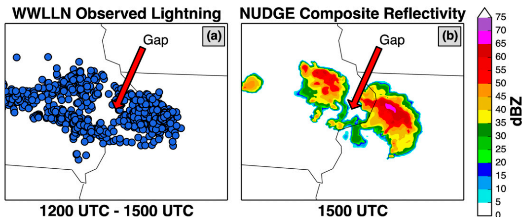
FIG. 5. (a) Lightning strikes observed by WWLLN between 1200 and 1500 UTC over eastern Iowa and western Illinois. (b) Simulated composite reflectivity in NUDGE over the same region at 1500 UTC (at the end of the 3-h nudging period). The red arrow indicates an area location with a lack of WWLLN-observed lightning strikes.
