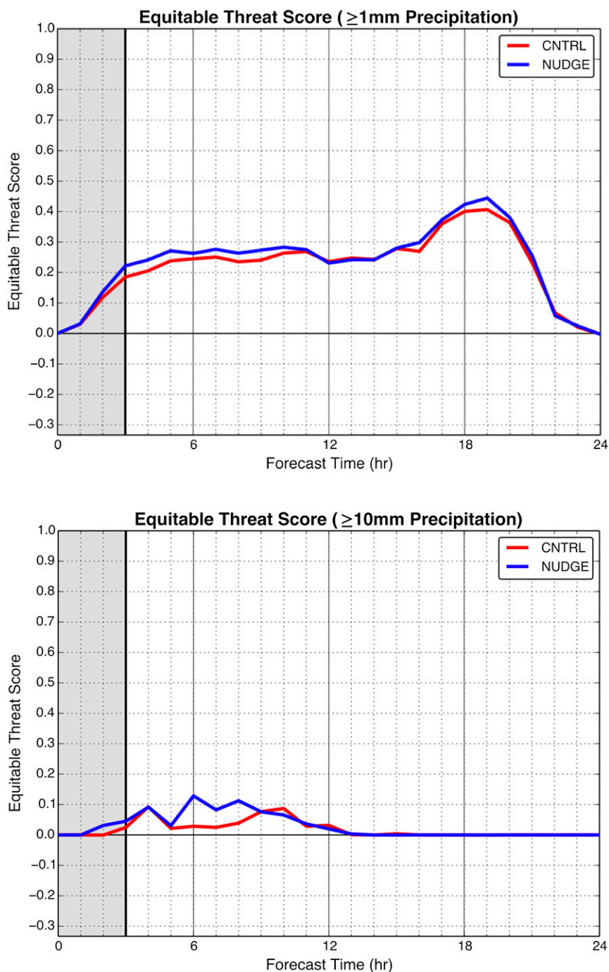
FIG. 20. Time series of ETS for CNTRL (thick red line) and NUDGE (thick blue line) for the 17 Nov 2013 event for both (top) 1- and (bottom) 10-mm thresholds. The vertical gray shaded area indicates times during which moisture nudging occurred in the NUDGE simulations.
