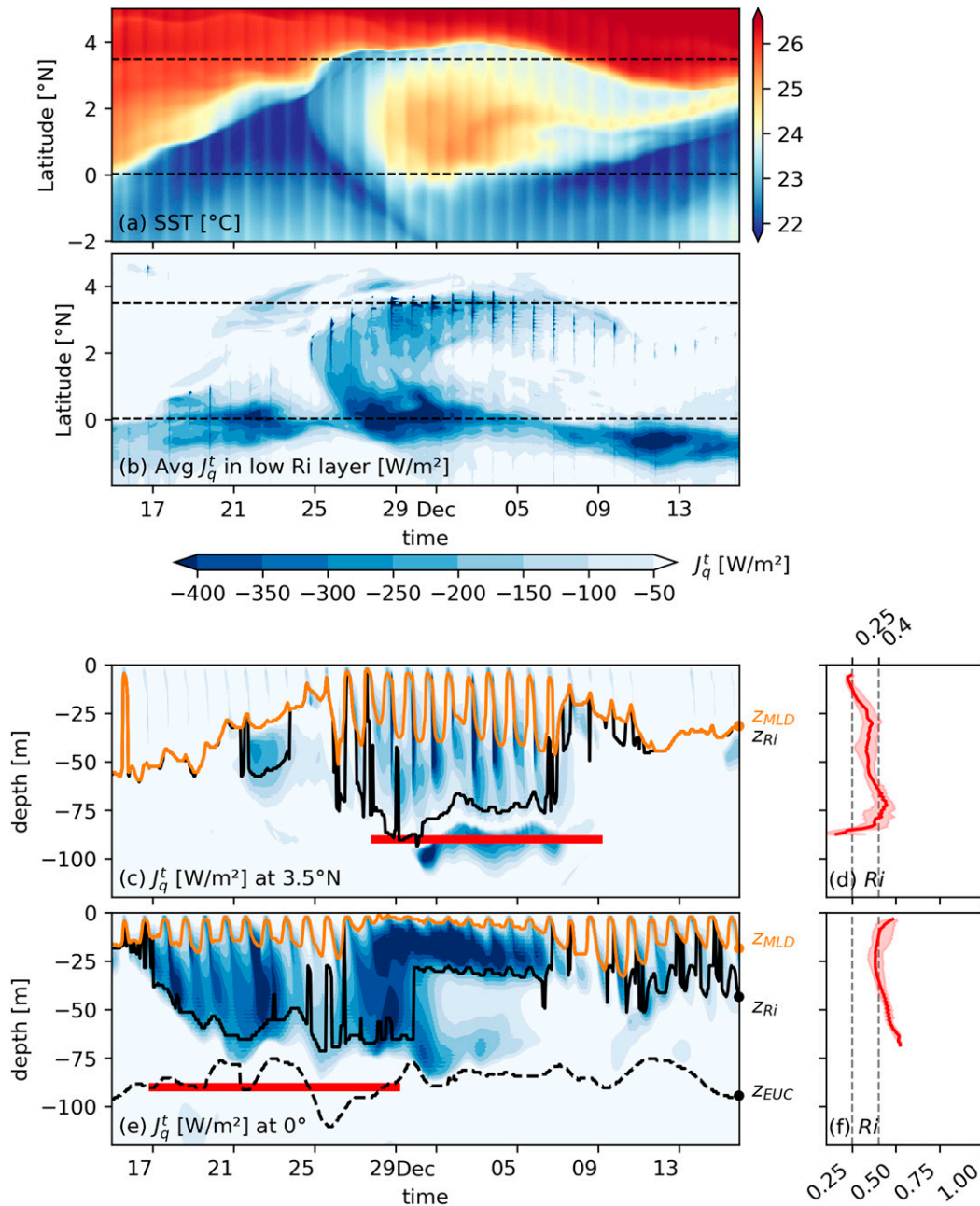
FIG. 4. Deep-cycle turbulence at the equator and 3.5°N. (a),(b) Time–latitude plots of (a) SST and (b) KPP heat flux J_q^t . (c),(e) Time–depth plots of KPP heat flux J_q^t . (d),(f) Median (solid line) and interquartile range (shading) of Ri in the low Ri layer z_{Ri} \leq z < z_{MLD} for the time period marked by red horizontal lines in (c) and (e), respectively. Dashed vertical lines in (d) and (f) mark Ri = 0.25 and Ri = 0.4 . Also shown are the mixed layer depth z_{MLD} (orange line), the depth of the base of the low Ri layer z_{Ri} (solid black line), and the depth of the EUC maximum z_{EUC} (dashed black line).
