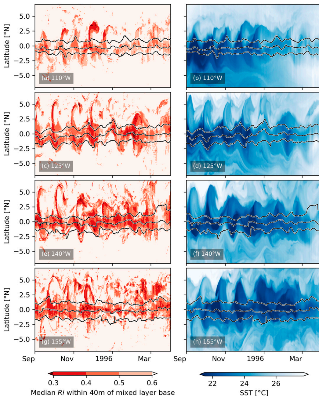
FIG. 3. Low Ri seen in the off-equatorial region at (a) 110°, (c) 125°, (e) 140°, and (g) 155°W between September 1995 and March 1996. (b), (d), (f), (h) Median Ri in the region z_{\text{MLD}} - 40 \leq z \leq z_{\text{MLD}} daily averaged SST illustrating TIW activity. Black lines on all panels show the EUC maximum and its latitudinal extent defined using the latitudes north and south of the core at which the eastward velocity drops by a factor of 2. The latitudes are determined using u at the depth of maximum eastward velocity.
