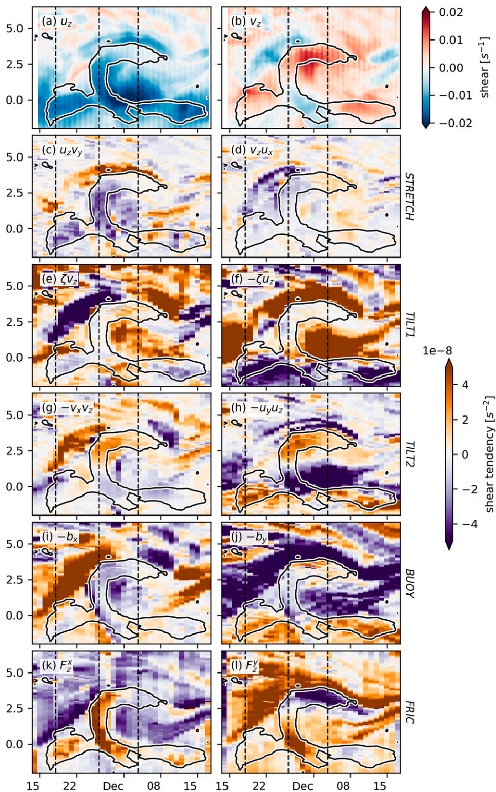
FIG. 9. Terms controlling the evolution of (left) u_z [Eq. (6)] and (right) v_z [Eq. (7)]. All quantities are depth-averaged in the top 60 m. Black contours mark low Ri layer thickness of 30 m for reference. Vertical lines mark the same time stamps as those in Fig. 7.
