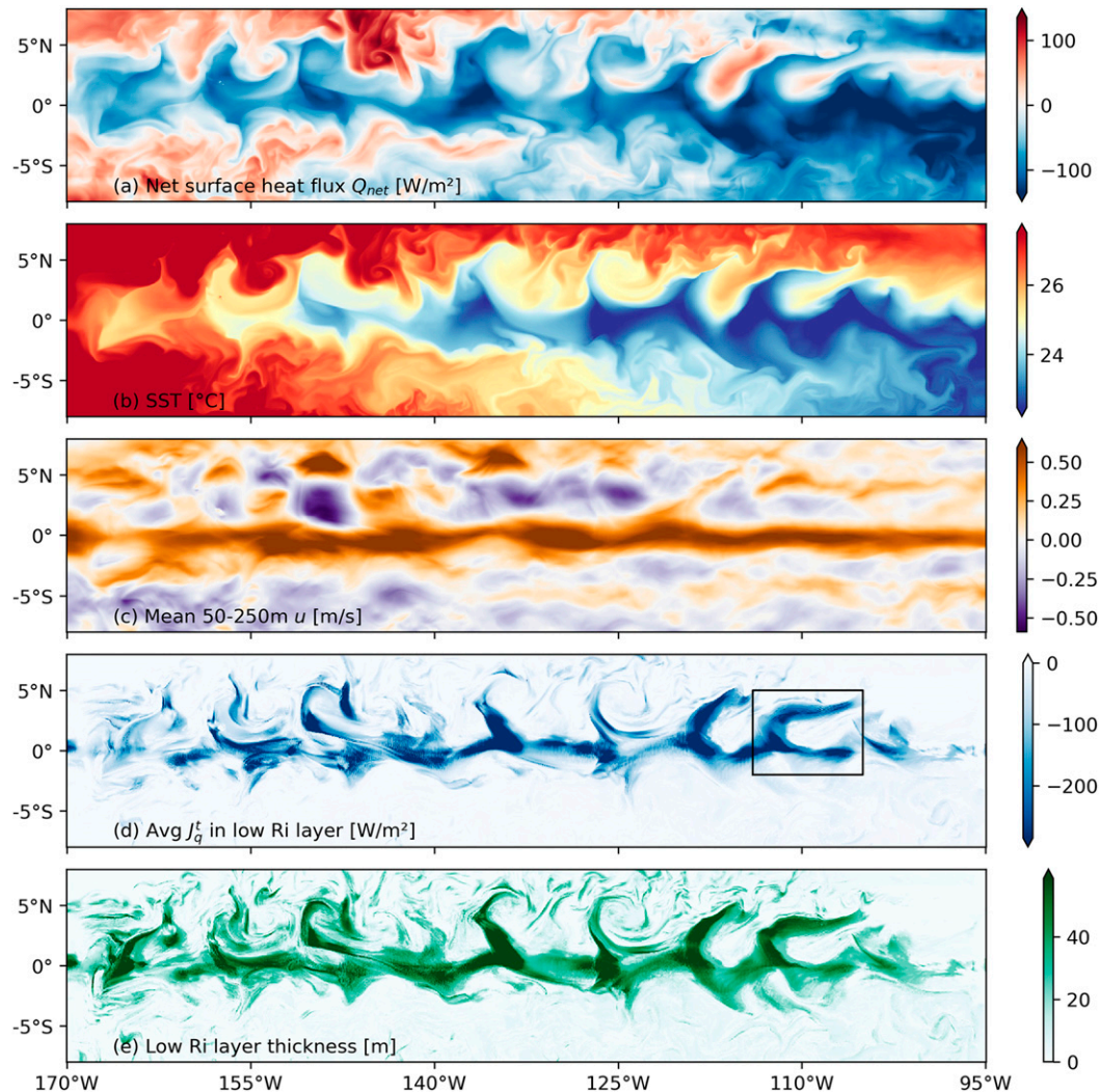
FIG. 2. Daily averaged fields for 5 Dec 1995. (a) Net surface heat flux Q_{\text{net}} (negative means heat enters the ocean). (b) SST. (c) Mean zonal velocity between 50 and 250 m. (d) Integrated turbulent heat flux in the low Ri layer ( z_{\text{Ri}} \leq Z < z_{\text{MLD}} ) normalized by a depth of 50 m. (e) Thickness of the low Ri layer ( z_{\text{MLD}} - z_{\text{Ri}} ). The black rectangle in (d) marks the TIW that is studied in detail later in this paper (e.g., Fig. 4).
