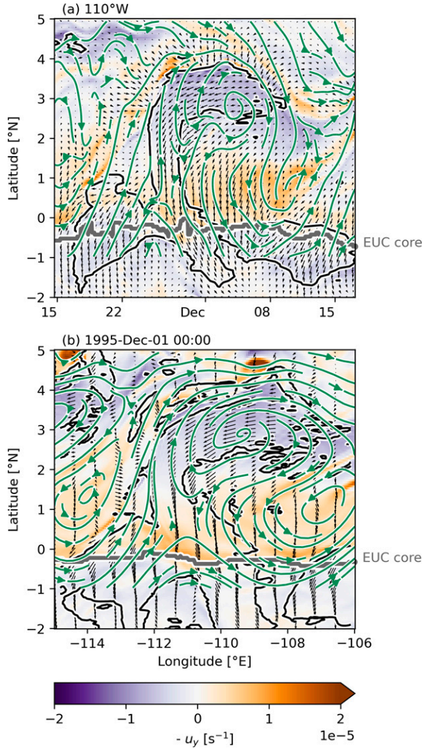
FIG. 8. Depth-averaged horizontal vorticity vectors \omega^x\hat{i} + \omega^y\hat{j} = (w_y - v_z)\hat{i} + (u_z - w_x)\hat{j} (black vectors) over depth-averaged -u_y (color). Streamlines, in green, are calculated using depth-averaged horizontal velocities with a TIW westward translation speed of 0.5 \text{ m s}^{-1} removed. All quantities are depth averaged to 60 m. Black contour indicates where the low Ri layer is 30 m thick. The latitude of the EUC core (defined as maximum u averaged between 30 and 120 m) is marked in gray. The horizontal vorticity vector rotates as parcels travel northward from the equator and then eastward. These quantities are presented in (a) time–latitude space at 110^\circ\text{W} , time in local time; (b) longitude–latitude space at 0000 UTC 1 Dec 1995.
