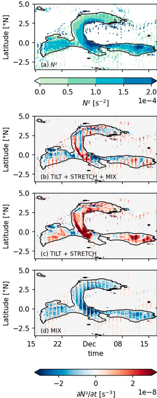
FIG. 10. Time–latitude plots of (a) N^2 , and (b)–(d) the stretching, tilting, and mixing terms that contribute to DN^2/Dt [from Eq. (9)] within the low Ri layer. The low Ri layer thickness is larger than 30 m within the black contour.
