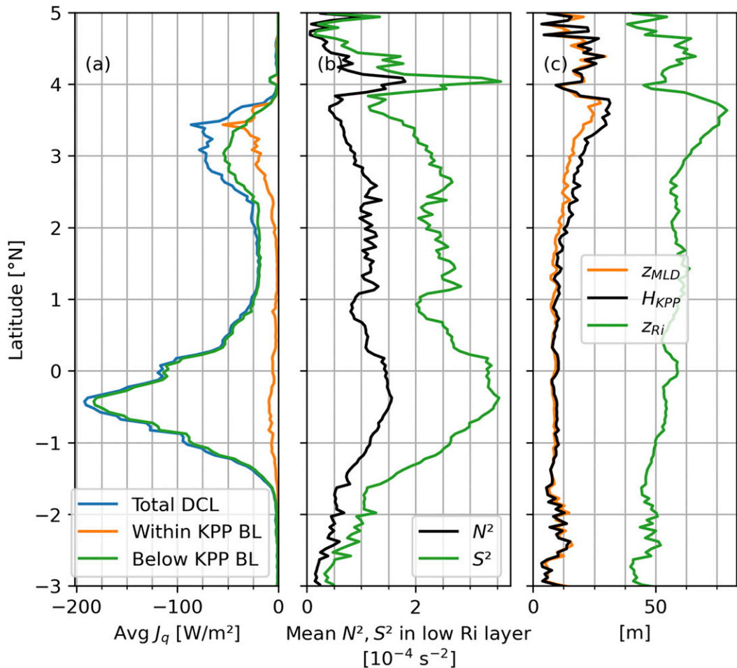
FIG. 12. Meridional profiles of quantities averaged within the low Ri layer at 110°W during the duration of the TIW. (a) J_q averaged over time and depth. (b) Mean N^2 , S^2 within the low Ri layer. The mean is taken over time and depth axes. (c) Time-mean z_{MLD} , H_{KPP} , and z_{Ri} over the period when the deep cycle is active.
