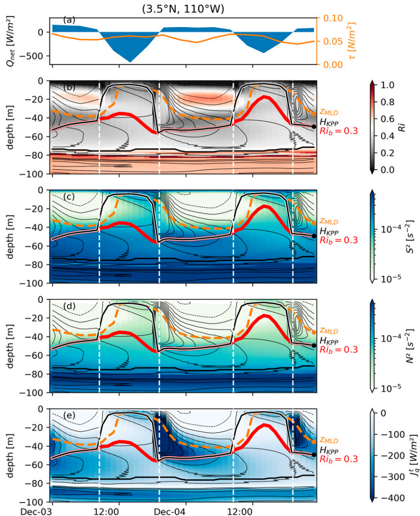
FIG. 11. Turbulence at 3.5°N, 110°W triggered by deepening of the boundary layer in the afternoon. (a) Surface forcing with net surface heat flux in blue and wind stress in orange. (b) Gradient Ri , (c) S^2 , (d) N^2 , and (e) turbulent heat flux J_q^t . Panels (b)–(e) also show the turbulent heat flux J_q^t (black contours; solid lines are negative, dashed are positive), the mixed layer depth ( z_{MLD} , orange dashed line), the KPP boundary layer depth (black line), and the depth at which the bulk Ri_b reaches 0.3 ( H_{0.3} , red line). Vertical white dashed lines mark time at which net surface heat flux changes sign.
