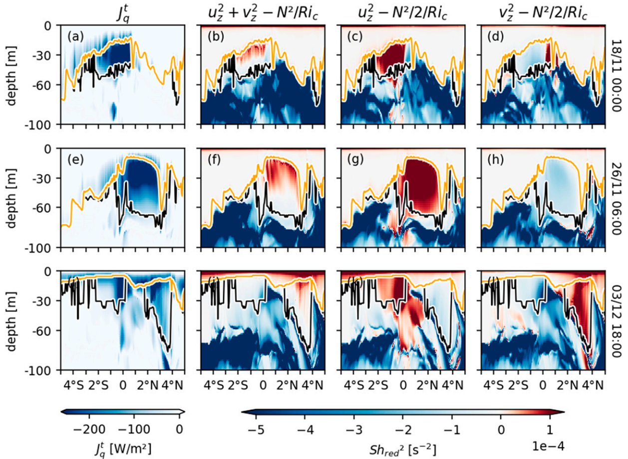
FIG. 7. Zonal shear drives enhanced equatorial turbulence while meridional shear drives enhanced off-equatorial turbulence. In both cases, the turbulence is in the low Ri layer. (a),(e),(i) Turbulent heat flux J_q^t ; (b),(f),(j) reduced shear Sh_{red}^2 ; (c),(g),(k) zonal shear contribution to Sh_{red}^2 ; and (d),(h),(l) meridional shear contribution to Sh_{red}^2 [see Eq. (5)]. All terms are plotted as a function of depth and latitude at three different time instants: (top) prior to the arrival of the cold cusp, (middle) when the cold cusp is oriented northward, and (bottom) when the cold cusp extends eastward. The time instants are labeled on the right of each row here and are marked by vertical lines in Fig. 6; z_{MLD} and z_{RL} are marked by orange and black lines, respectively.
