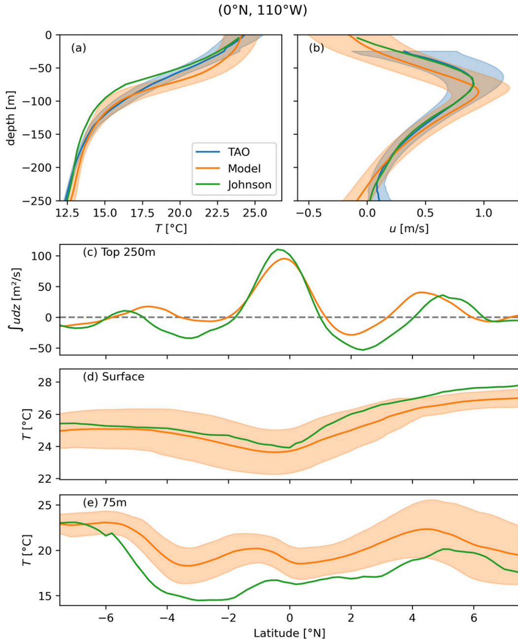
FIG. 1. Comparisons between modeled and observed zonal velocity and temperature at 110°W. (a),(b) Annual mean fields (solid line) and standard deviation of daily means over a year (shaded) for three datasets: the model during 1996 (orange), a climatological annual cycle constructed from the TAO dataset between 1990 and 2000 (blue), and the Johnson et al. (2002) climatology (green, no standard deviation available). (c) Vertically integrated zonal velocity in the top 250 m from the model and the Johnson dataset. Meridional section of temperature at (d) the surface and (e) 75 m.
