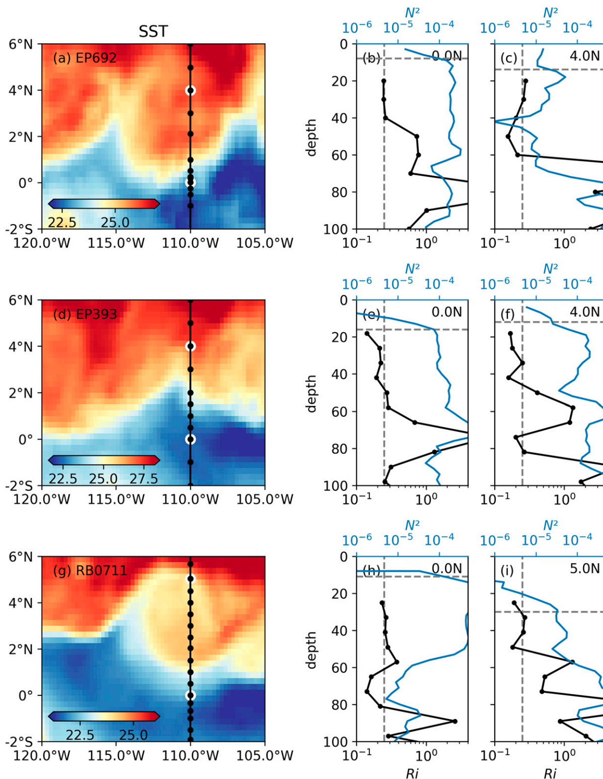
FIG. 13. Indirect evidence for an off-equatorial deep cycle from three cruise transects (Table 1). (a),(d),(g) SST from the daily 0.25° OISST product (Reynolds et al. 2007) with CTD stations marked (note changing color scale). (b),(c),(e),(f),(h),(i) Profiles of Ri (black) and N^2 (blue) at stations marked with white circles in (a), (d), and (g). The vertical line is Ri = 0.25 , and the horizontal line is mixed layer depth estimated as the shallowest depth at which the potential density exceeds the shallowest recorded density value by 0.015 \text{ kg m}^{-3} .
