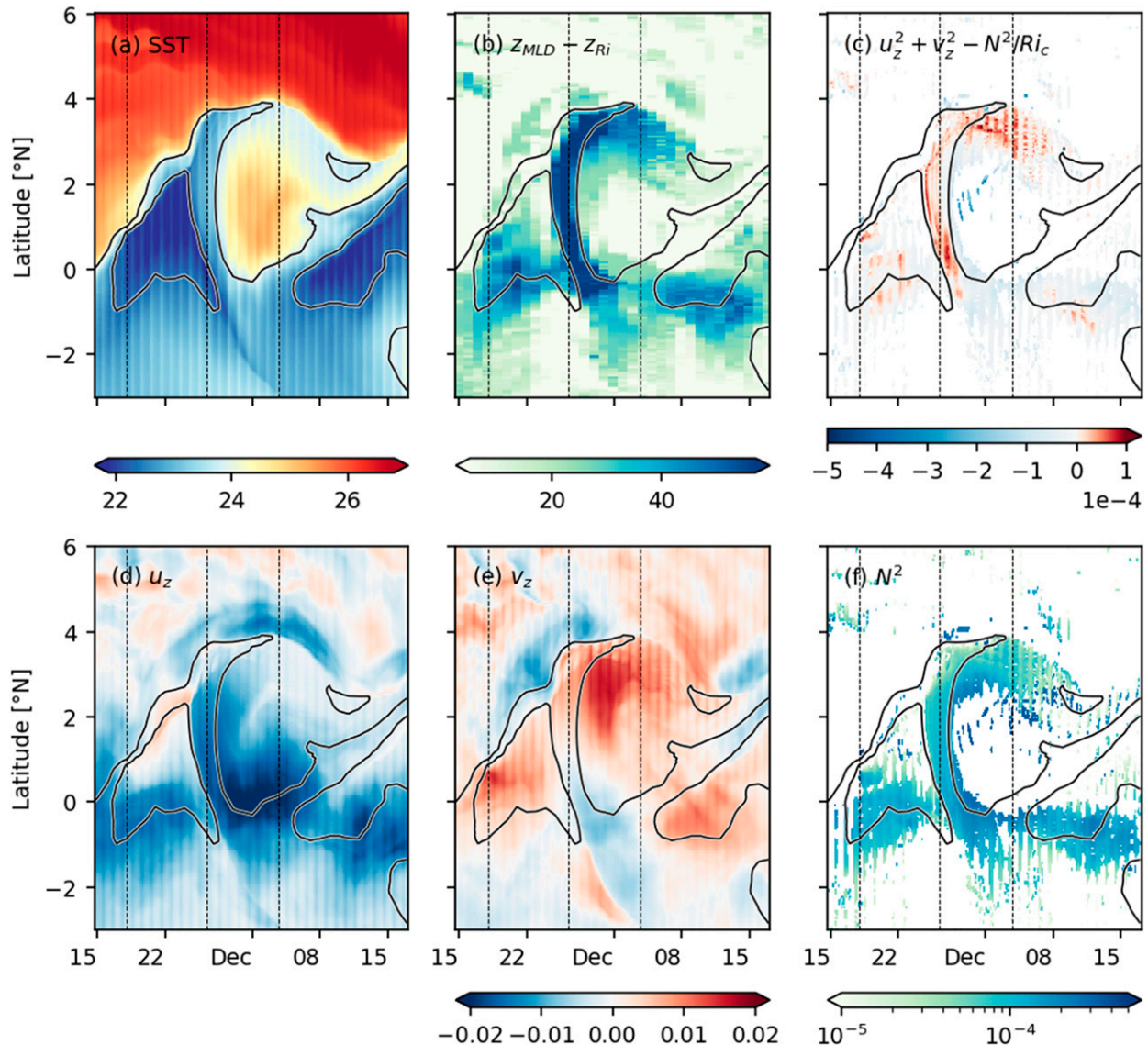
FIG. 6. Time–latitude plots of (a) SST, (b) low Ri layer thickness, (c) median Sh_{red}^2 within the low Ri layer (same color bar as in Fig. 7), (d) mean u_z in the top 60 m, (e) mean v_z in the top 60 m, and (f) mean N^2 within the low Ri layer for one TIW. Vertical lines mark time instants presented in Fig. 7. The black contours mark SSTs of 22.4° and 23.5°C.
