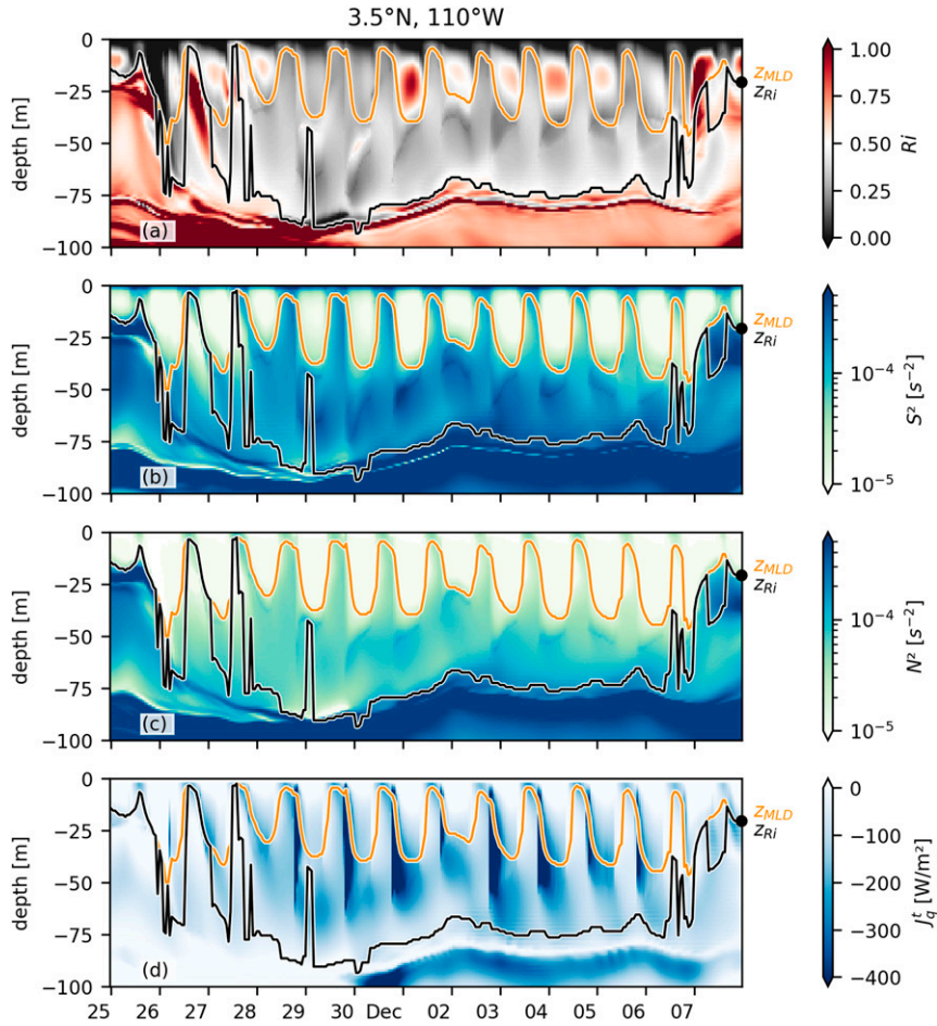
FIG. 5. Daily cycles in (a) Ri , (b) squared shear S^2 , (c) buoyancy frequency N^2 , and (d) J_q^t at 3.5^\circ\text{N} . This time period is a subset of the time period shown in Fig. 4. Also shown are the mixed layer depth z_{\text{MLD}} (orange line) and the depth of the base of the low Ri layer z_{\text{Ri}} (black line).
