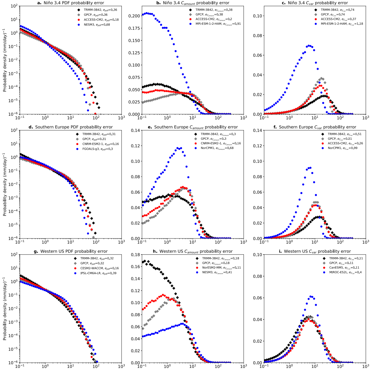
FIG. 7. Best (red) and lowest (blue) performing models under (left) probability error metrics for the PDF ( e_{pdf} ), (center) contribution to precipitation amount C_{amount} ( e_{C_{amount}} ), and (right) contribution to variance ( e_{C_{var}} ) in three different regions: (a)–(c) the Niño-3.4 region (5°S–5°N, 190°–240°E), (d)–(f) southern Europe (40°–50°N, 0°–20°E), and (g)–(i) the western United States (30°–48°N, 236°–257°E). Comparison is against GPCP (gray) and TRMM-3B42 (black).
