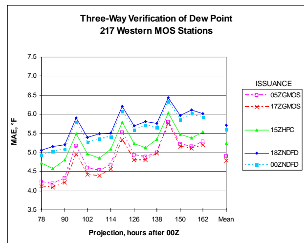
Figure 2. MAE of maximum temperature (a,b), minimum temperature (c,d), and dew point (e,f), at non-MOS and MOS observation sites. The mean of all projections is shown at far right.
