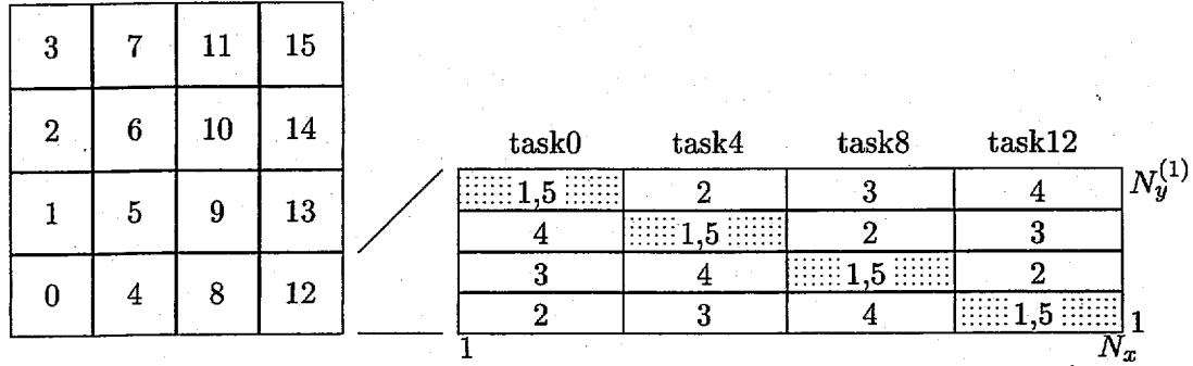
Figure 11. Same as Fig.10 but for the forward sweep in the case of Method 2 when, effectively, Q = 0 . Each task sweeps its own four-partitioned subregion once except for the repetition in each stripe where sweeping is initiated (dotted region marked by '1,5'). For the corresponding backward sweep, the initiation stripes are also staggered, but lie diagonally but in the opposite orientation to ensure proper alignment and ordering of the sequence-numbered stripes.
