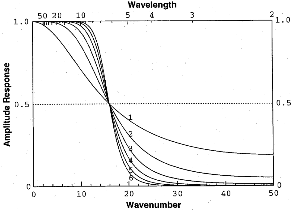
Figure 4. The amplitude responses of sine-Butterworth filters with different orders but the same critical wavenumber of 16.
