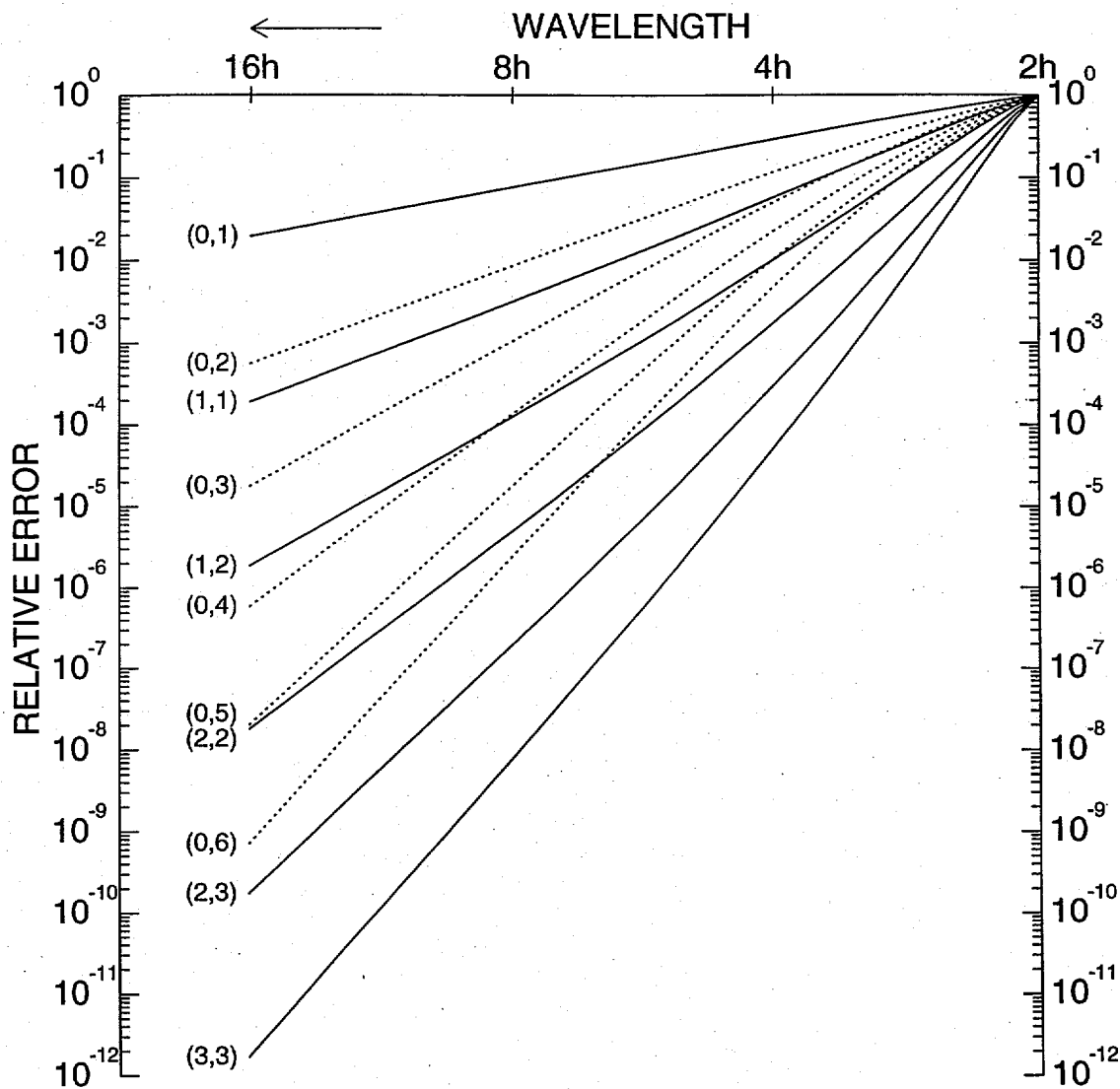
Figure 3. Same as Figure 1 but for the midpoint interpolation stencil.
