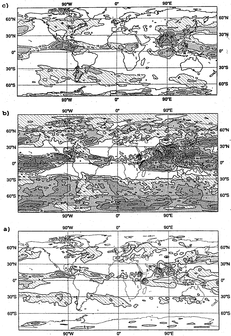
FIG. 2. As Fig. 1 but cloud cover of high-level clouds: (a) model-produced effective cloud cover; (b) model-produced real cloud cover; and (c) observed cloud cover from ISCCP.
