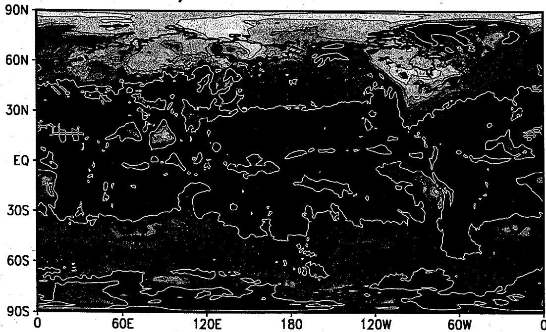
d) Nature run LCC
