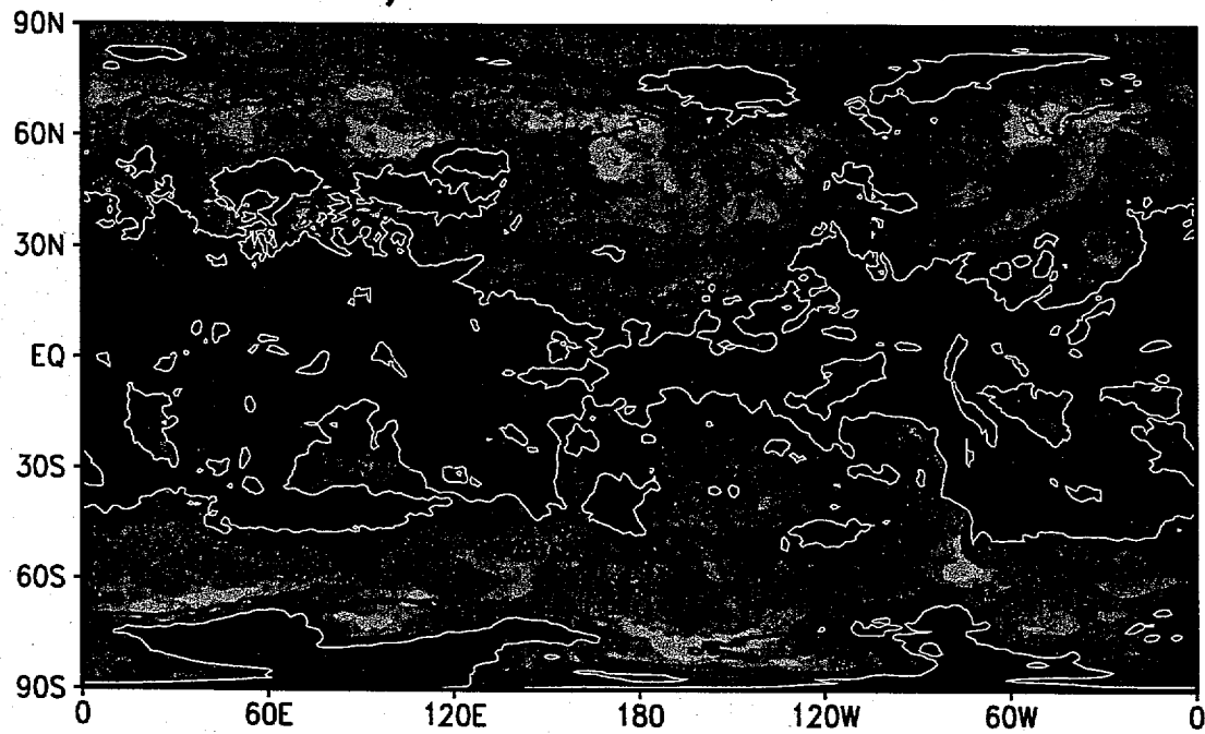
c) Nature run MCC
