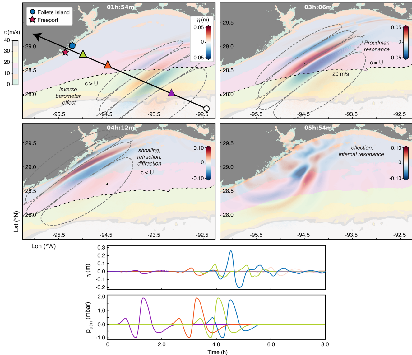
Figure 4. Overview of the model domain and processes responsible for meteotsunami generation, amplification, and propagation in the model, shown for the “early storm” air pressure disturbance p_{atm} (Figures 2e and 3b). The colored contours represent the shallow water wave celerity c = \sqrt{gh} in terms of the water depth h and the blue-red colormap the instantaneous sea-level anomaly \eta . The bold dashed contour line identifies the location of Proudman resonance—that is, when the speed of the air pressure disturbance U matches c —and maximum energy transfer (here, 21 m/s); the solid black line shows the path along which the disturbance travels (offshore to onshore); and the dashed gray lines indicate the spatial extent of the pressure disturbance. Time series at select offshore recording stations are also shown to illustrate wave transformation across the continental shelf.
