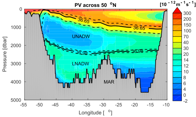
Figure 1. Identification of UNADW and LNADW in \sigma_2 space at 50^\circ\text{N} in FLAME. The upper bound of UNADW is denoted by \sigma_2^{\text{max}}(50^\circ\text{N}) , the time mean of which is 36.65 \text{ kg/m}^3 (solid black line), with a minimum/maximum of 36.47/36.80 \text{ kg/m}^3 (dashed lines). The lower bound of UNADW is denoted by the isopycnal of 36.98 \text{ kg/m}^3 , which is determined by the climatological PV field ( \leq 10 \times 10^{-12} \text{ m}^{-1} \cdot \text{s}^{-1} , shown in background color). The standard deviation of this lower bound, determined by annually varying low PV, is also shown as dashed lines, with a minimum of 36.97 \text{ kg/m}^3 and a maximum of 36.99 \text{ kg/m}^3 . Sensitivity tests show robust results using different choices of the separating isopycnals that lie within one standard deviation of the climatology. See Figures S2 and S3 for similar plots in ORCA and SODA. UNADW = Upper North Atlantic Deep Water; LNADW = the Lower North Atlantic Deep Water; PV = potential vorticity.
