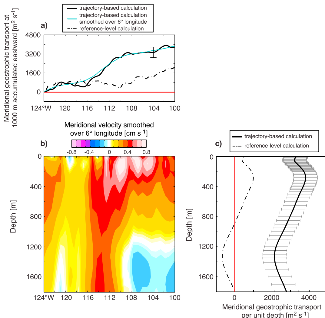
Figure 3. (a) Geostrophic transport at 1000 m averaged between 30°S and 42°S accumulated from 124°W eastward based on trajectories (solid black) and relative to 1800 m (dashed black). The error bar in black shows random error generated from heterogeneous trajectory density. The blue line shows geostrophic transport accumulated eastward based on geostrophic velocities smoothed using a 6° longitude running mean. (b) Meridional geostrophic velocity, based on geostrophic shear and trajectory-derived reference velocities, averaged between 30°S and 42°S. The geostrophic velocities are smoothed using a 6° longitude running mean for display purposes only. (c) Estimate of the meridional geostrophic transport per unit depth, computed using trajectory-based reference velocity with a correction for shear-induced error ( E_{\text{sys}} ), averaged between 30°S and 42°S, and integrated between 117°W and 108°W (solid black), and meridional geostrophic transport per unit depth relative to 1800 m (dashed black). The error bars in gray color show random errors generated from heterogeneous trajectory density.
