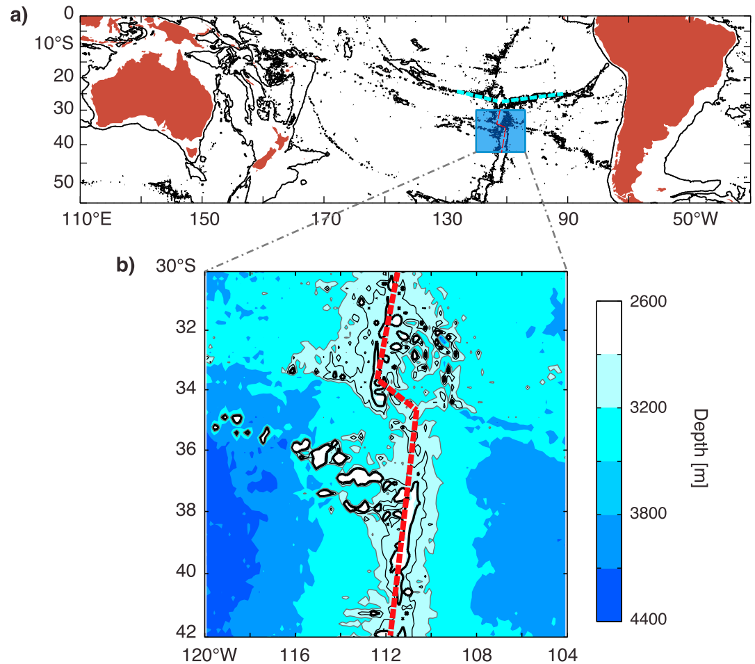
Figure 1. (a) The dark blue boxed region, 42°S to 30°S, 120°W to 104°W, indicates the location of the study area in the South Pacific Ocean. The black contours indicate 3000 m depth. The dashed red line indicates the EPR. The dashed blue line indicates the Easter Fracture Zone. (b) ETOPO2 2 min bathymetry over the EPR. The contour lines indicate 2600 m (thickest black), 2800 m (thin black), and 3000 m (thin gray) depth. The crest of the EPR is indicated in red.
