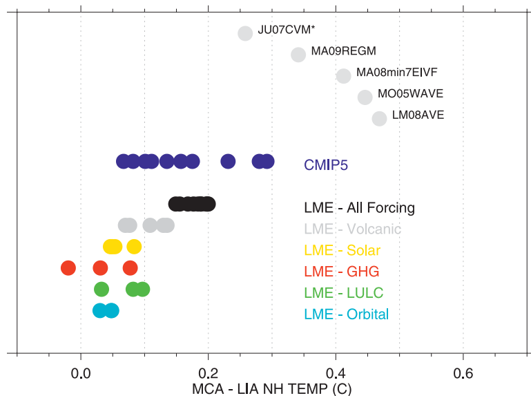
FIG. 5. NH annual surface temperature changes ( ^{\circ}\text{C} ), MCA (950–1250) minus LIA (1450–1850), for reconstructions plotted in Fig. 3, CMIP5 LM simulations, and each of the CESM-LME ensemble members.
