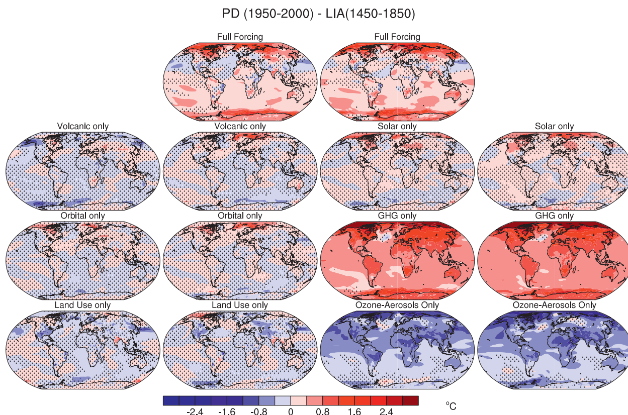
FIG. 8. Annual surface temperature anomalies ( ^{\circ}\text{C} ), PD (1950–2000) minus LIA (1450–1850), as simulated in CESM-LME. Shown for each forcing set are the ensemble members with (left) minimum and (right) maximum global average temperature differences. Stippling indicates differences not statistically significant at the 95% level using a Student's t test.
