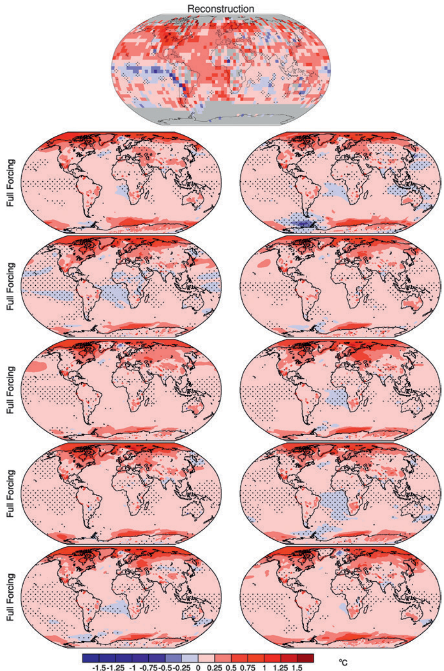
FIG. 4. Annual surface temperature changes ( ^{\circ}\text{C} ), MCA (950–1250) minus LIA (1450–1850), from Mann et al. (2009) proxy-based reconstruction are shown in the top panel and in the remaining panels the changes as simulated in the 10 CESM-LME full-forcing simulations. Stippling indicates differences not statistically significant at the 95% level using a Student's t test.
