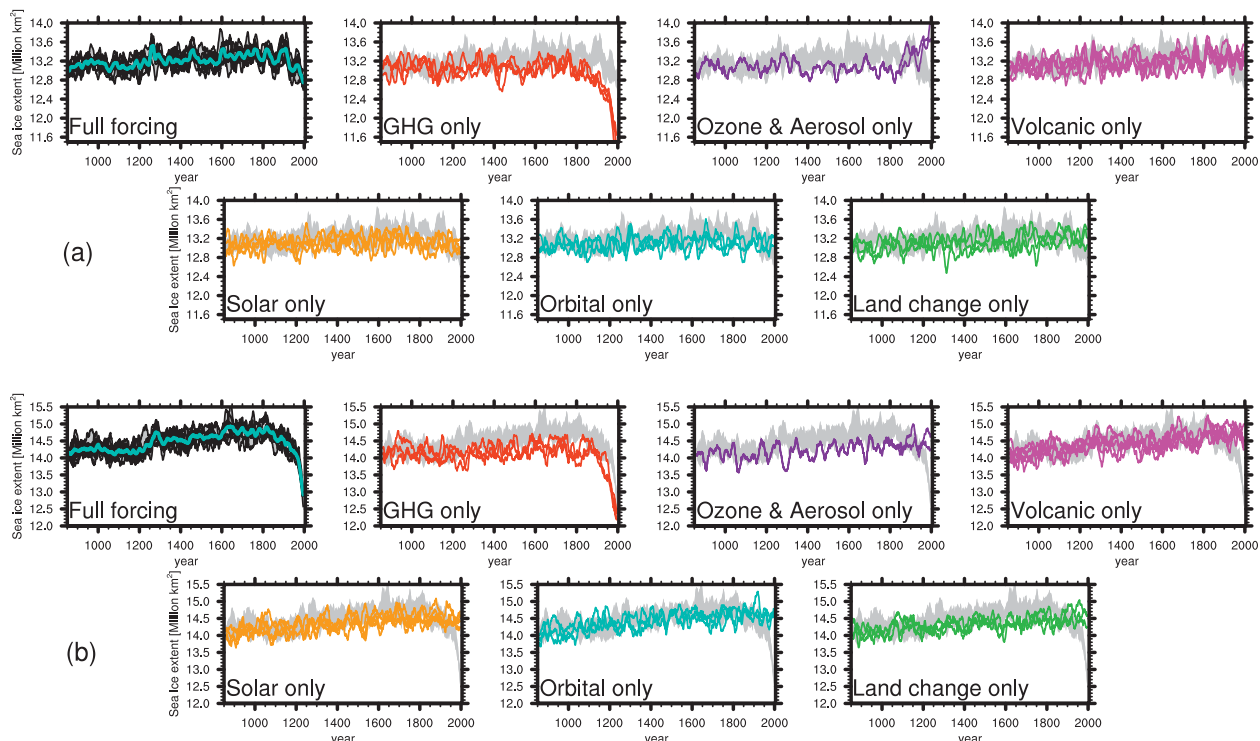
FIG. 9. Annual mean sea ice extent (million km 2 ) for the (a) Northern and (b) Southern Hemispheres in the CESM-LME single-forcing and the full-forcing ensemble simulations (smoothed with a 20-yr running mean). The ensemble spread in the full-forcing ensemble is shown by gray shading in all panels and the ensemble mean of the 10 fully forced ensemble members is shown in cyan in the full-forcing panels.
