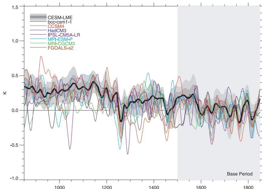
FIG. 6. Jun–Aug land surface temperature anomalies ( ^{\circ}\text{C} ) for Europe ( 35^{\circ}\text{--}70^{\circ}\text{N} , 5^{\circ}\text{W--}40^{\circ}\text{E} ) for the mean of the full-forcing runs (black) with 1\sigma (dark gray) and 2\sigma (light gray) ranges vs the CMIP5 LM simulations. Anomalies are computed relative to the base period of 1500–1850. A 20-yr Gaussian smoothing has been applied.
