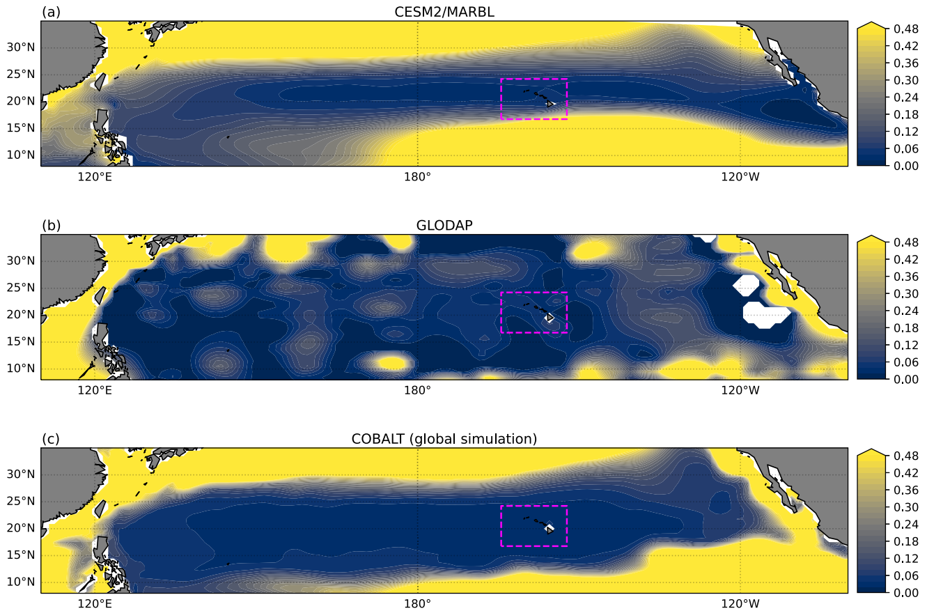
Figure 5. Comparison of time-averaged surface nitrate concentrations ( \mu\text{mol kg}^{-1} ): (a) CESM2/MARBL, (b) GLODAP, and (c) a global COBALT simulation. White areas in (b) indicate gaps in GLODAP nitrate data. Magenta rectangle indicates regional model domain. See text for details.
