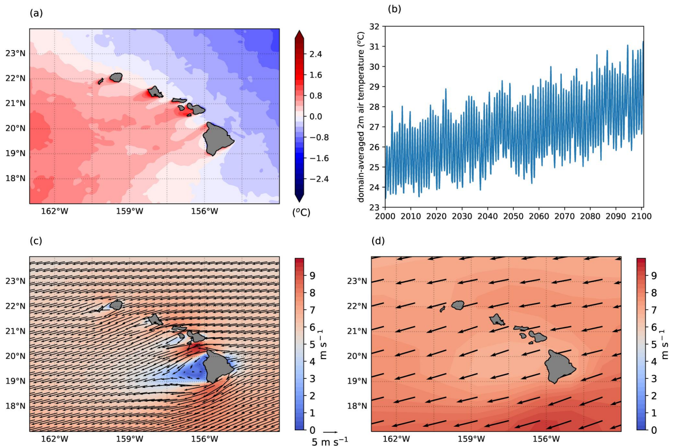
Figure 3. Atmospheric forcing components: (a): snapshot of climatological WRF 2 m air temperature anomaly for September 1 (°C). (b): Domain-averaged CESM2 2 m air temperature (°C) for LE2–1301.009 (SSP3–7.0). (c): Time-averaged (2000–2020) 10 m wind field ( \text{m s}^{-1} ) derived by the neural network. (d): Time-averaged (2000–2020) 10 m wind field ( \text{m s}^{-1} ) of CESM2. See text for details.
