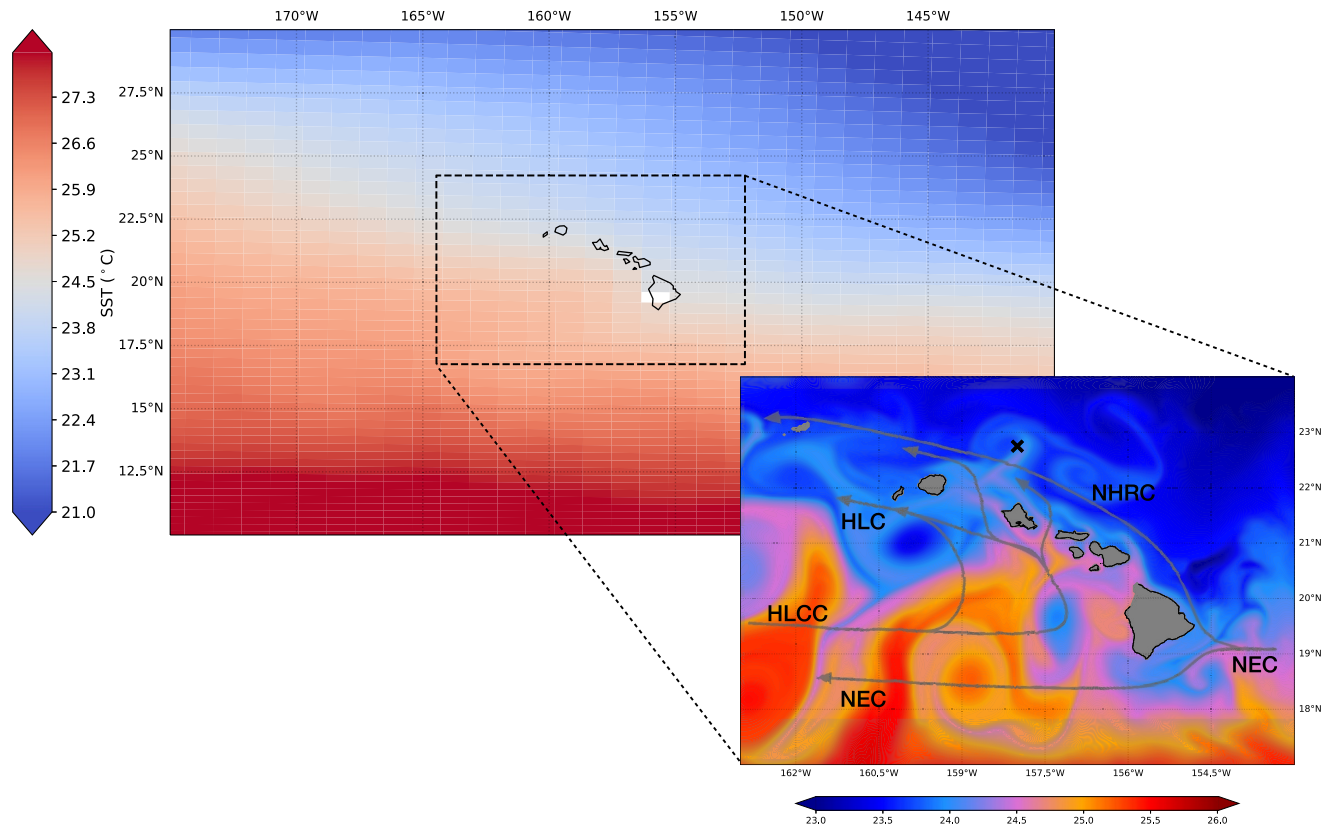
Figure 1. Domain of regional ROMS/COBALT model (dashed rectangular). A snapshot of monthly mean SST ( ^{\circ}\text{C} ) is shown for CESM2 (upper panel) and ROMS/COBALT (inlay) to illustrate the location of the model domain as well as different horizontal model resolutions. CESM2 does not represent the islands of Hawai'i, merely one rectangular island. The cross indicates the location of Station ALOHA. Arrows indicate a schematic map of the mean currents around Hawai'i. Please see text for details.
