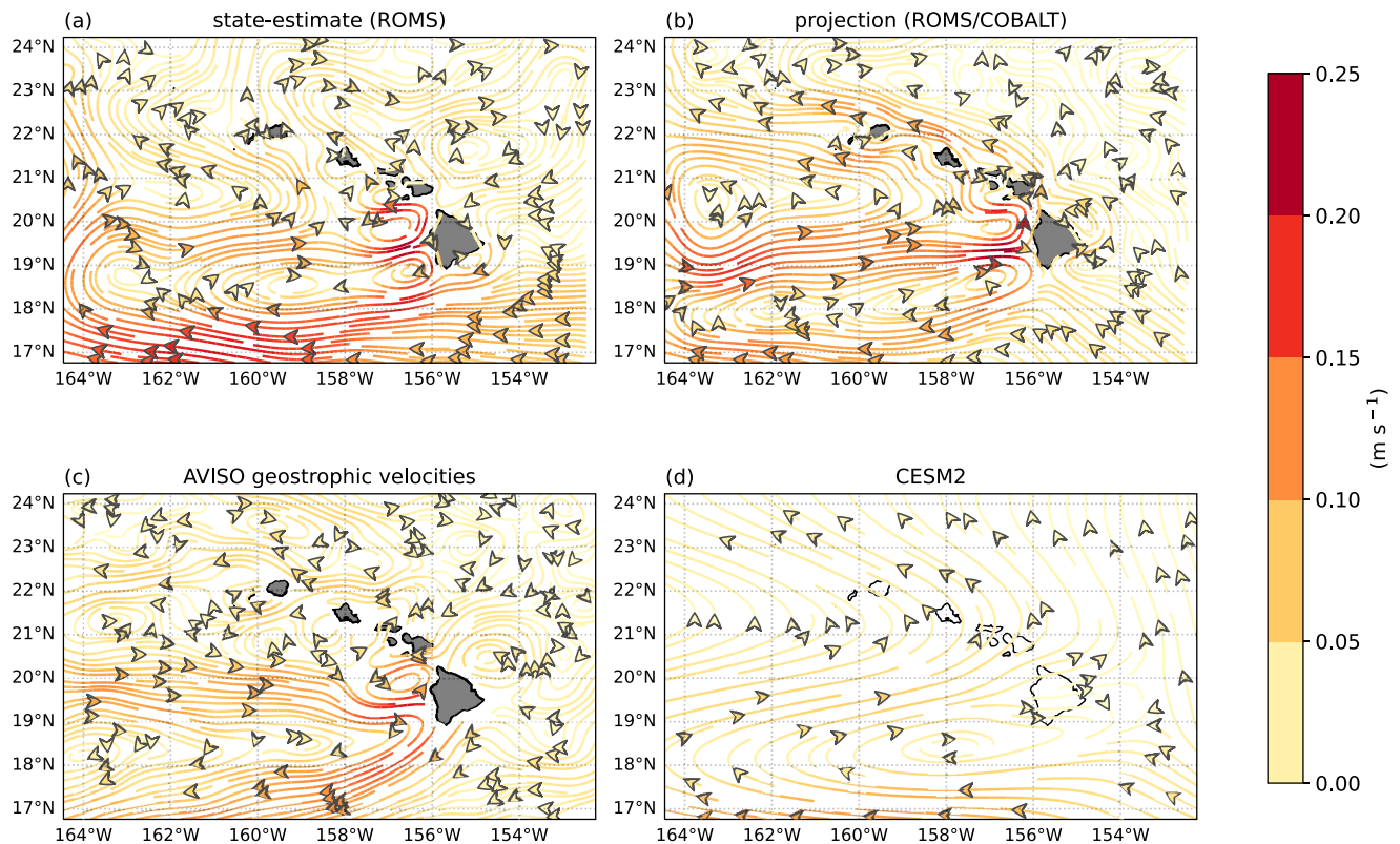
Figure 9. Comparison of time-averaged (years 2010–2020) upper ocean currents (0–100 m, \text{m s}^{-1} ) for (a) ROMS state estimate (Partridge et al., 2019), (b) ROMS/COBALT downscaled within CESM2, (c) AVISO geostrophic currents, and (d) CESM2 (LE2–1301.009).
