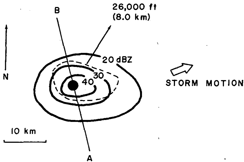
Figure 1b. Schematic composite of the same moderate thunderstorm as in Figure 1a, but as seen on a radar VPP PPI during a tilt sequence. Solid lines are the low-level reflectivity contours. Dashed line outlines the echo \geq 20 dBZ derived from the mid-level elevation scan. The black dot is the location of the maximum echo top from the high-level scan.
