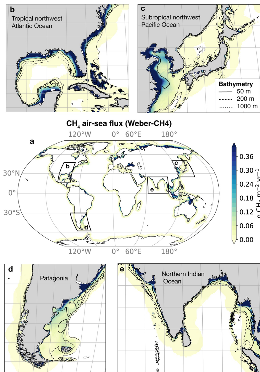
Figure 11. (a) Global maps of coastal \text{CH}_4 flux from the Weber-CH4 product (includes diffusive and ebullitive flux, in \text{g CH}_4 \text{ m}^{-2} \text{ year}^{-1} ); (b–e) insets show the \text{CH}_4 flux in four coastal regions along with 50, 200 and 1,000 m bathymetry contours. \text{CH}_4 emissions are most intense in shallow coastal environments.
