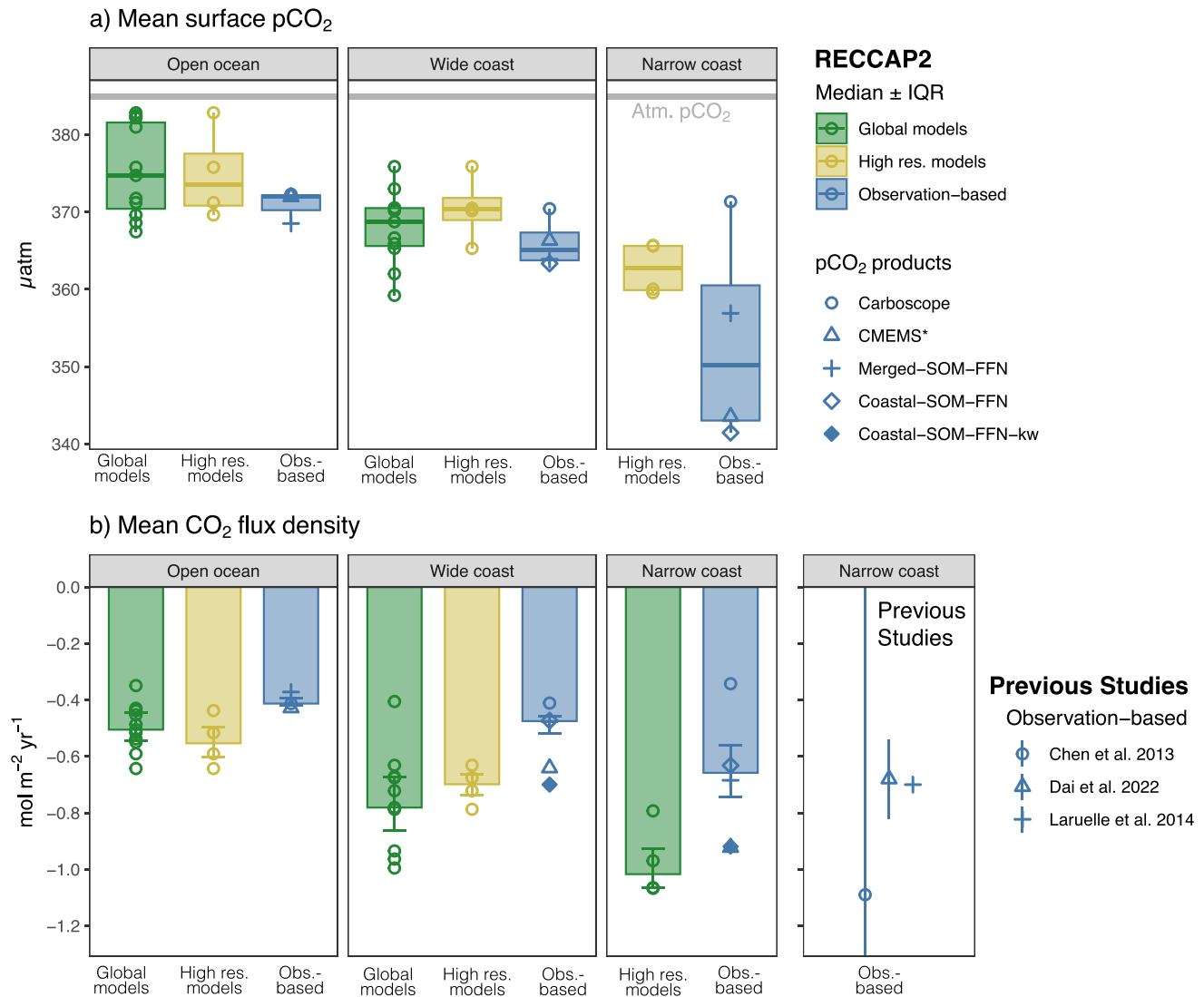
Figure 4. Comparison of globally-averaged (a) sea surface pCO 2 [μatm] and (b) flux density [mol C m 2 year -1 ] averaged over open ocean, wide coastal and narrow coastal ocean waters in pCO 2 -products and ocean models. Figure shows individual products and models (symbols) and their median and interquartile ranges. Models are shown for the full ensemble available (11 models) and a subset of higher resolution models (4 models, see Methods and Table 2 for details). Previous estimates available for the narrow coastal ocean are shown on the right of panel (b). Coastal-SOM-FFN-k w , which is a second version of Coastal-SOM-FFN computed using different wind speeds and k w formulation (filled diamond, see Methods), is not used in the calculation of the pCO 2 -product median.
