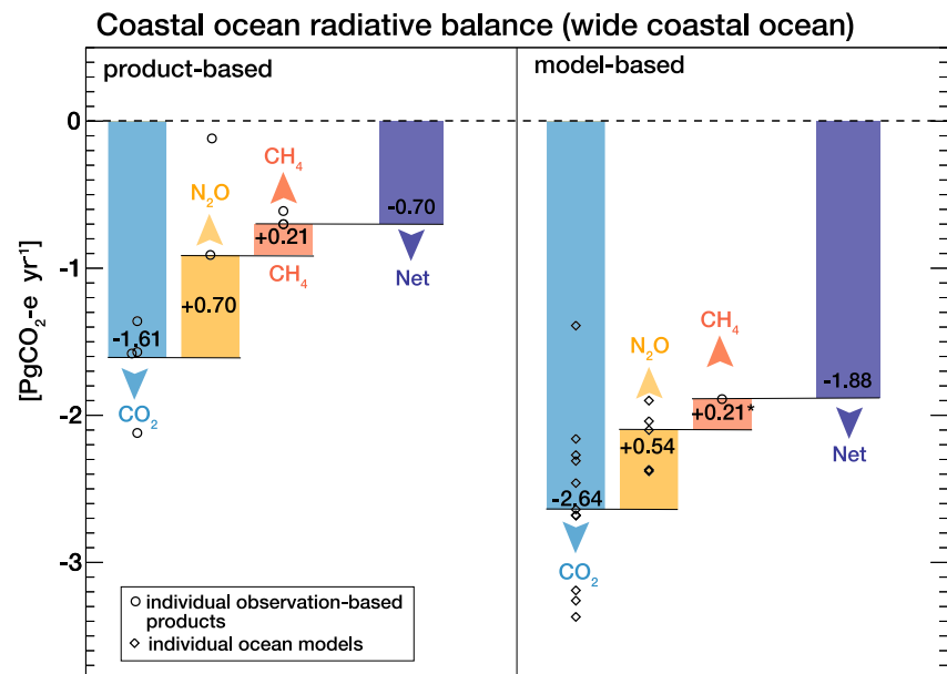
Figure 3. Wide coastal ocean atmospheric radiative balance (using \text{PgCO}_2\text{-e yr}^{-1} ) based on observational products and models of contemporary \text{CO}_2 , \text{N}_2\text{O} and \text{CH}_4 fluxes. Observation-based central values are from 4 \text{pCO}_2 -products, Yang-N2O and Weber-CH4. Model-based central values are from the 11 global models for \text{CO}_2 and 4 global models for \text{N}_2\text{O} , but the Weber-CH4 product is used for \text{CH}_4 as indicated by the asterisk (no model available for \text{CH}_4 , hence minimizing the difference between the two assessments). Individual models and observation-based product estimates are shown by symbols. The net greenhouse gas flux in \text{PgCO}_2\text{-e yr}^{-1} corresponds to the sum of the three gases' contributions.
