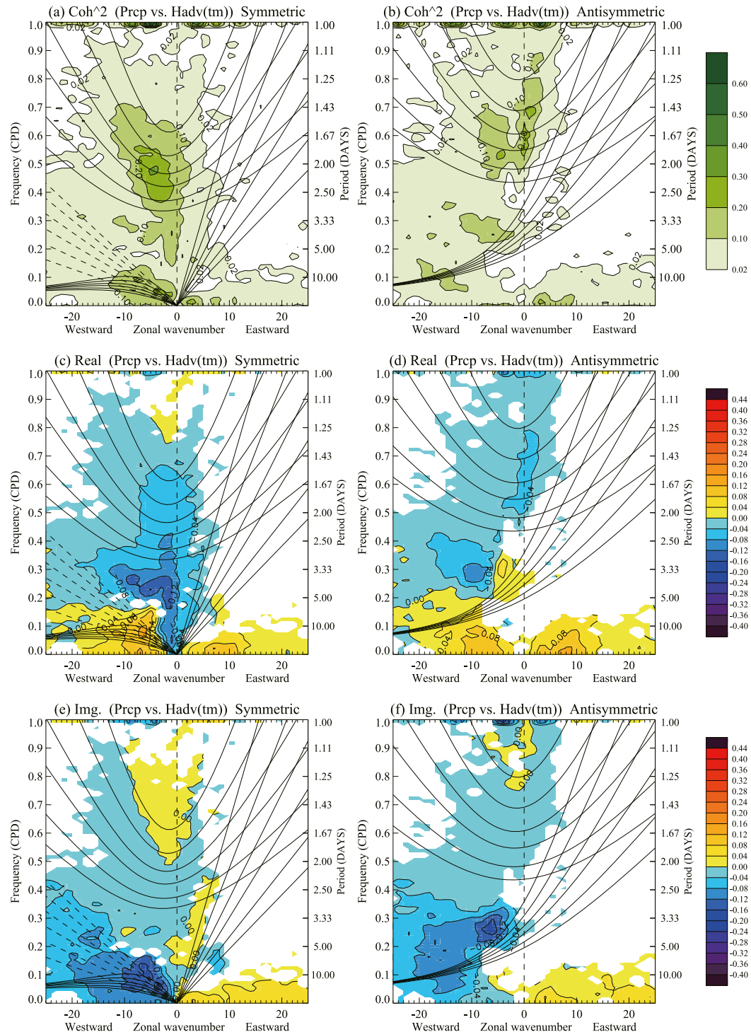
FIG. 8. As in Fig. 3, but for the results from cross-power spectrum between precipitation and column-integrated horizontal advection of time-mean MSE \overline{m}(\mathbf{x}, p) .
