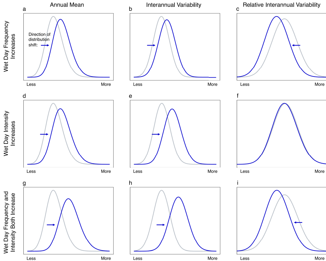
Figure 3. Responses of Annual Precipitation Totals and Interannual Variability of Precipitation to Changes in Wet Day Frequency and Intensity. (a) Initial probability distribution function (light gray) of annual precipitation totals based on Great Lakes domain precipitation intensity distribution. Projected probability distribution function (blue) after incorporating 10% increase in wet day frequency. (b) Same as (a) but for interannual variability of precipitation. (c) Same as (a) but for relative interannual variability of precipitation. (d–f) Same as (a–c) but projected probability distribution function incorporates a 10% increase in mean wet day intensity while the standard deviation of precipitation intensity distribution remains the same. (g–i) Same as (a–c) but projected distribution function incorporates a 10% increase in both wet day frequency and mean wet day intensity.
