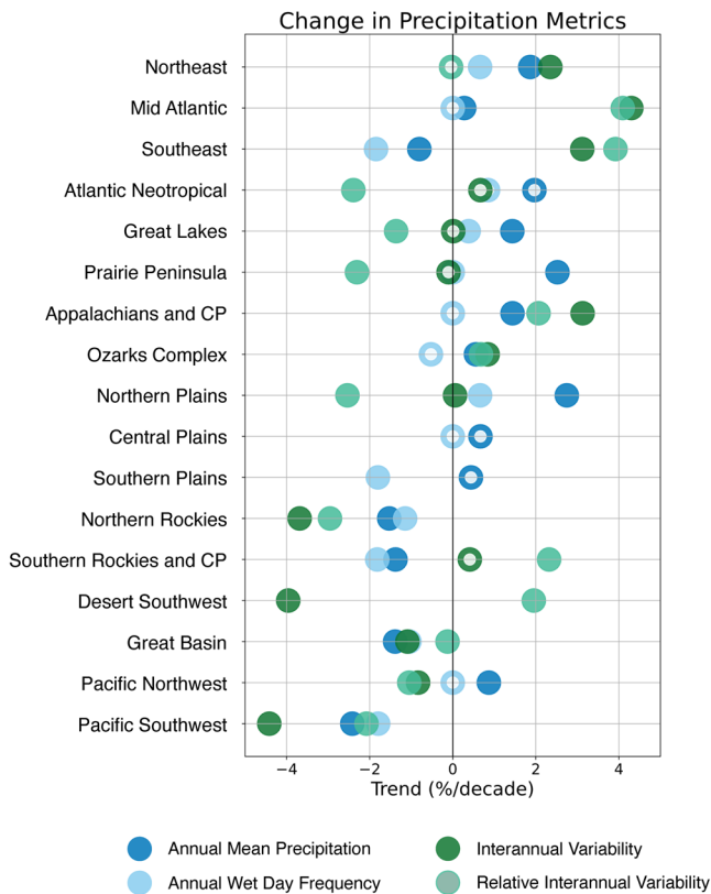
Figure 2. Domain Trends in Annual Precipitation Metrics. Trends in annual mean precipitation (dark blue), annual wet day frequency (light blue), interannual precipitation variability (dark green), and relative interannual precipitation variability (light green) for each domain. Trends are normalized against the mean value within each domain to produce trends in percent change/decade. Non-filled circles indicate non-significant domain-trends ( p > 0.05 ). Note that outlying trends in both metrics of interannual variability for the Central and Southern Plains, as well as annual mean precipitation and annual wet day frequency in the Desert Southwest, are not displayed.
