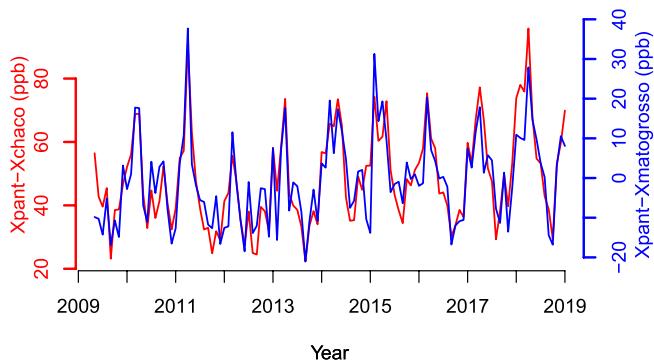
Figure 4. Difference of whole column CH 4 (ppb) at Pantanal and Mato Grosso (north-east of Pantanal, blue line), and Chaco (south-west of Pantanal, red line), respectively, retrieved from shortwave infrared radiances measured on the GOSAT satellite mission.
