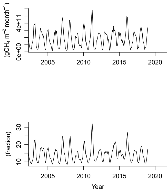
Figure 5. Pantanal average CH 4 flux (upper panel) and fraction of flooded area (lower panel) estimated by LPJ-wsl wetlands model (Zhang et al., 2016).
