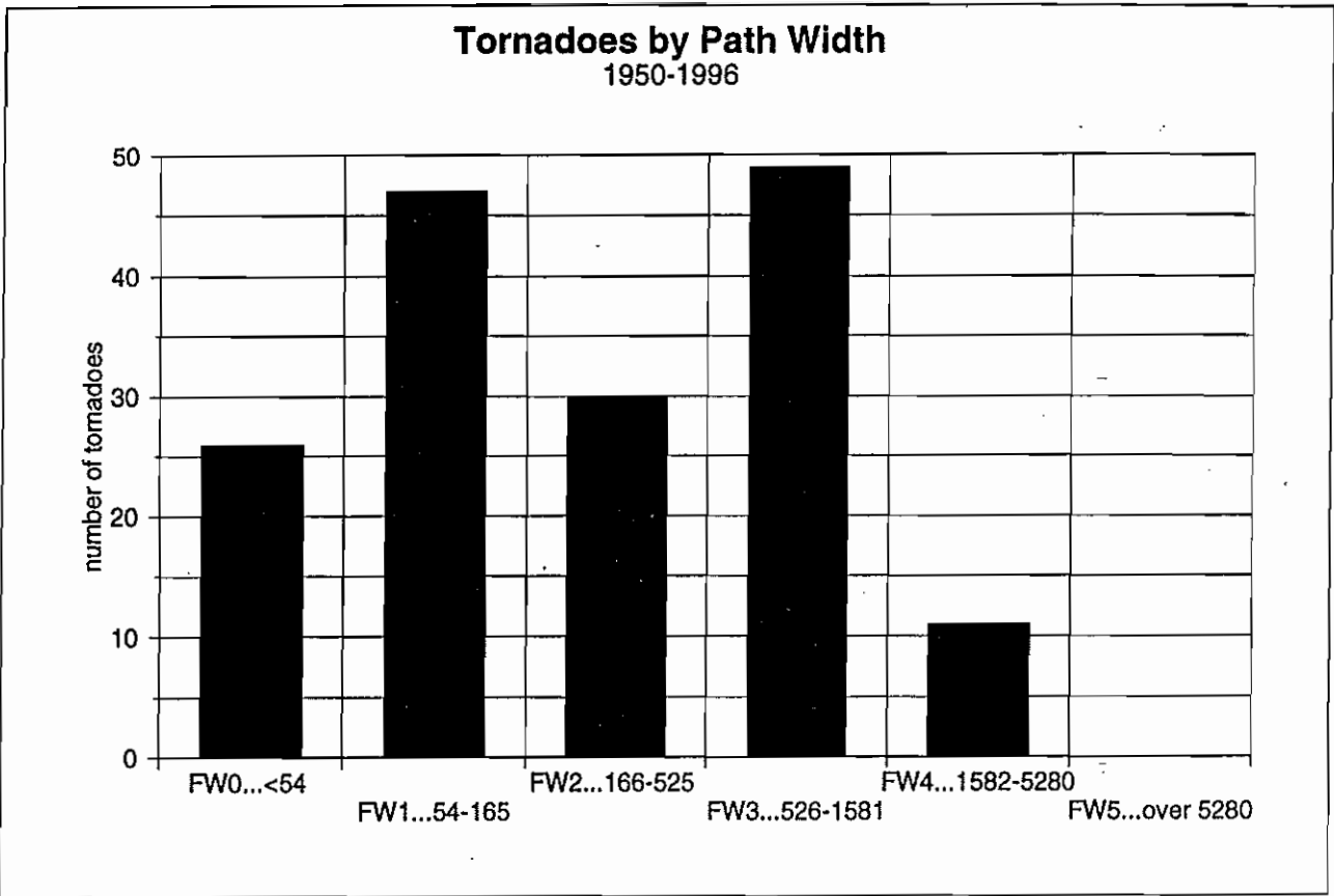
Figure 10. Number of tornadoes by path width (ft.).
