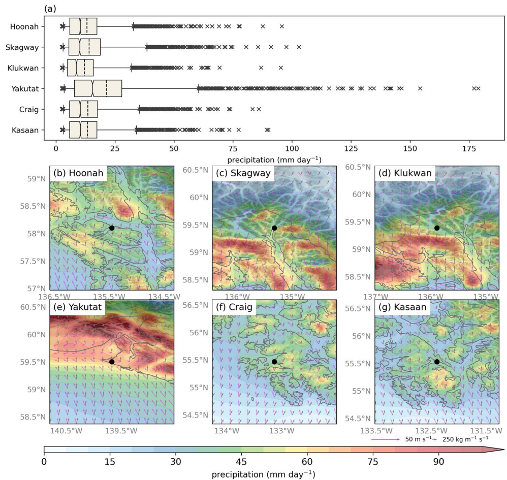
Figure 6. (a) Distribution of daily WRF precipitation for all AR days between 1 January 1980 and 31 December 2019 when precipitation was >2.5 \text{ mm day}^{-1} for each community (note that the sample size of AR days for each community ranges from 3,155 to 3,618). The box extends from lower to upper quartiles of the data, with a black solid line at the median and a black dotted line at the mean. The whiskers show the range of the data from the fifth percentile to the 95th percentile. (b) Average daily composites of WRF precipitation (shaded, \text{mm day}^{-1} ), ERA5 IVT (gray vectors, \text{kg m}^{-1} \text{ s}^{-1} ), and WRF 1000 hPa winds (pink vectors, \text{m s}^{-1} ) for Hoonah during extreme AR days. The location of Hoonah is shown by the black point. USGS GMT elevation data (gray shaded, m) is shown where higher elevations are darker shades (c)–(h) Same as (b) but for (c) Skagway, (d) Klukwan, (e) Yakutat, (f) Craig and (g) Kasaan.
